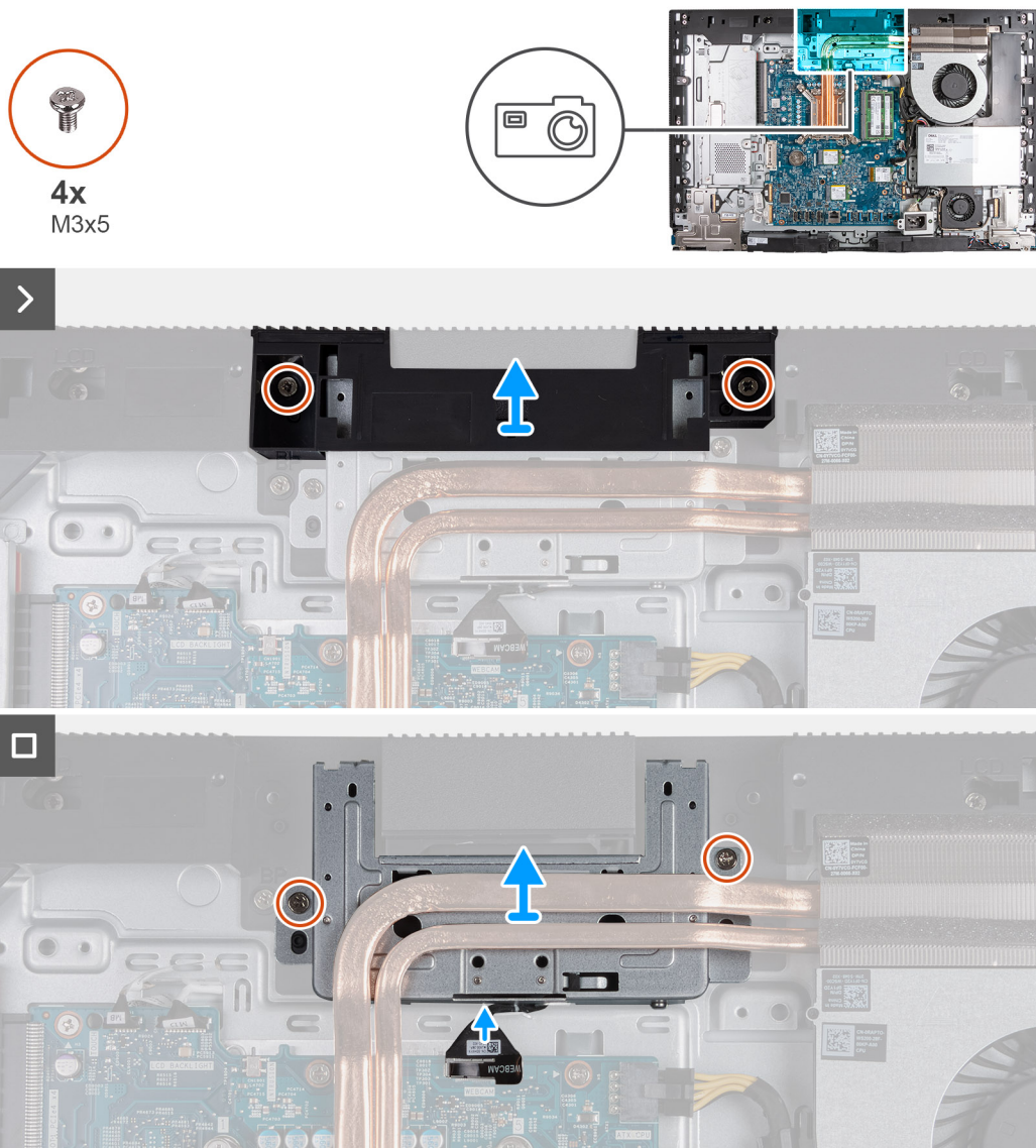
Figure 45. Removing the retractable-camera assembly
