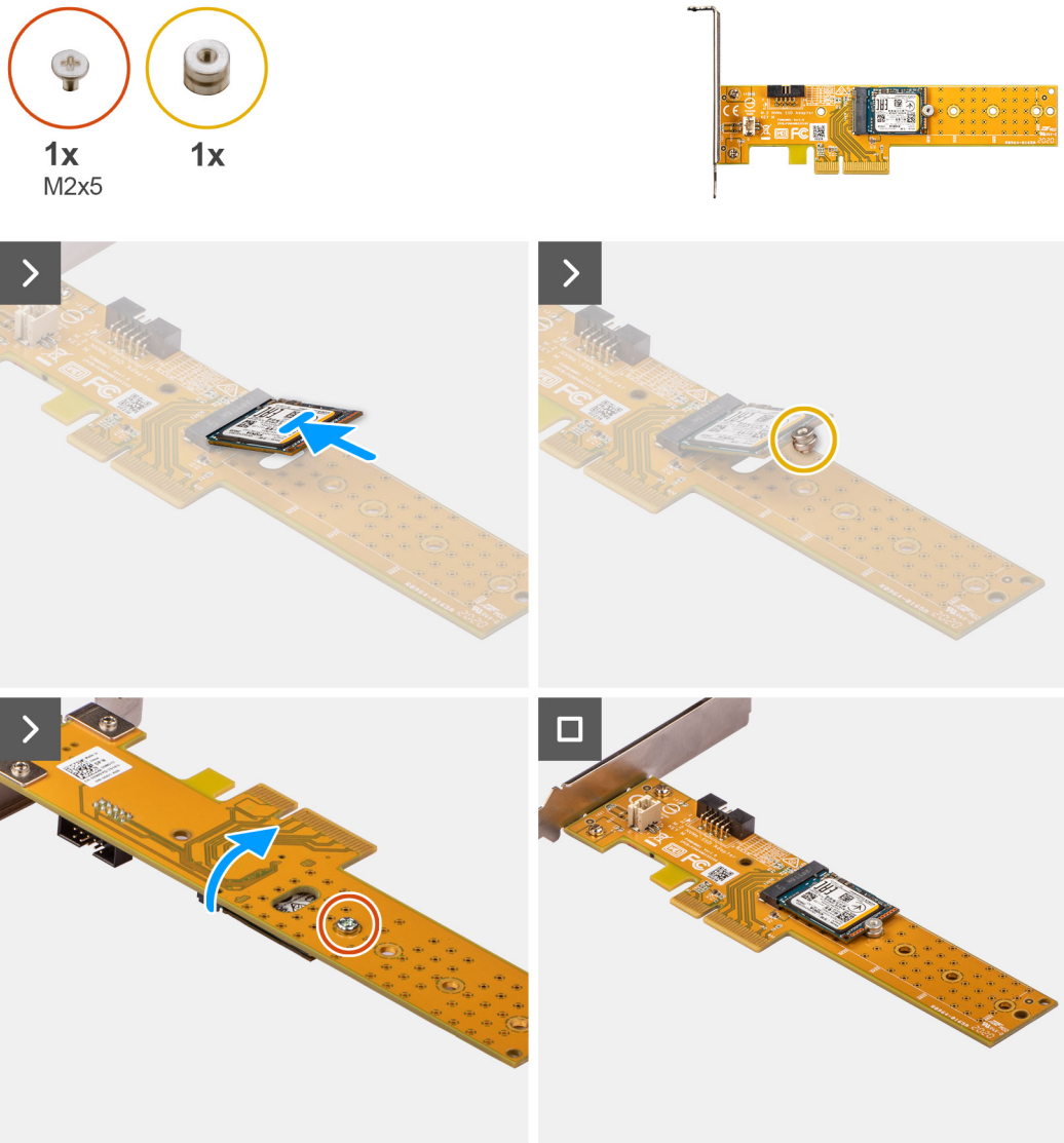
Figure 26. Installing the M.2 2230 solid-state drive on Dell Ultra Speed Drive Gen3 card
