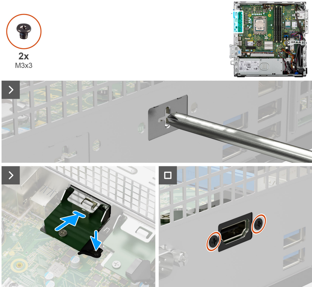
Figure 59. Installing the HDMI module
