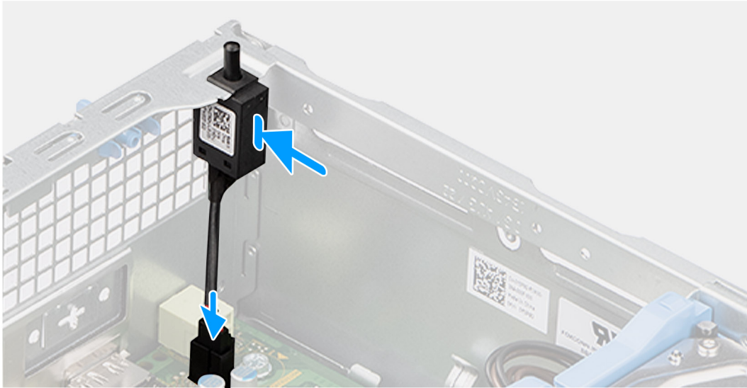
Figure 38. Installing the Intrusion switch
