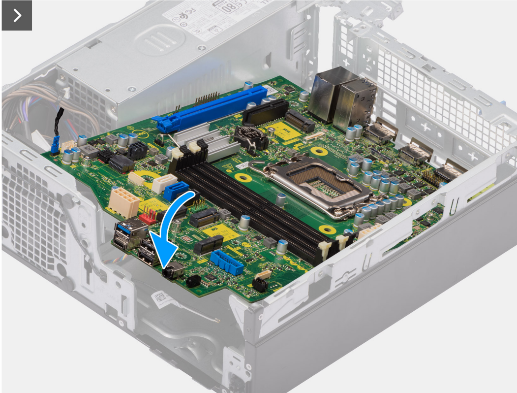
Figure 70. Installing the system board
