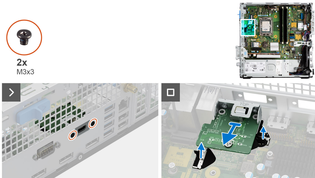
Figure 62. Removing the Type-C module
