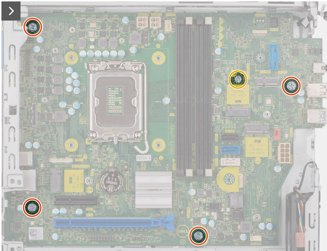
Figure 67. Removing the system board
