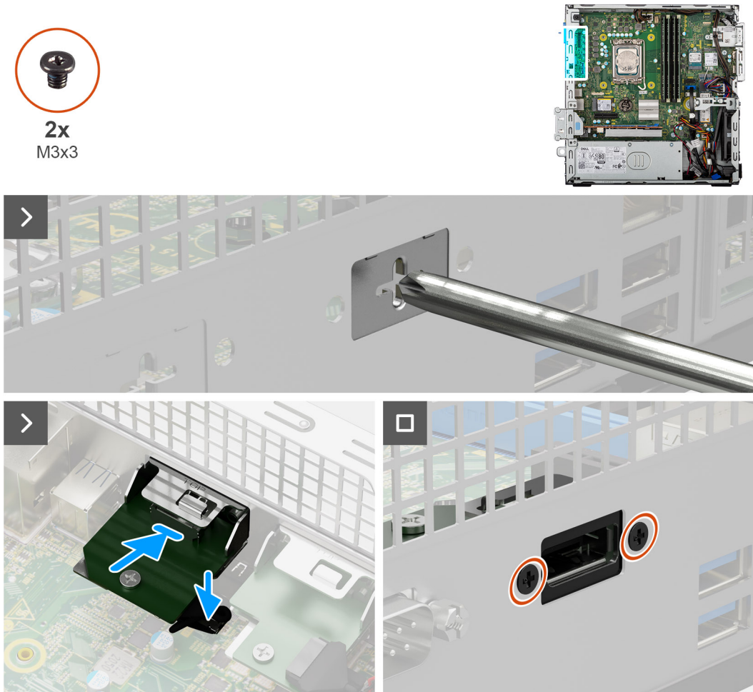
Figure 57. Installing the DisplayPort module
