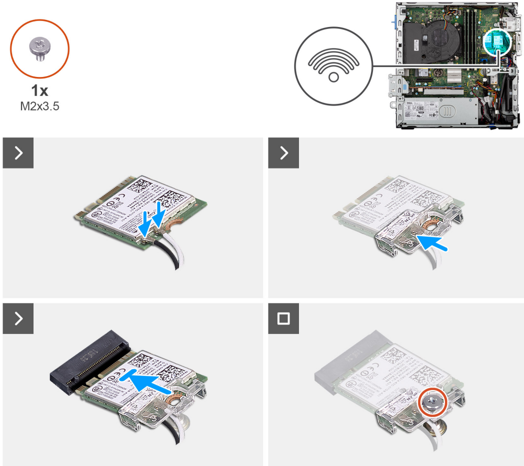
Figure 30. Installing the wireless card
