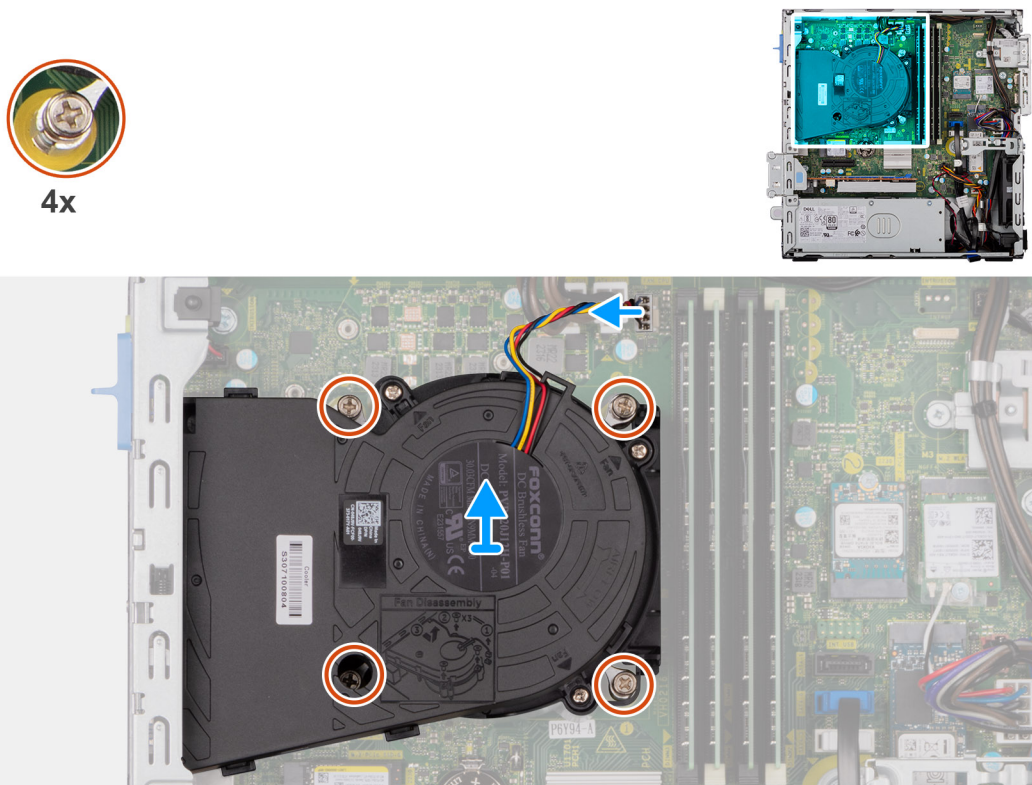
Figure 50. Removing the processor-fan and heat-sink assembly
