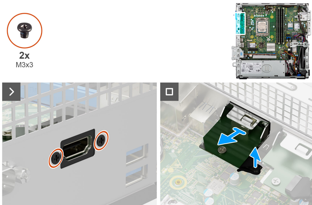
Figure 58. Removing the HDMI module
