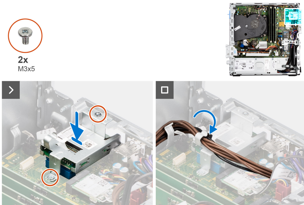
Figure 32. Installing the media-card reader
