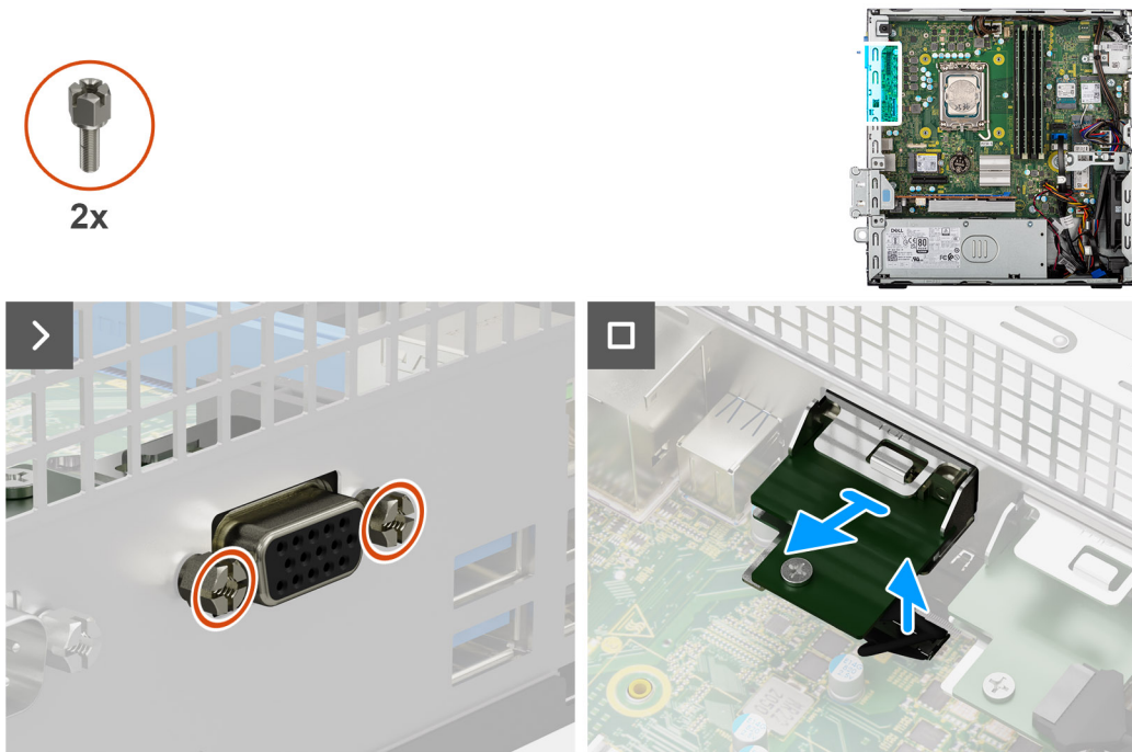
Figure 60. Removing the VGA module
