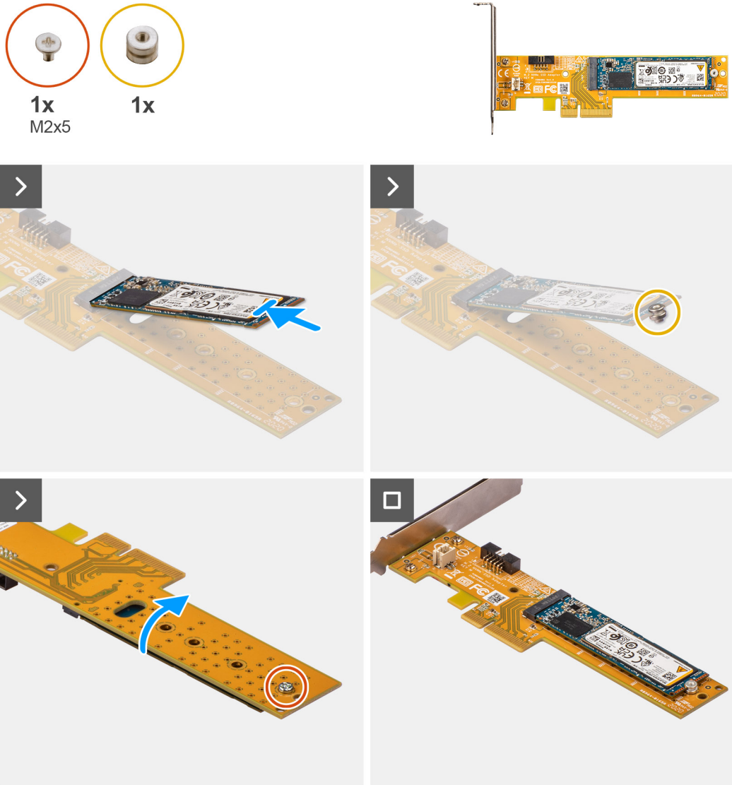
Figure 27. Installing the M.2 2280 solid-state drive on Dell Ultra Speed Drive Gen3 card
