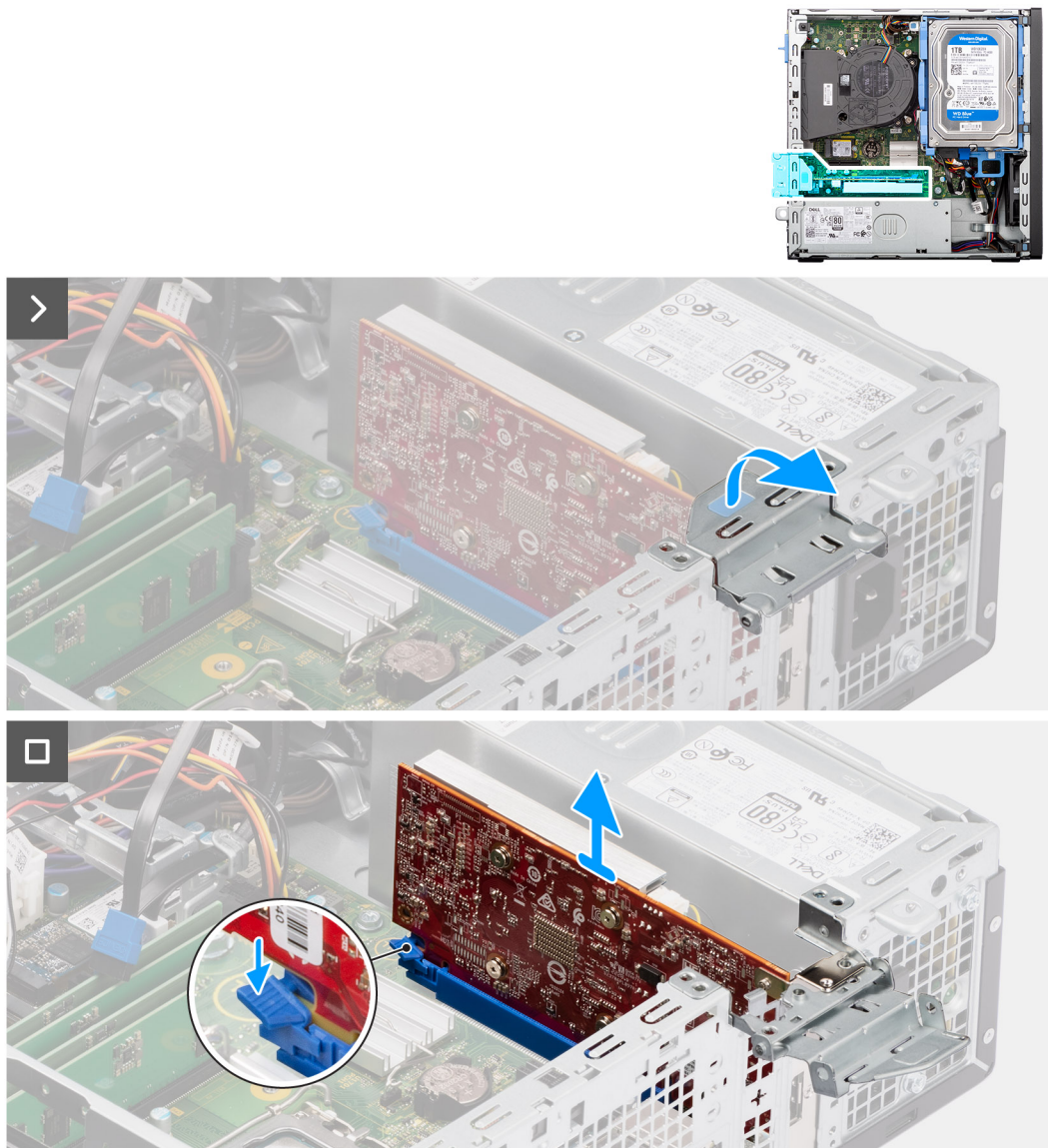
Figure 33. Removing the graphics card
