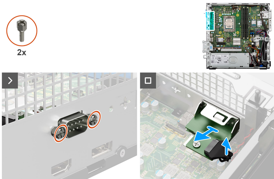
Figure 54. Removing the serial module
