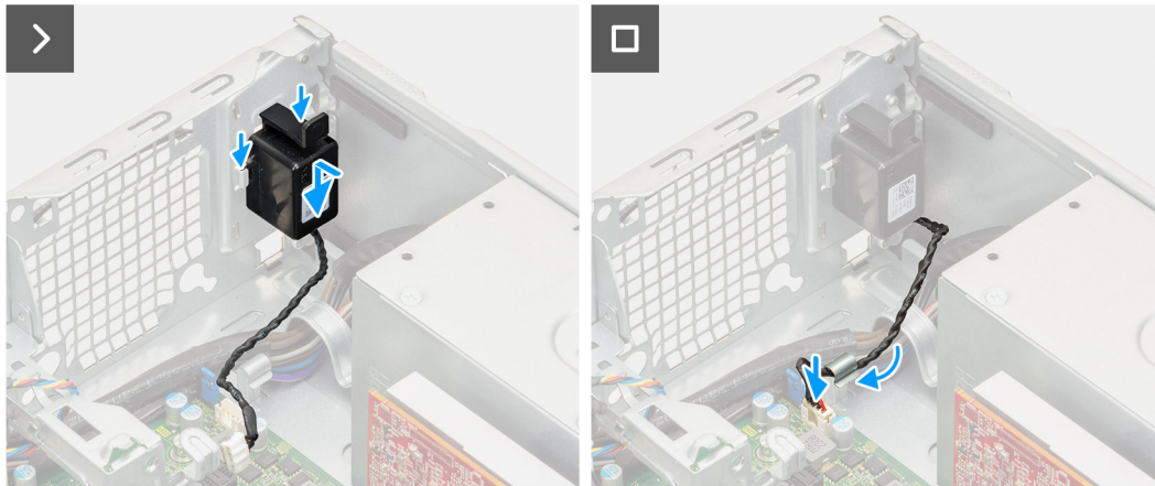
Figure 36. Installing the speaker
