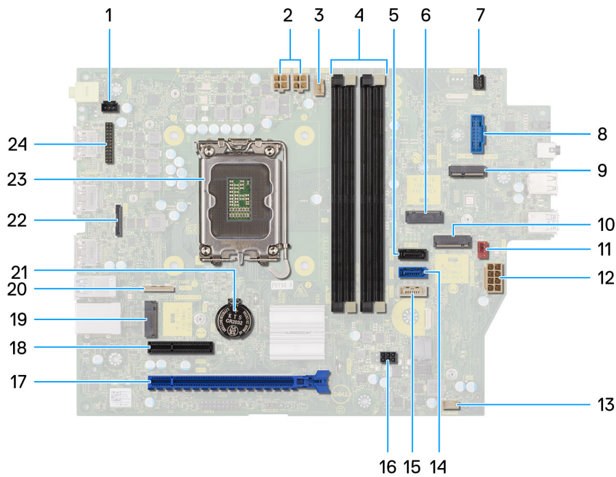
Figure 69. System board overview
