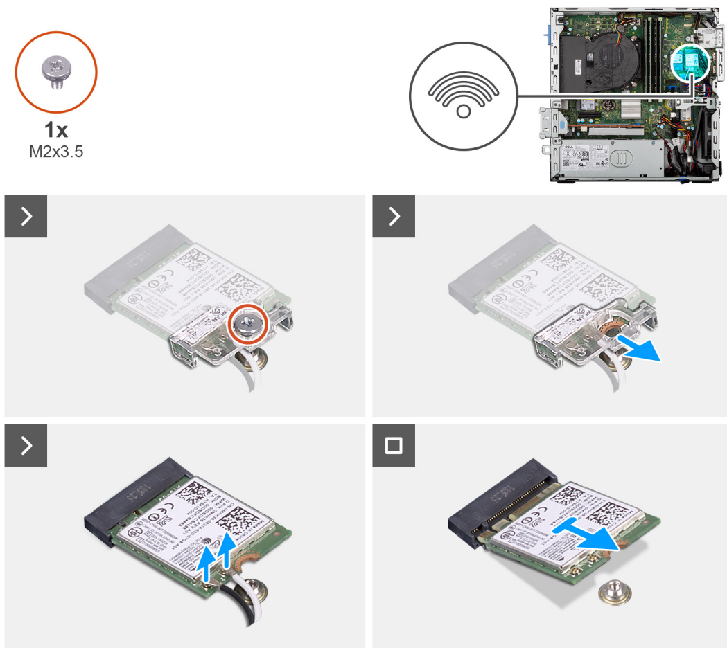
Figure 29. Removing the wireless card
