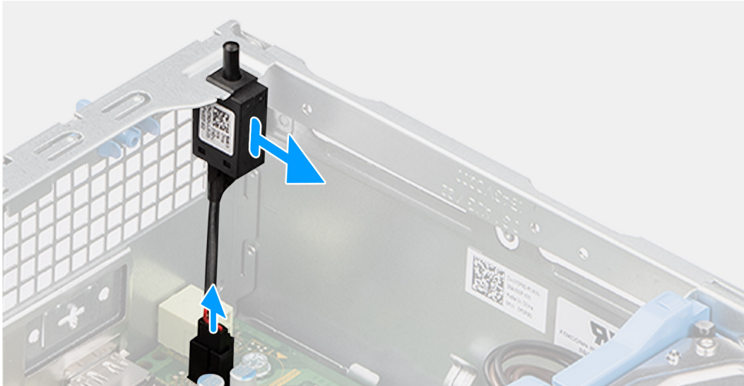
Figure 37. Removing the intrusion switch
