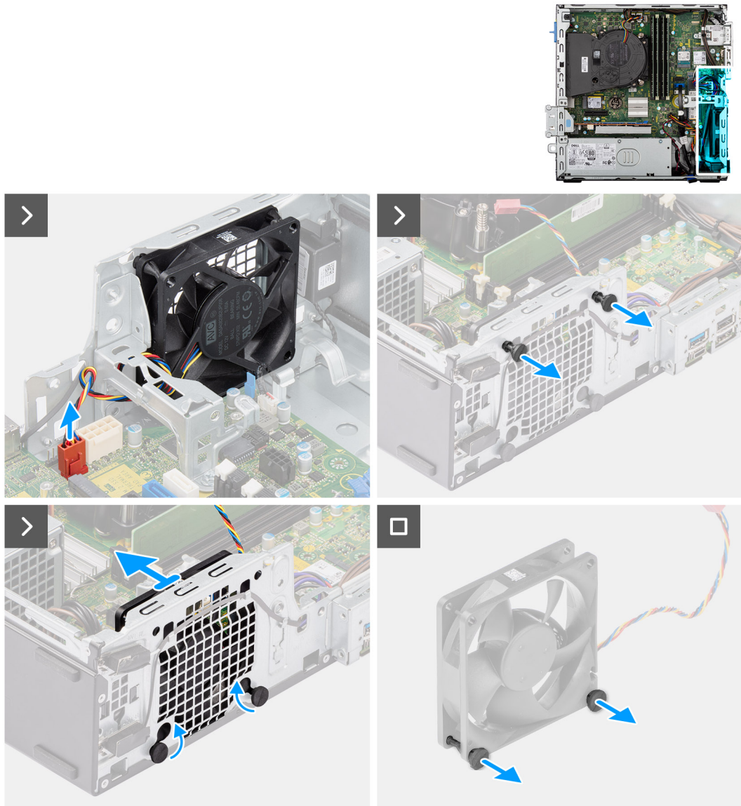
Figure 41. Removing the system fan
