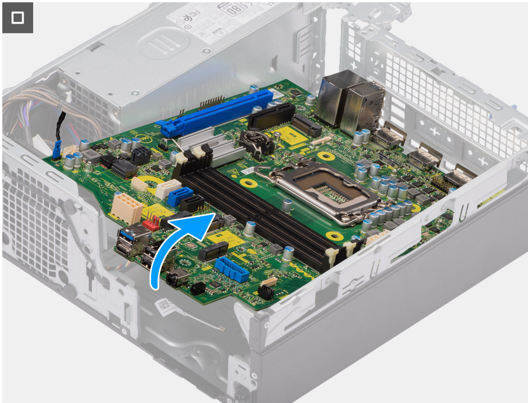
Figure 68. Removing the system board
