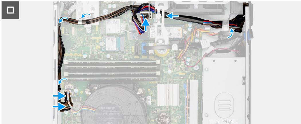
Figure 49. Installing the power-supply unit
