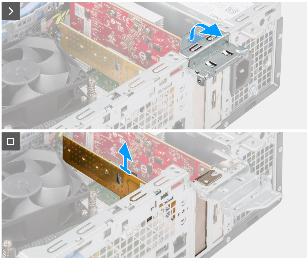
Figure 23. Removing Dell Ultra Speed Drive Gen3 card
