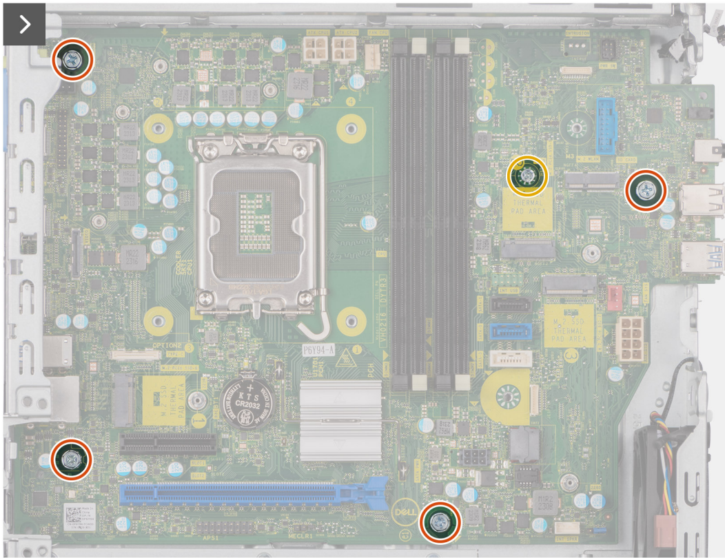
Figure 71. Installing the system board
