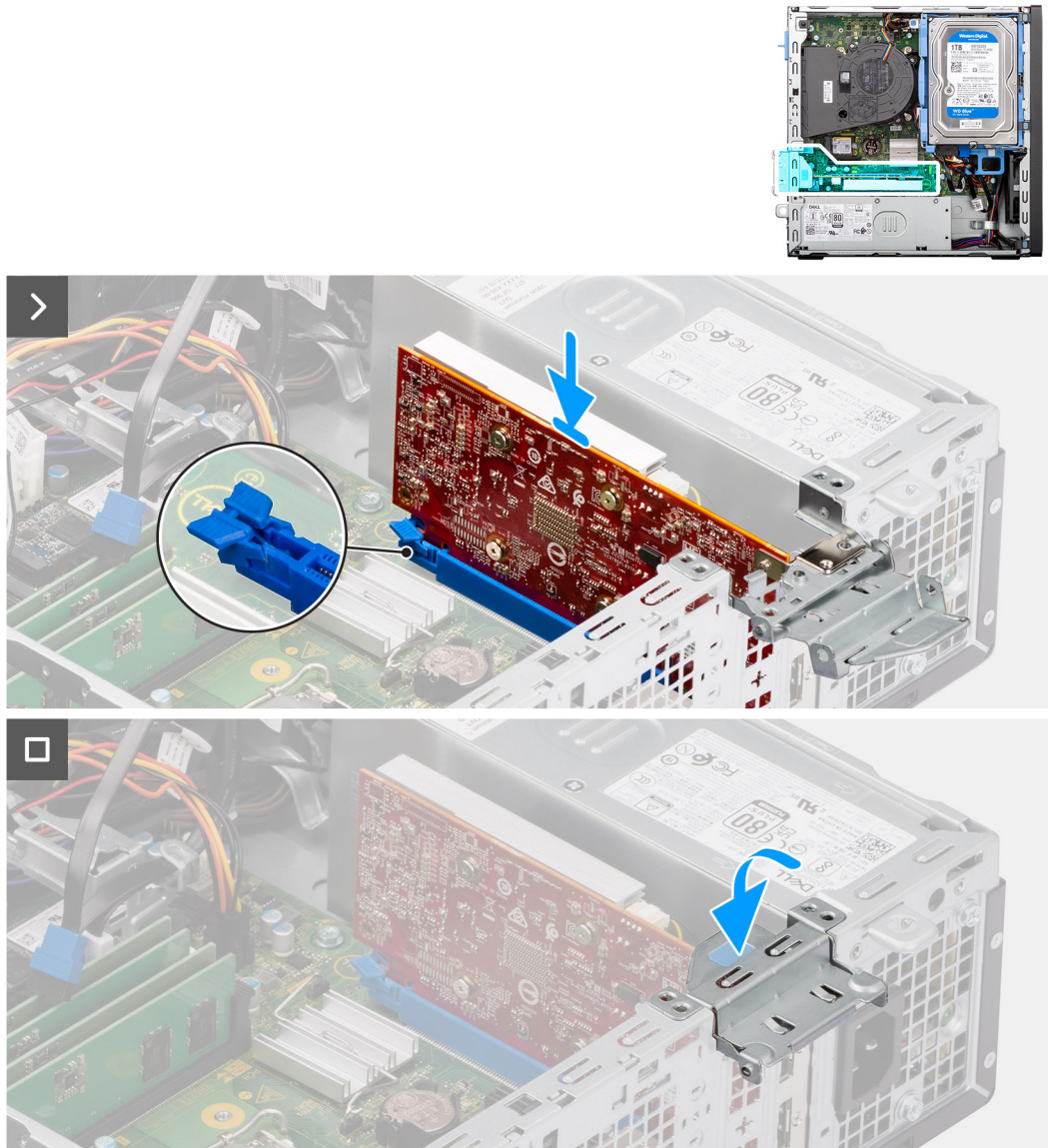
Figure 34. Installing the graphics card
