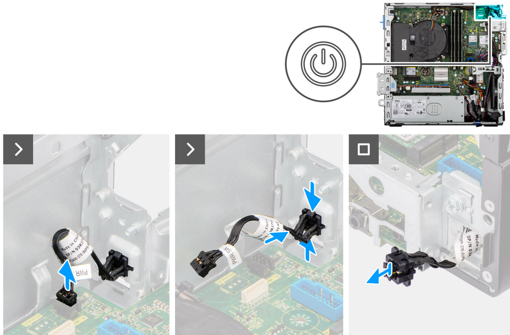
Figure 39. Removing the power button
