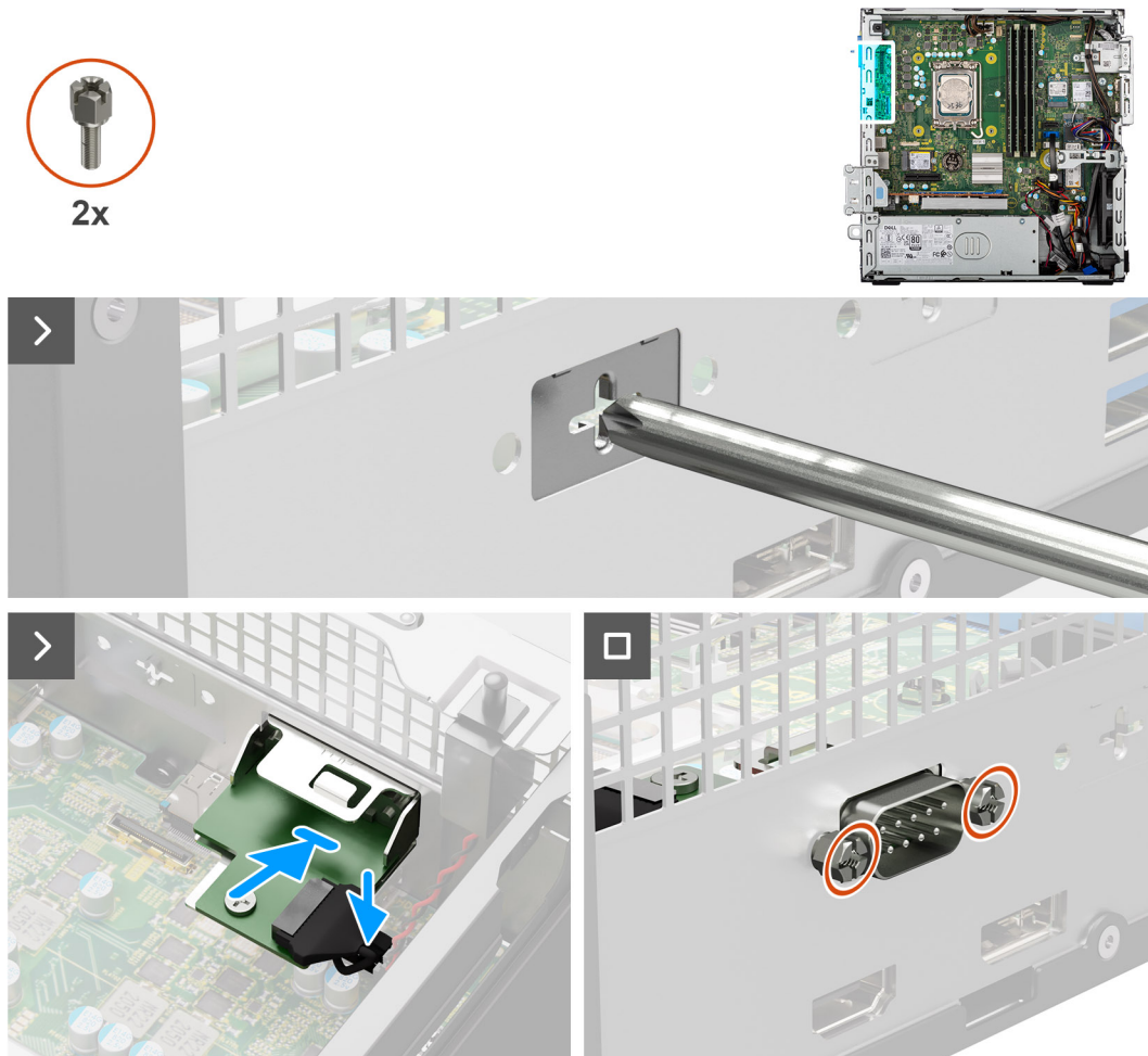
Figure 55. Installing the serial module
