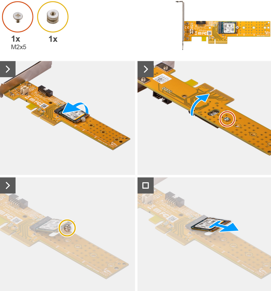
Figure 24. Removing M.2 2230 solid-state drive from Dell Ultra Speed Drive Gen3 card
