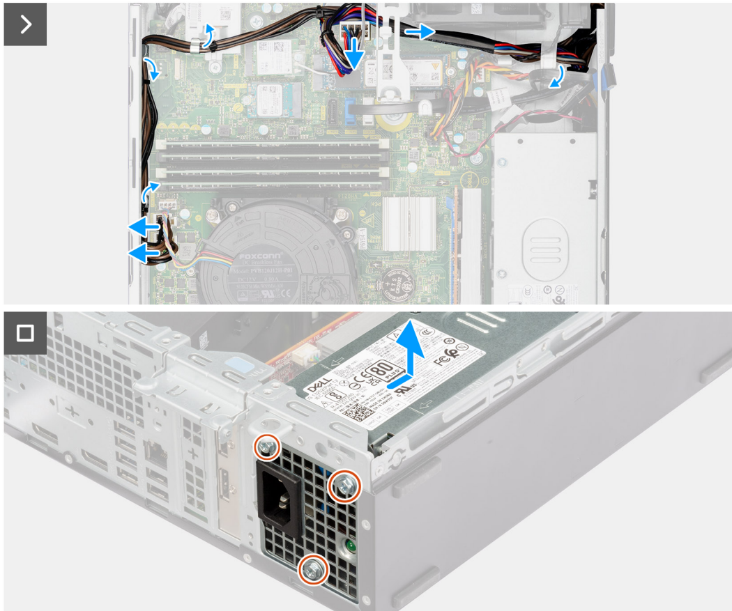
Figure 48. Removing the power-supply unit
