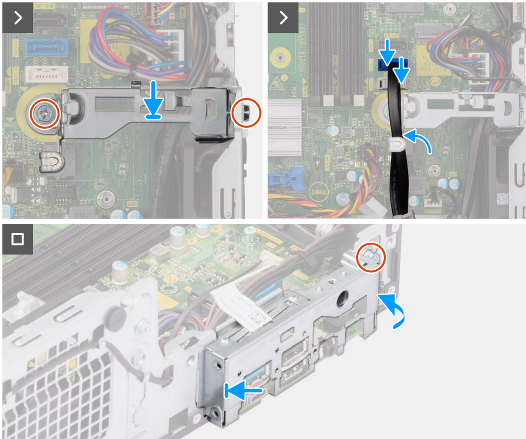
Figure 73. Installing the system board
