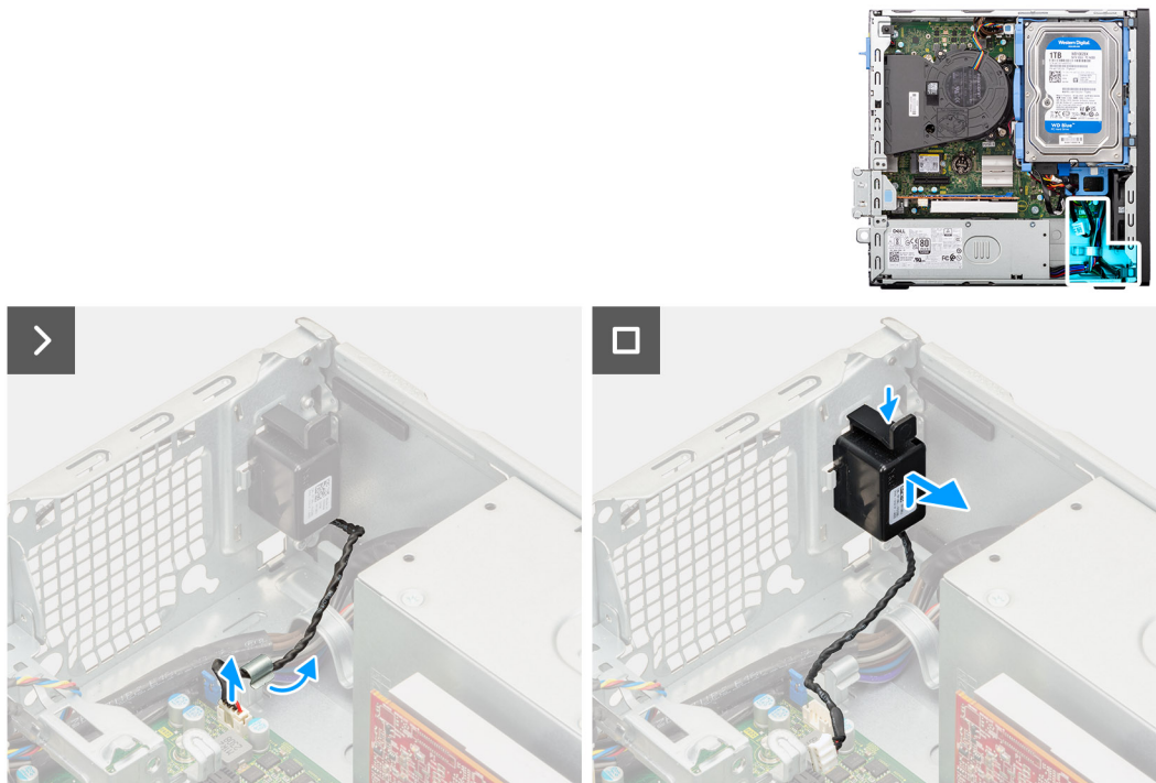
Figure 35. Removing the speaker
