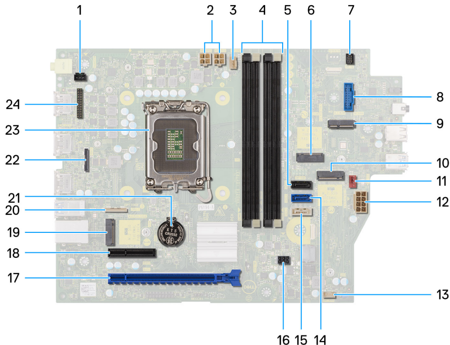
Figure 64. System board overview
