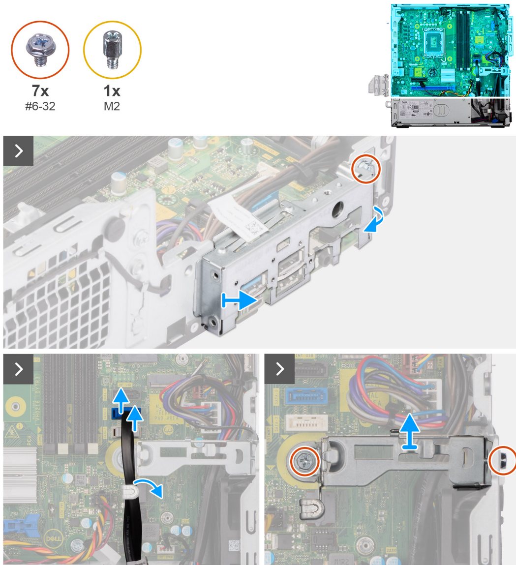
Figure 65. Removing the system board
