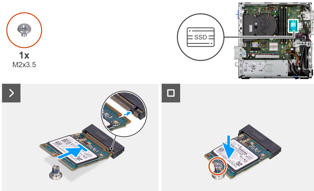
Figure 20. Installing the M.2 2230 solid-state drives in slot 1
