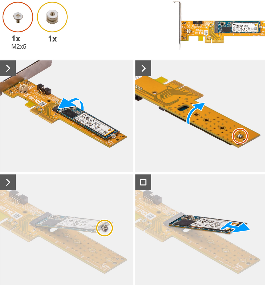
Figure 25. Removing M.2 2280 solid-state drive from Dell Ultra Speed Drive Gen3 card
