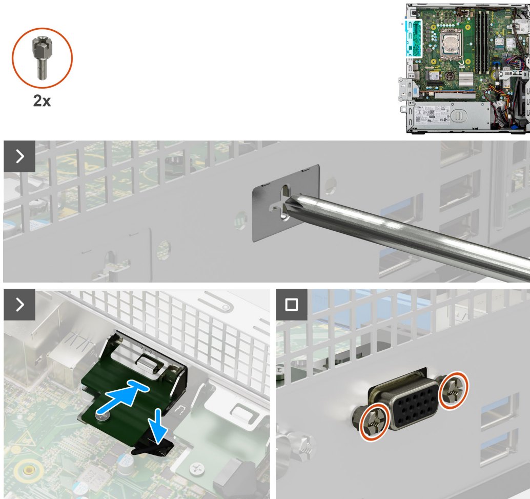
Figure 61. Installing the VGA module
