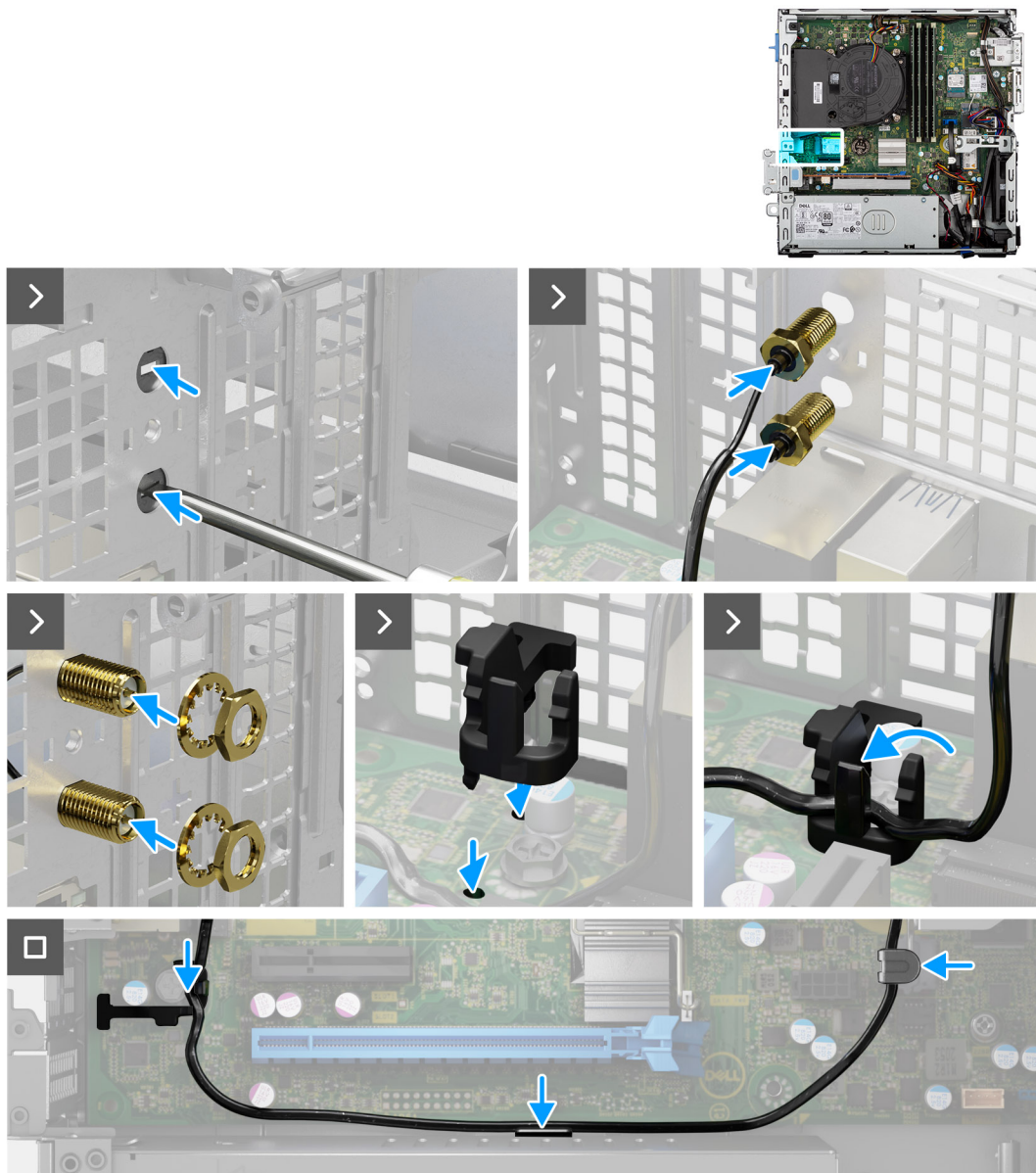
Figure 47. Installing the external SMA antenna module
