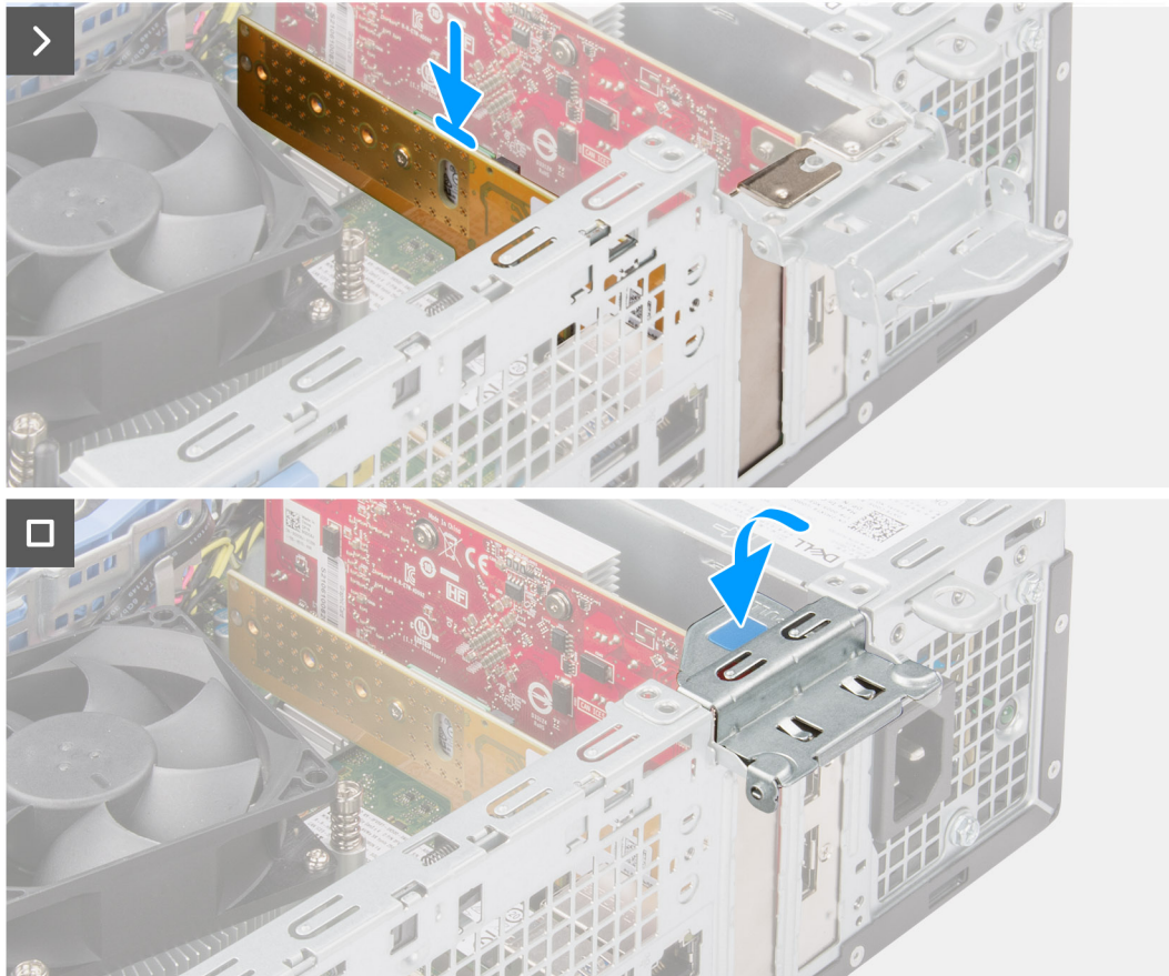
Figure 28. Installing the Dell Ultra Speed Drive Gen3 card
