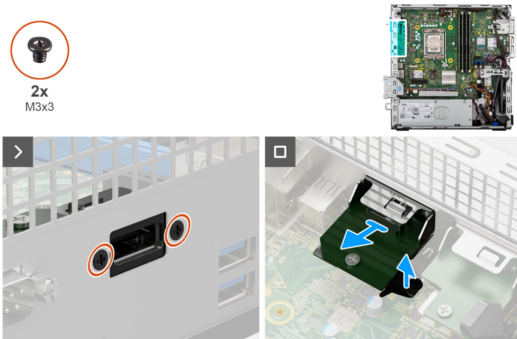
Figure 56. Removing the DisplayPort module
