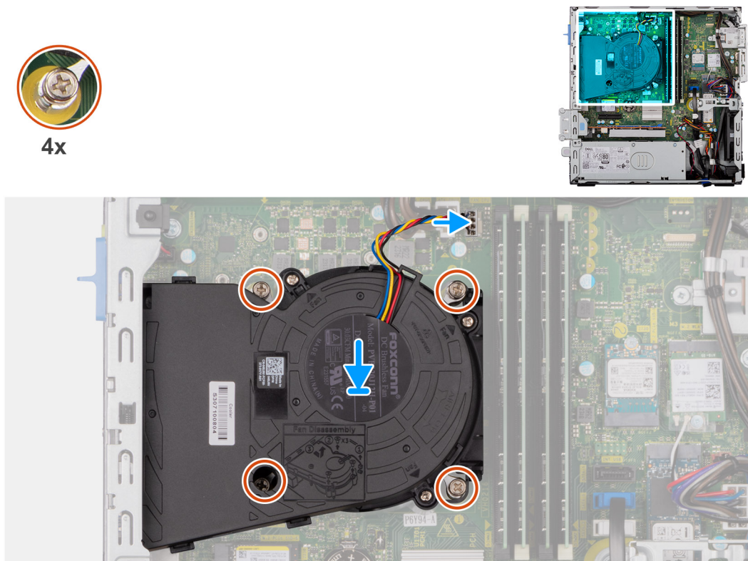
Figure 51. Installing the processor fan and heat-sink assembly
