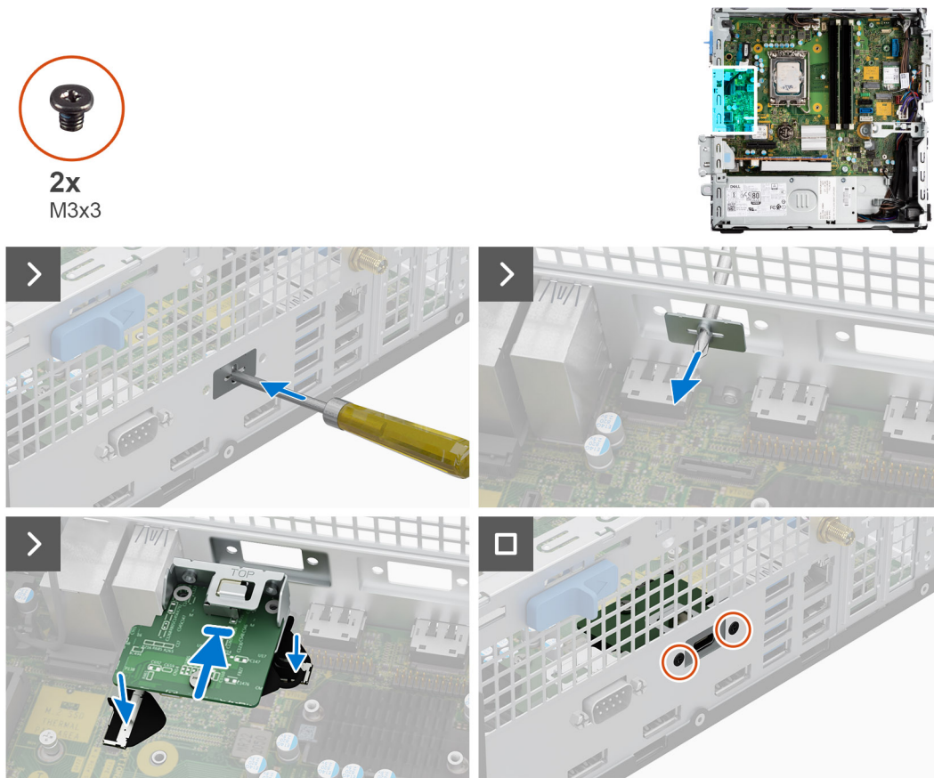
Figure 63. Installing the Type-C module
