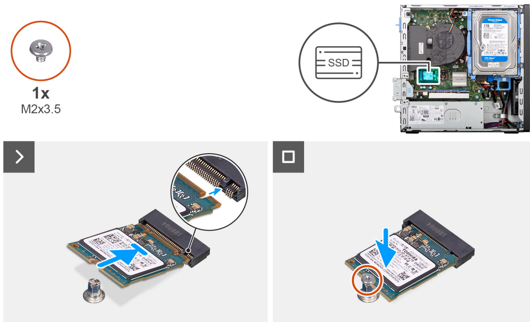
Figure 18. Installing the M.2 2230 solid-state drive in slot 0
