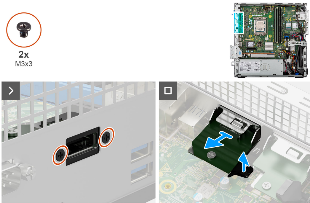
Figure 56. Removing the DisplayPort module
