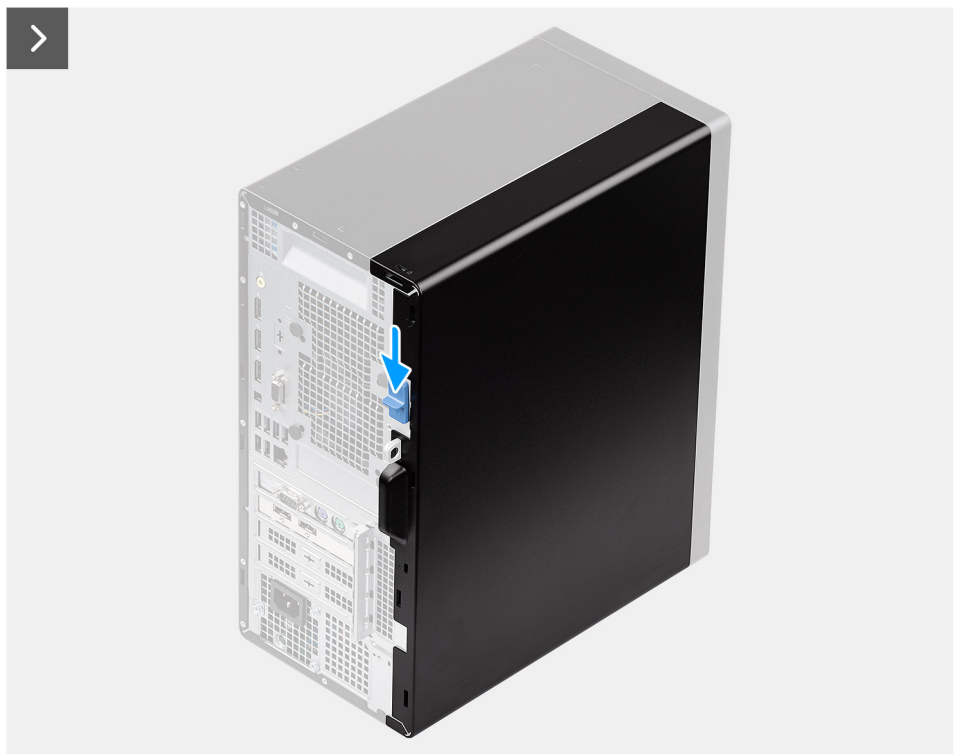
Figure 9. Removing the side cover
