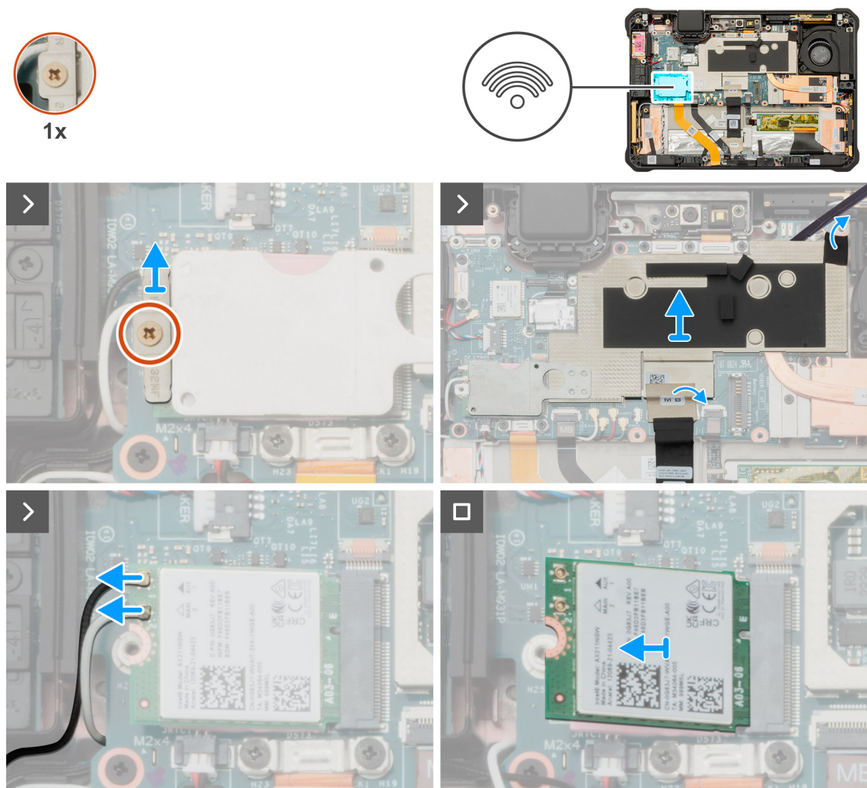
Figure 61. Removing the wireless card
