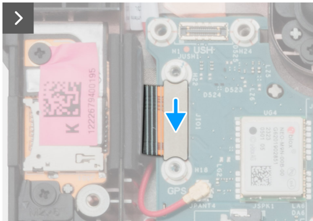
Figure 60. Installing the I/O daughter-board
