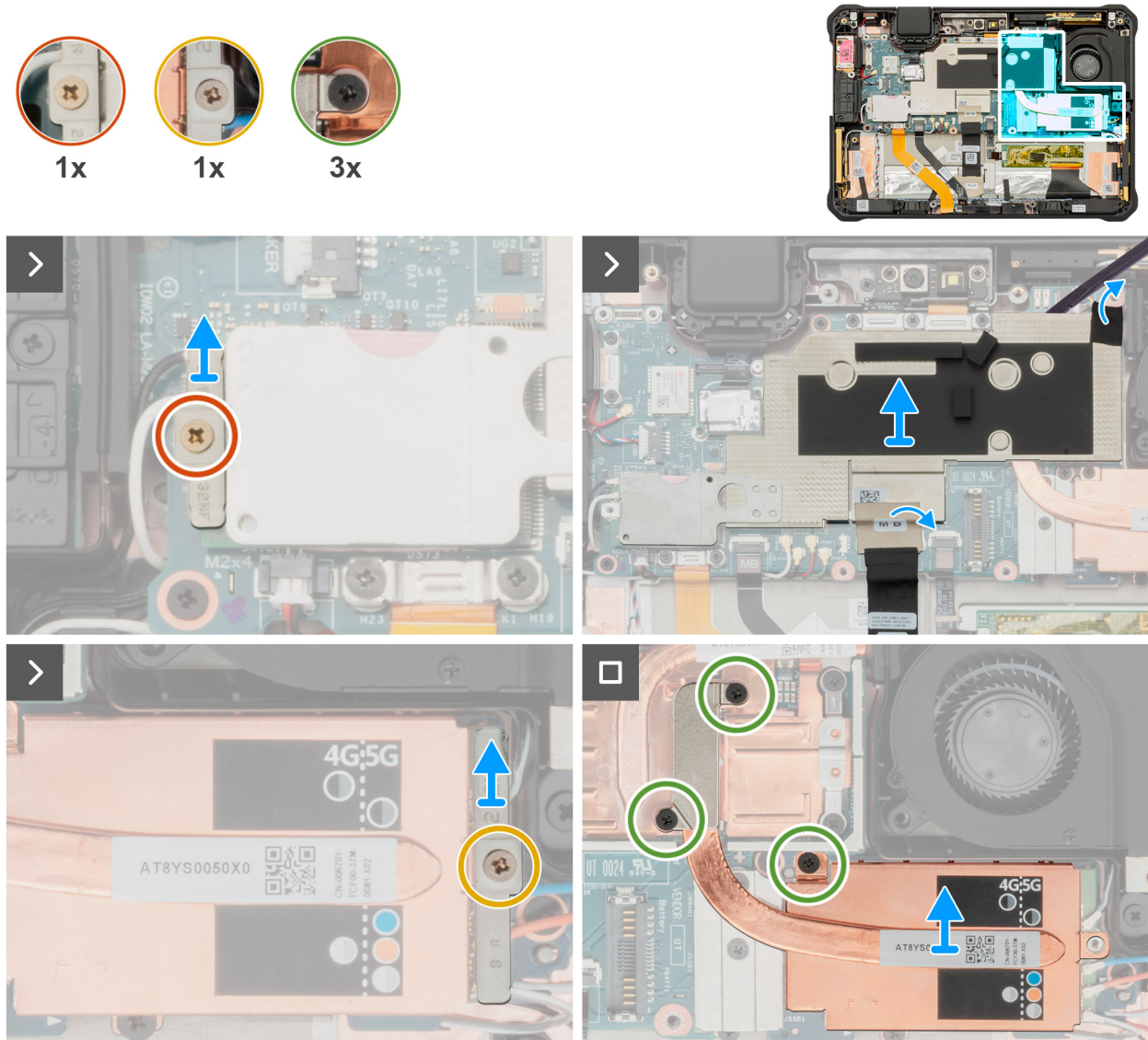
Figure 79. Removing the WWAN-card heat-sink
