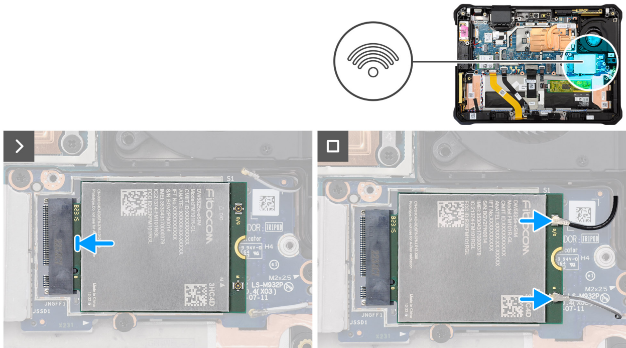
Figure 88. Installing the 4G WWAN card
