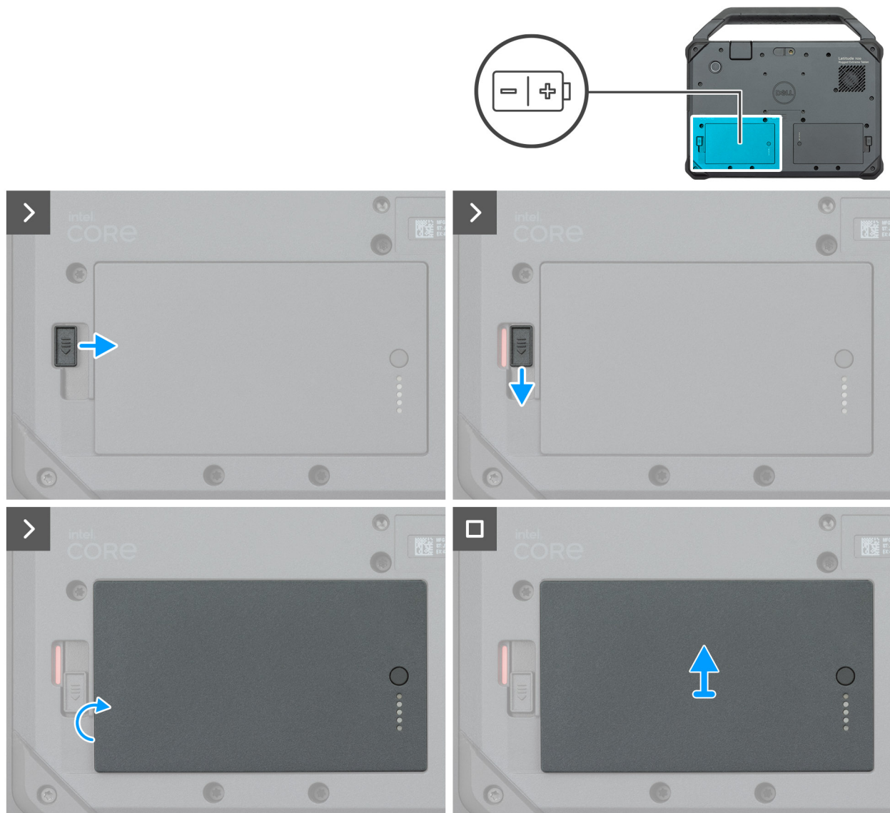
Figure 43. Removing the hot-swappable batteries
