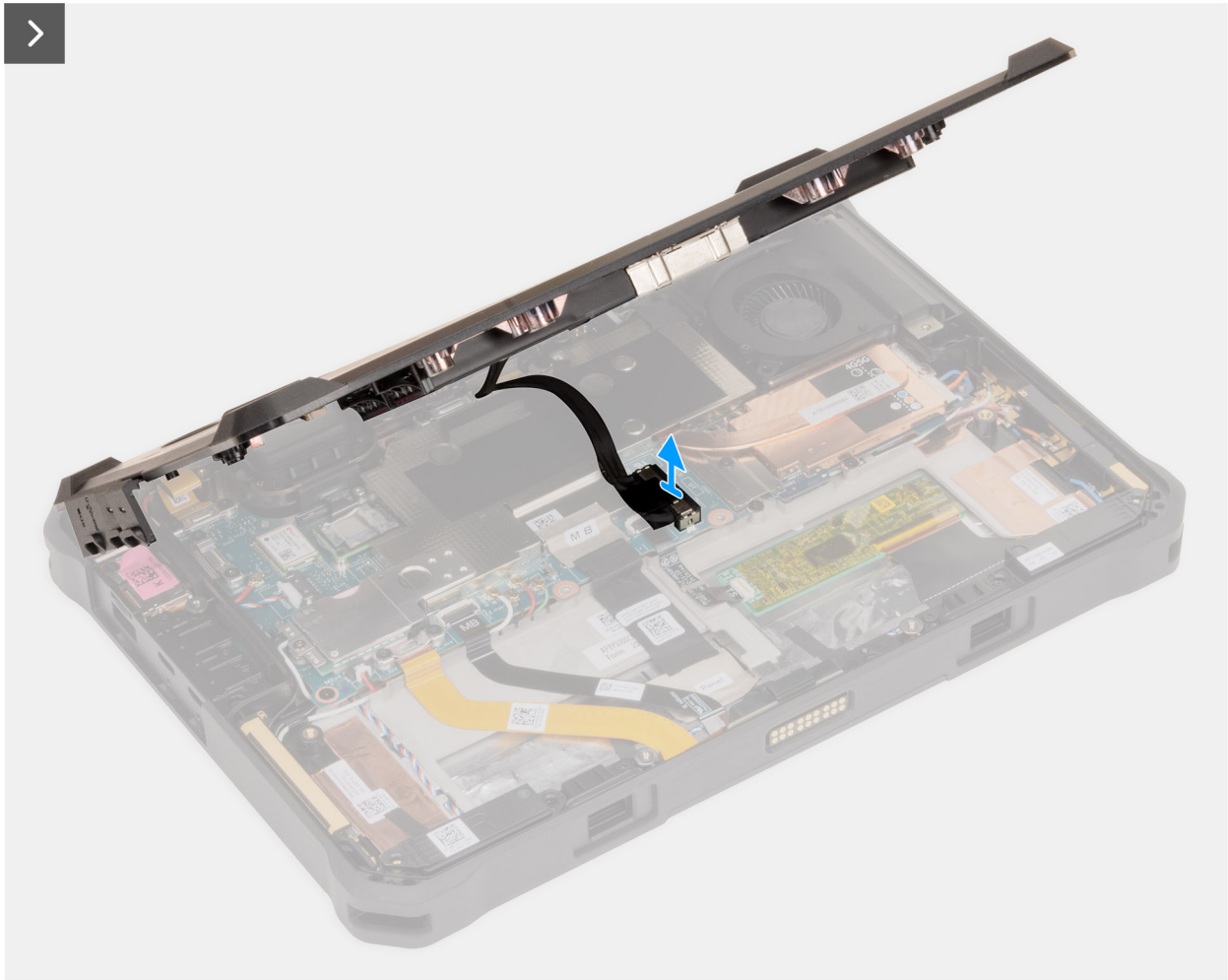
Figure 49. Removing the base-cover assembly
