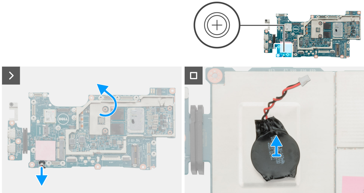
Figure 106. Removing the coin-cell battery
