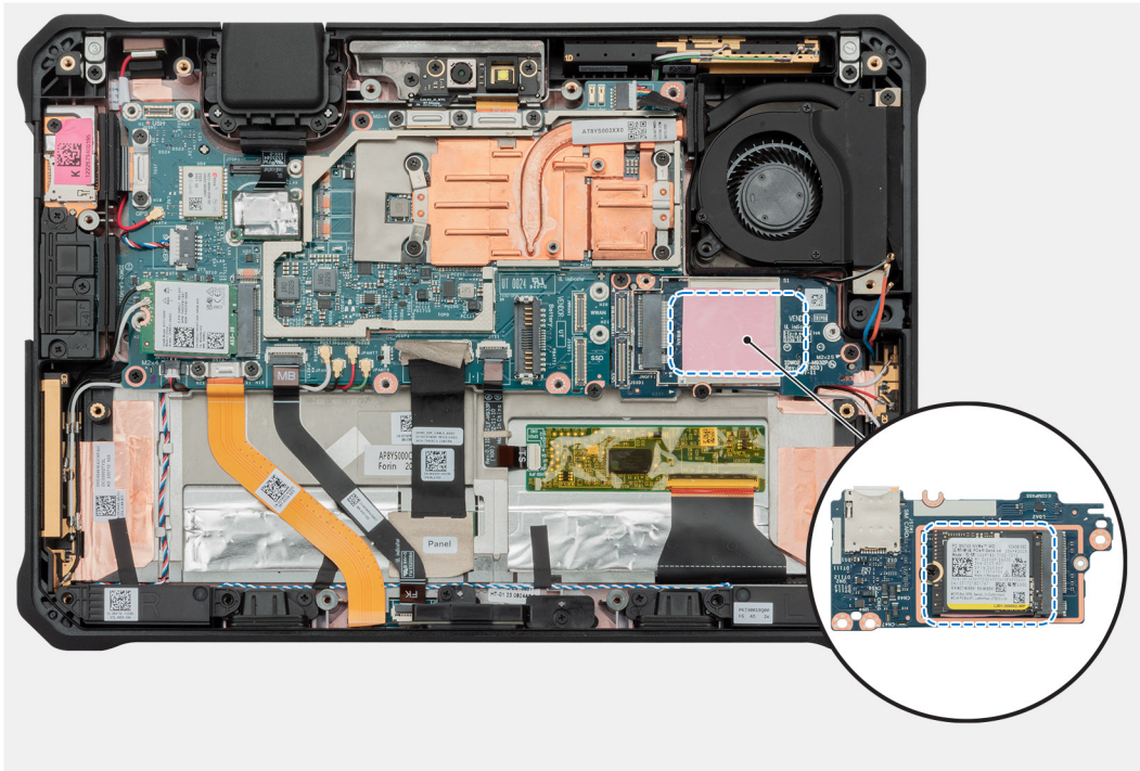
Figure 91. Removing the WWAN/SSD daughter-board
