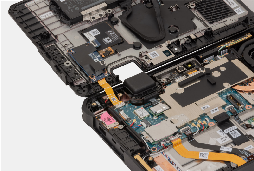
Figure 51. Removing the base-cover assembly
