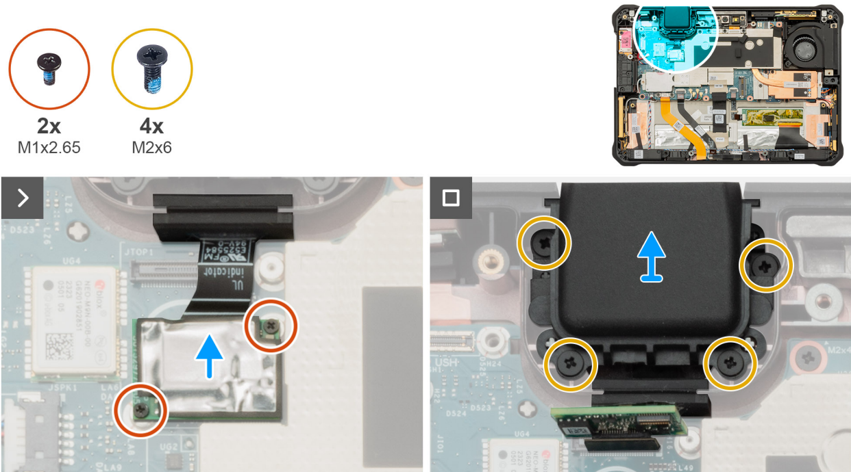
Figure 77. Removing the 1D-2D barcode-scanner assembly
