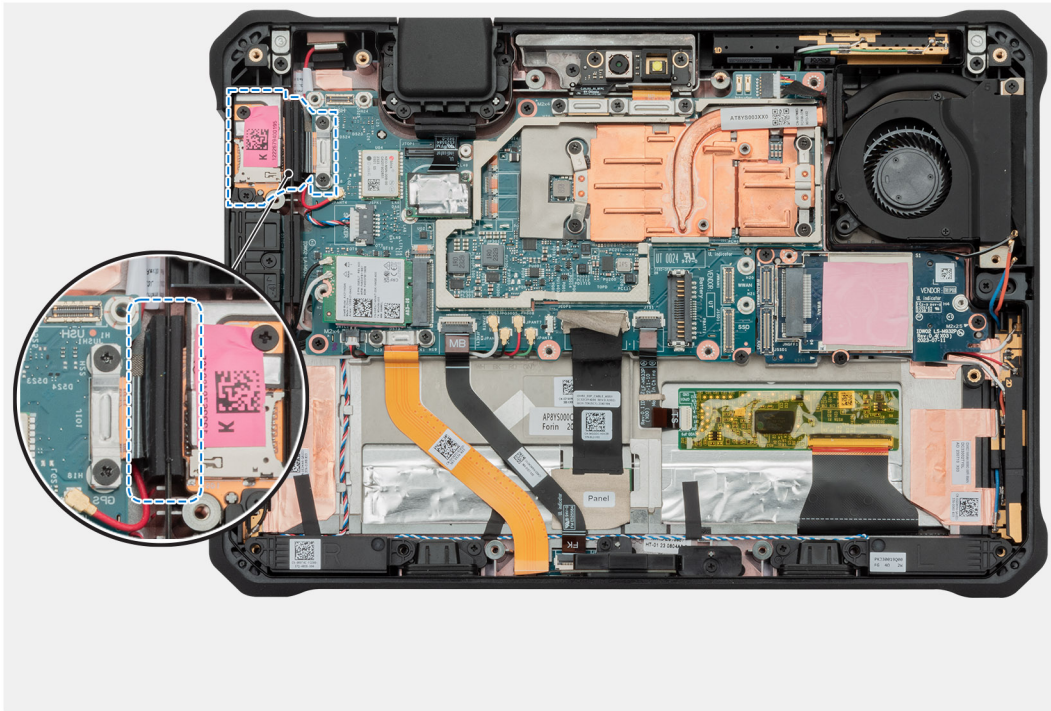
Figure 59. Removing the I/O daughter-board
