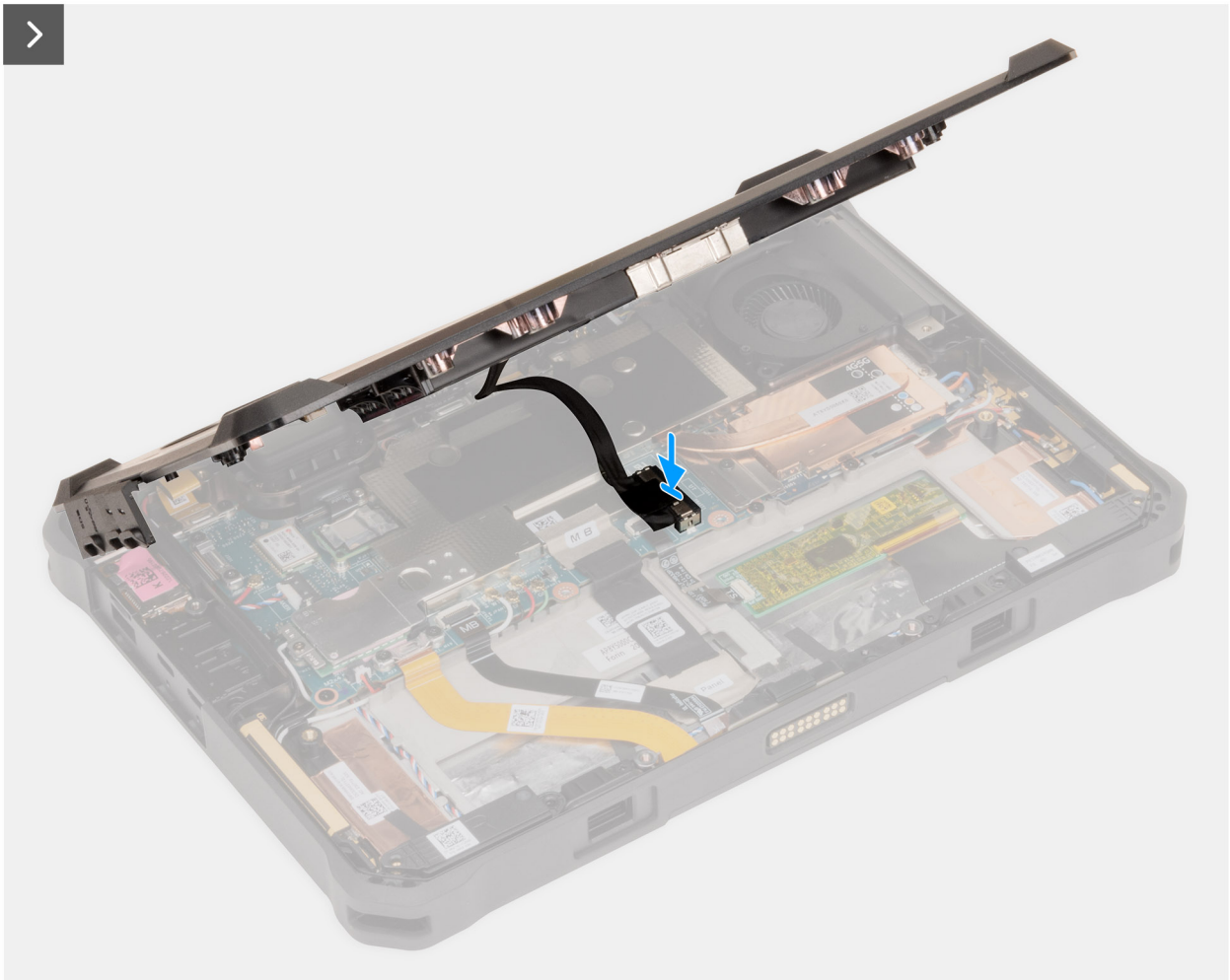
Figure 53. Installing the base-cover assembly
