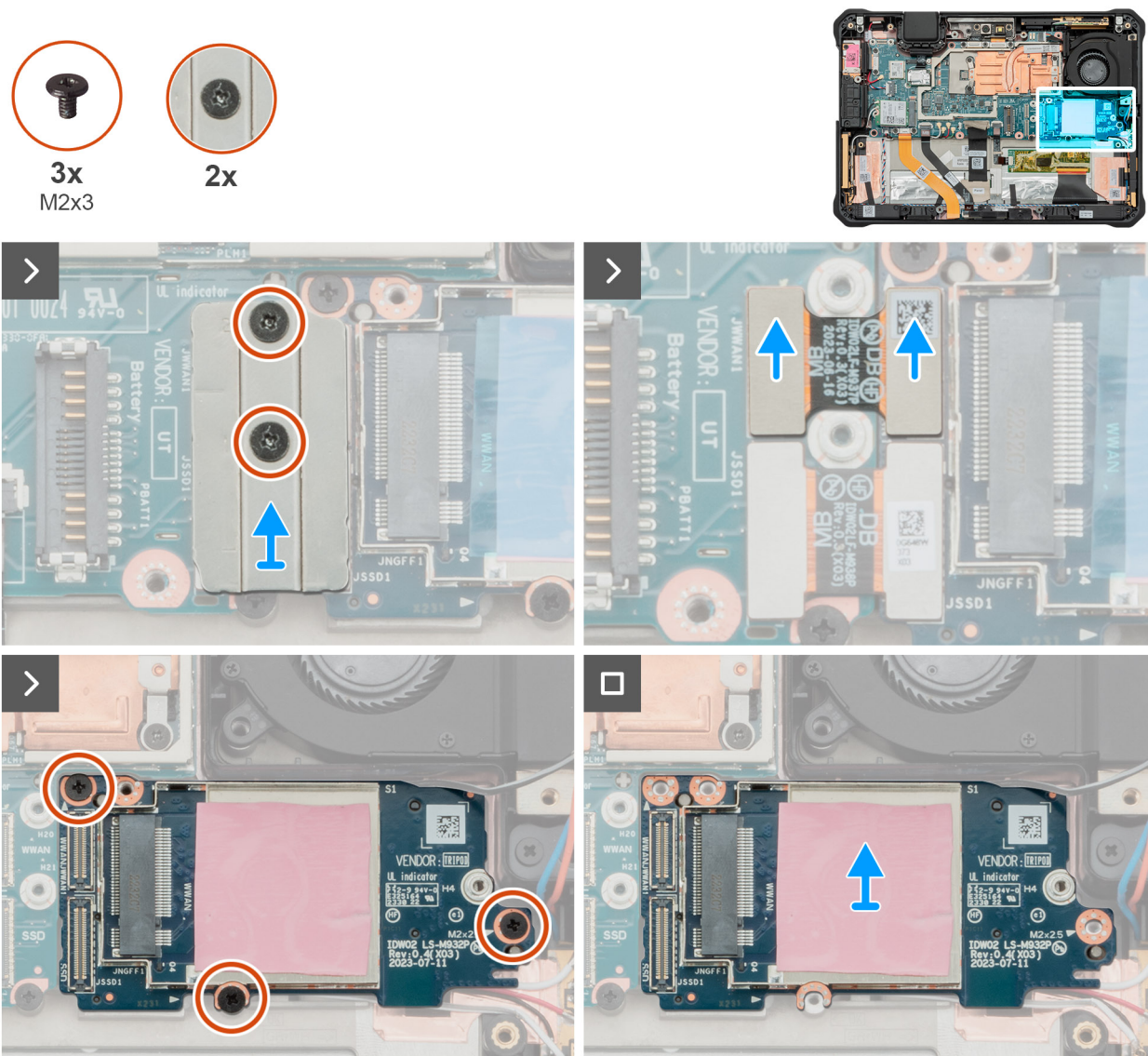
Figure 90. Removing the WWAN/SSD daughter-board
