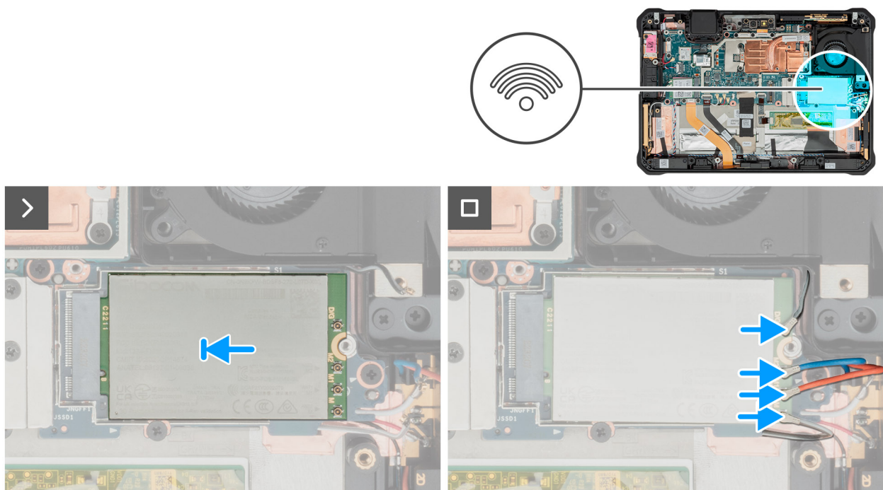
Figure 89. Installing the 5G WWAN card
