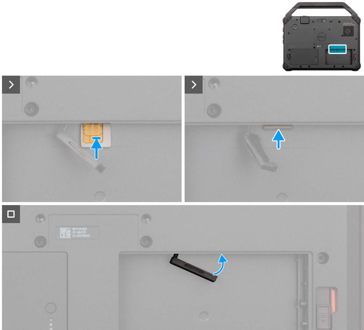
Figure 46. Inserting the SIM card
