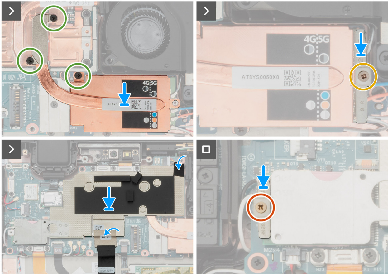
Figure 82. Installing the WWAN-card heat-sink
