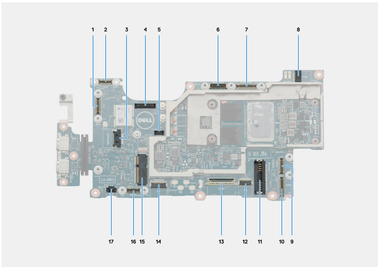
Figure 97. System board connectors
