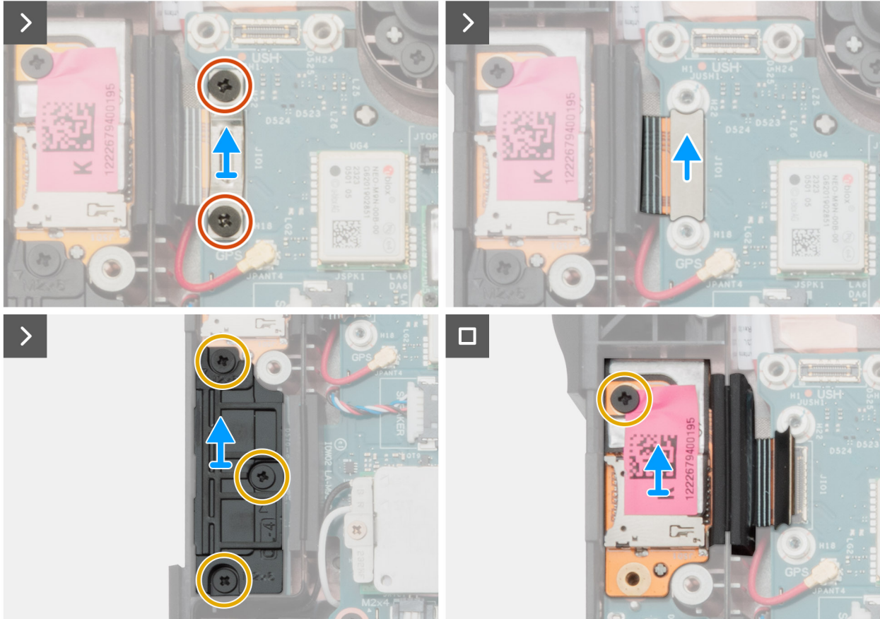
Figure 58. Removing the I/O daughter-board
