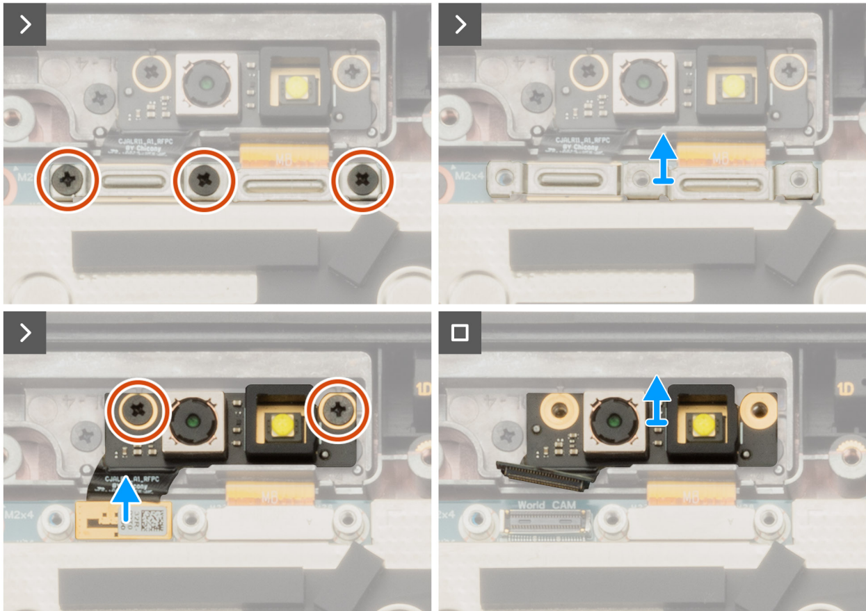
Figure 64. Removing the world-facing camera
