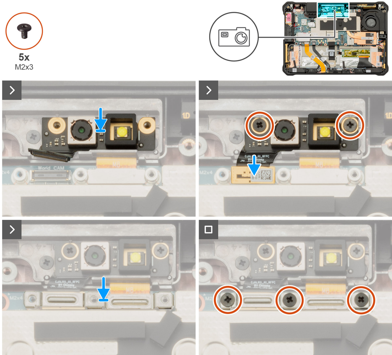
Figure 65. Installing the world-facing camera
