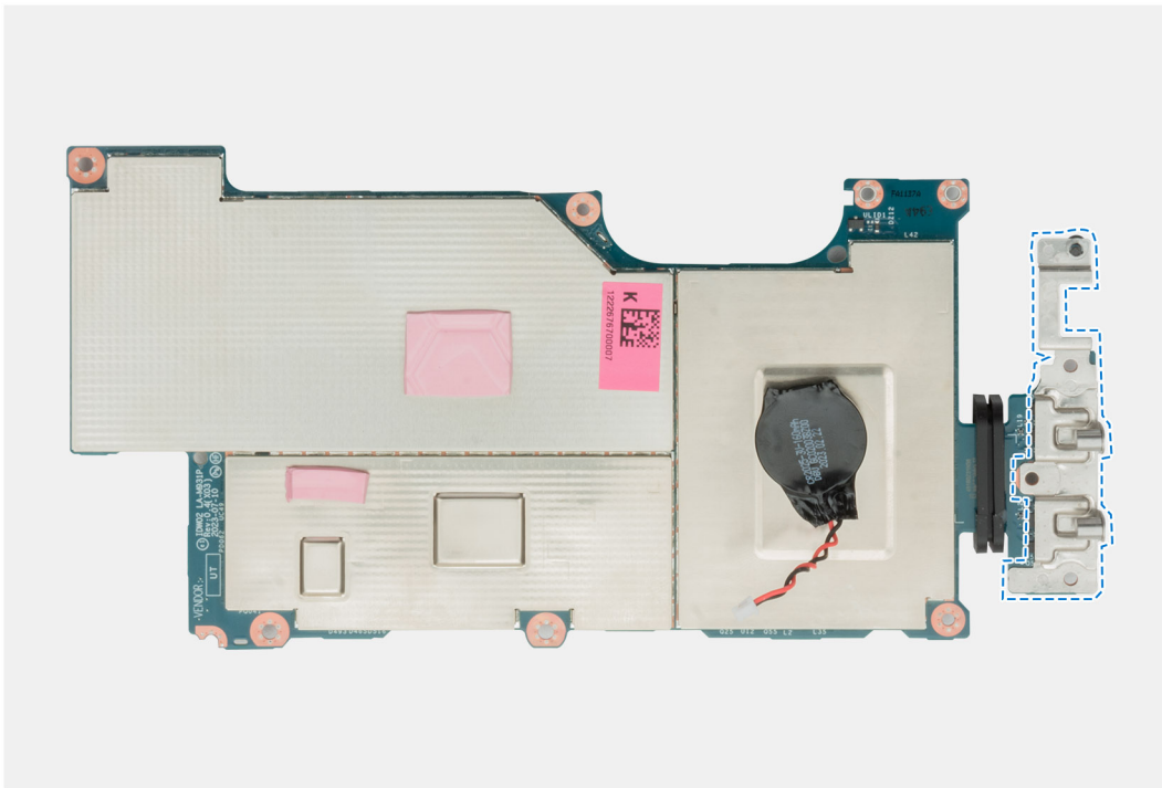
Figure 101. Removing the system board
