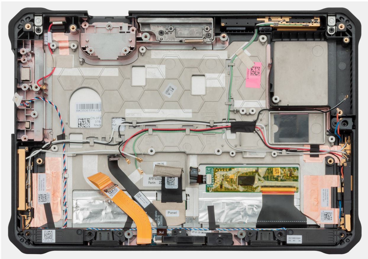
Figure 108. Removing the display assembly
