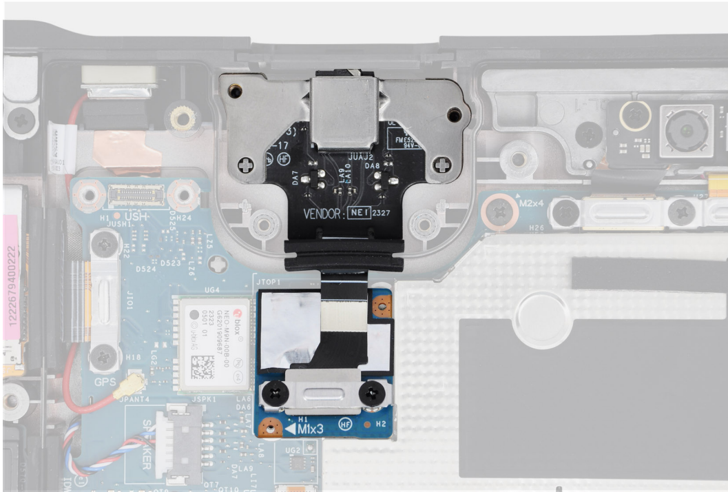
Figure 76. Installing the audio-jack assembly
