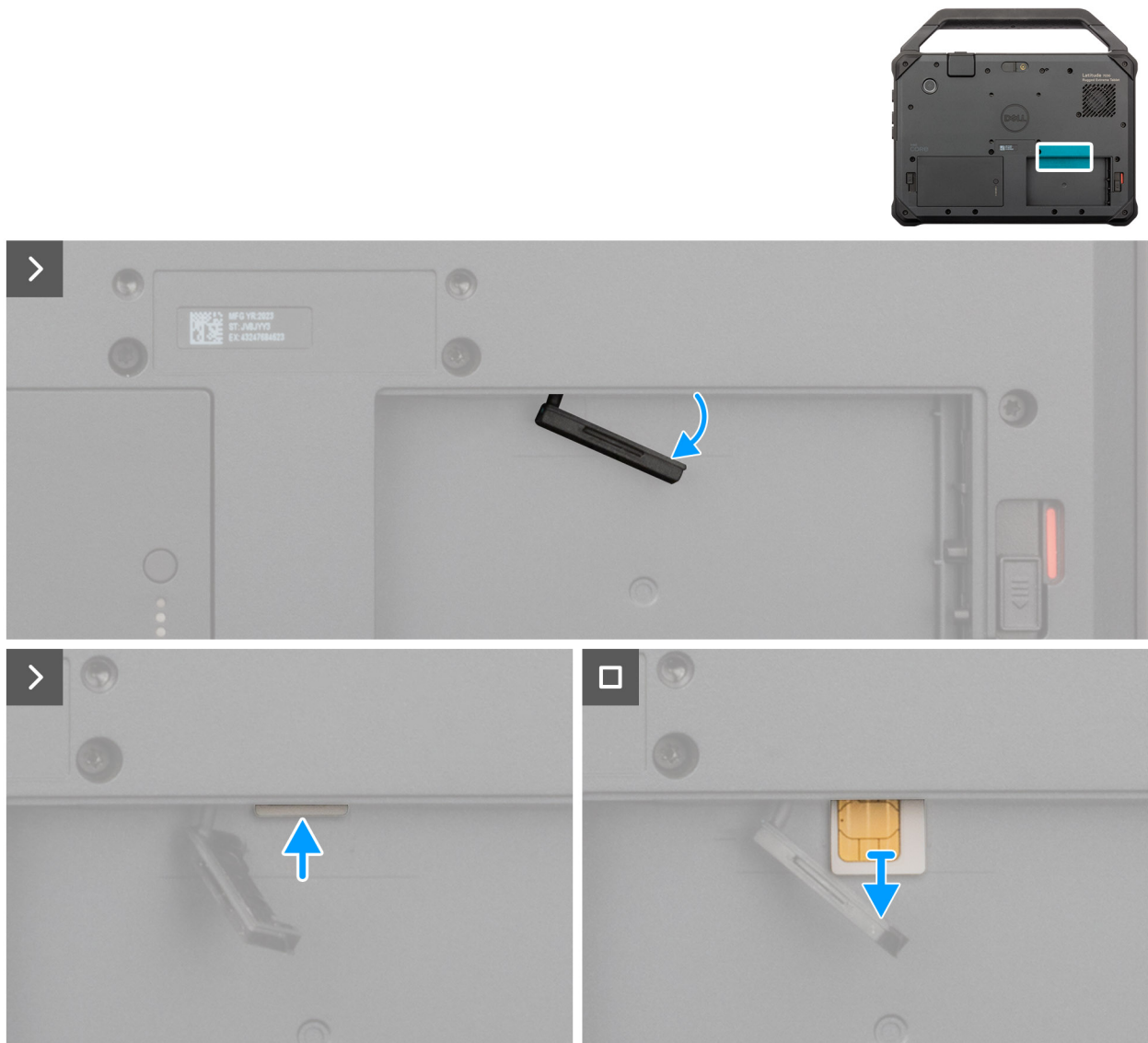
Figure 45. Removing the SIM card
