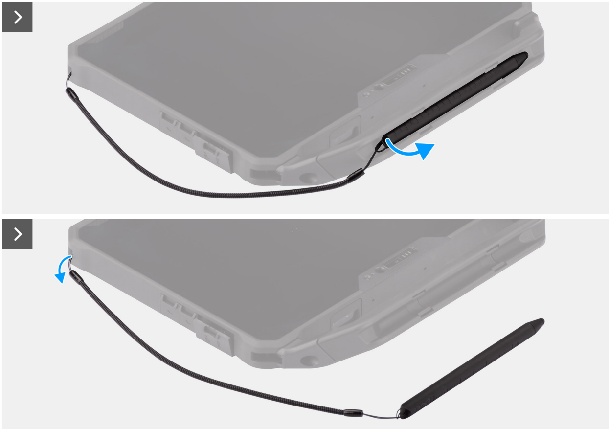
Figure 37. Removing the stylus
