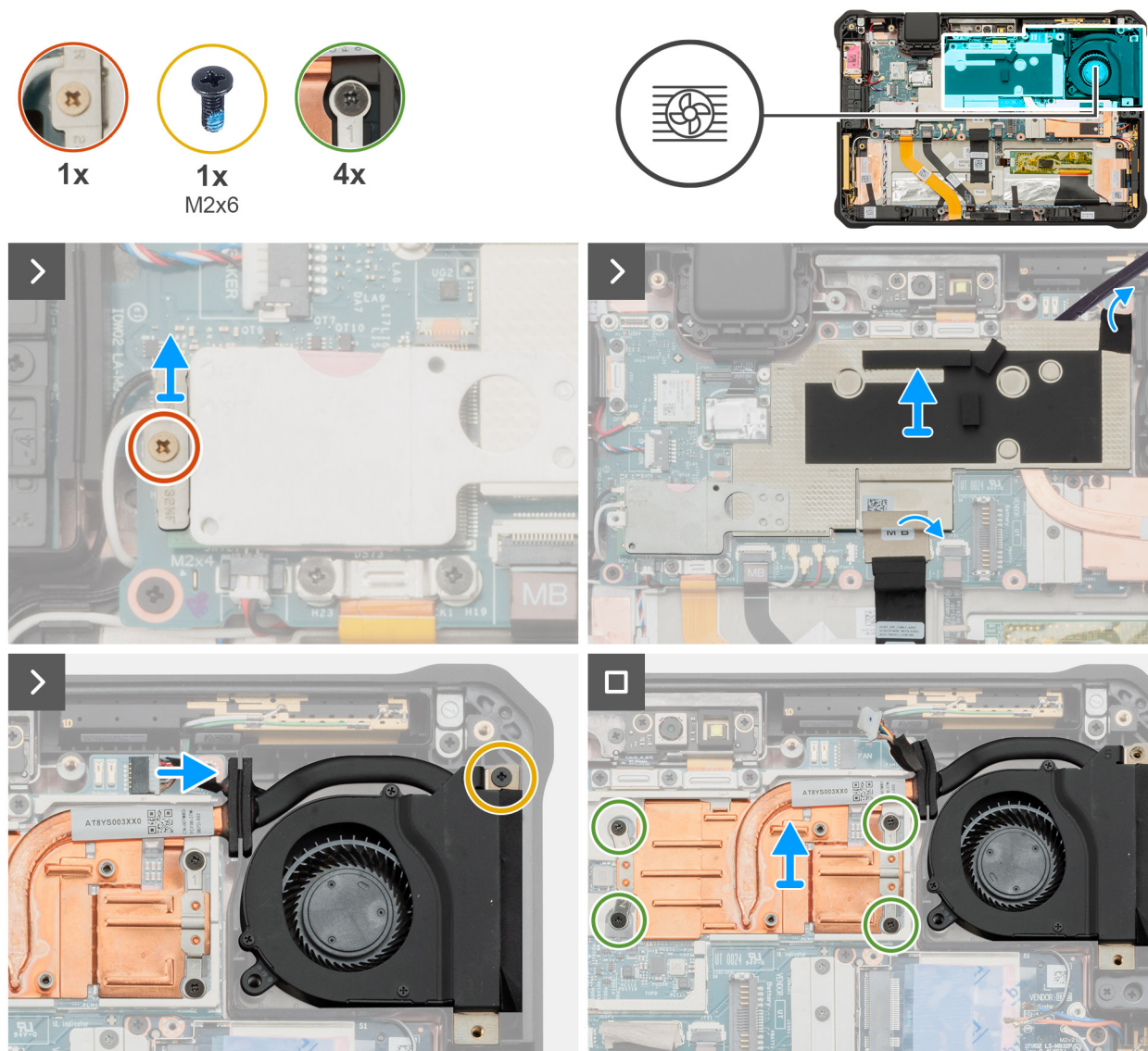
Figure 83. Removing the fan and heat-sink assembly
