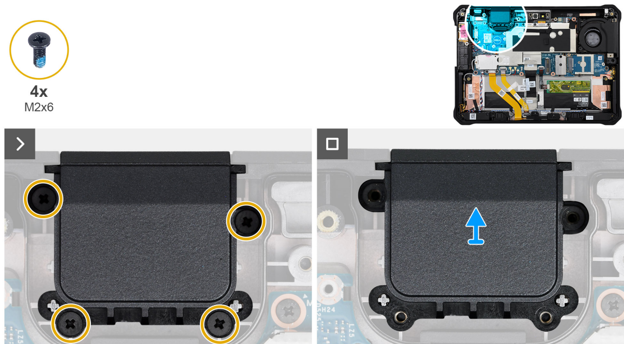
Figure 68. Removing the blank top-cover
