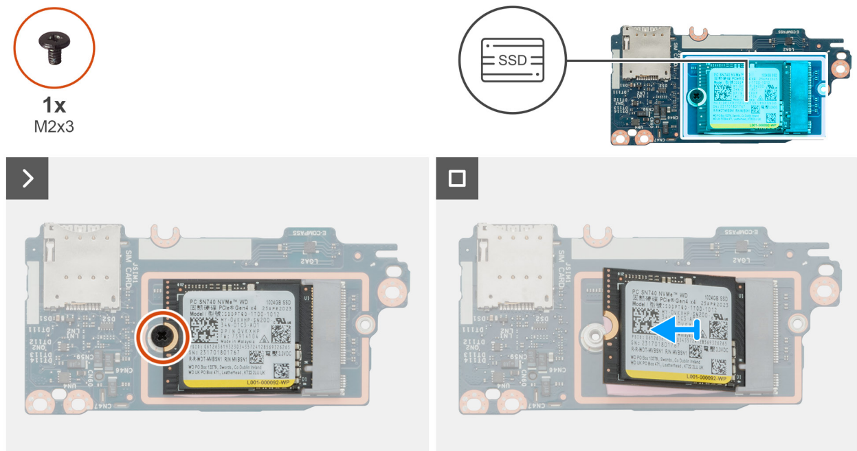
Figure 93. Removing the M.2 2230 solid-state drive
