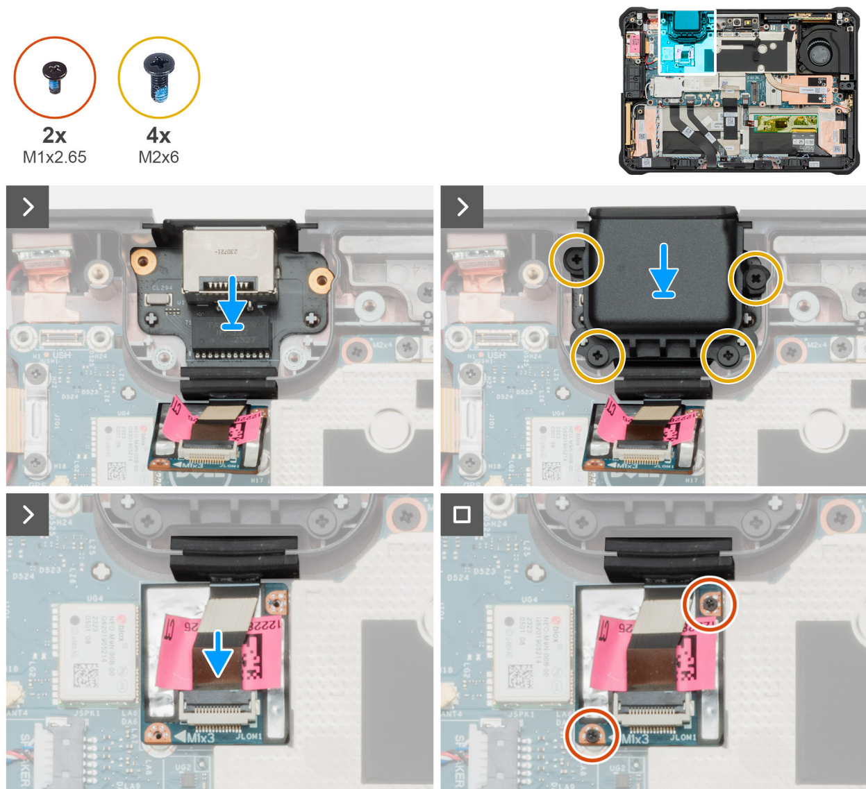
Figure 71. Installing the RJ45-port assembly
