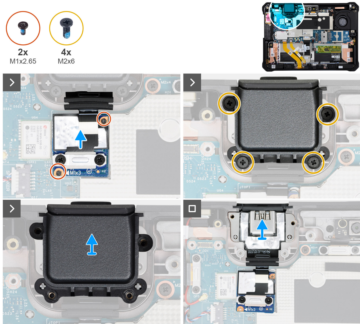
Figure 72. Removing the USB-port assembly
