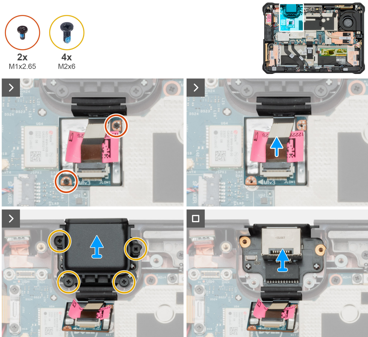
Figure 70. Removing the RJ45-port assembly
