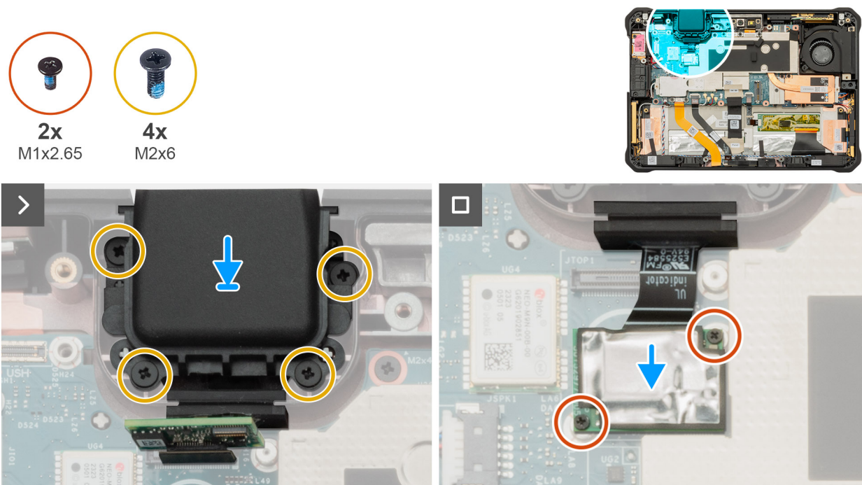
Figure 78. Installing the 1D-2D barcode-scanner assembly
