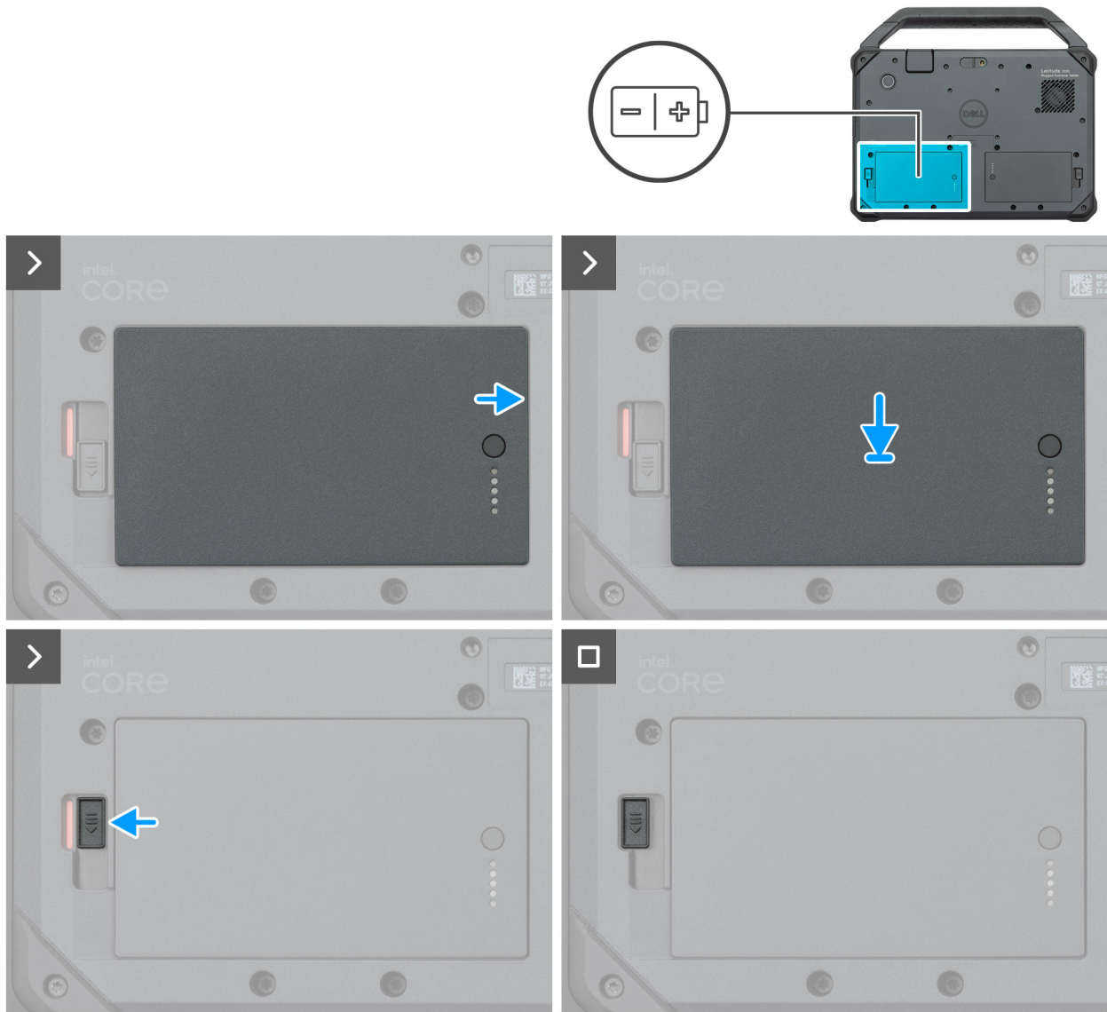
Figure 44. Installing the hot-swappable batteries
