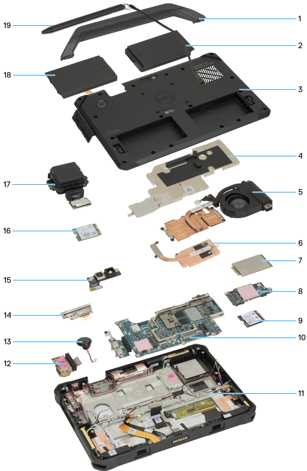
Figure 36. Major components of Latitude 7030 Rugged Extreme Tablet
