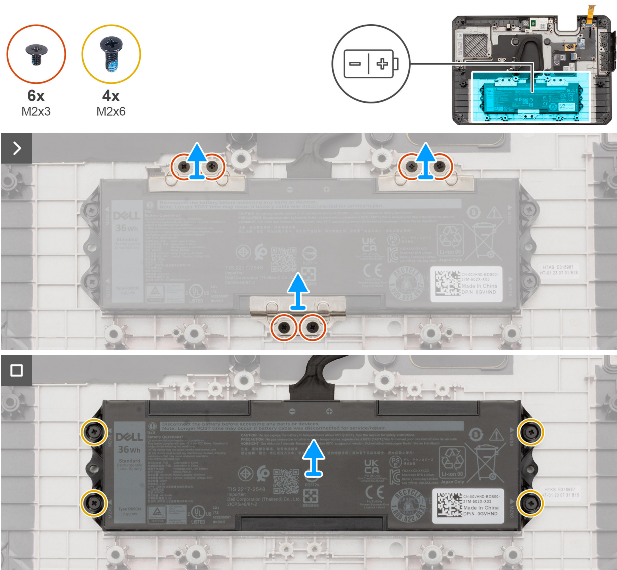
Figure 56. Removing the internal battery
