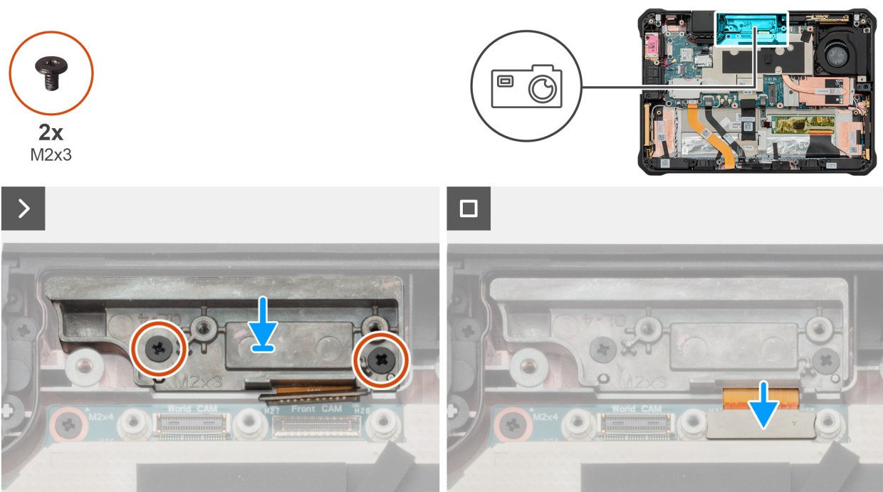
Figure 67. Installing the front camera and microphone assembly
