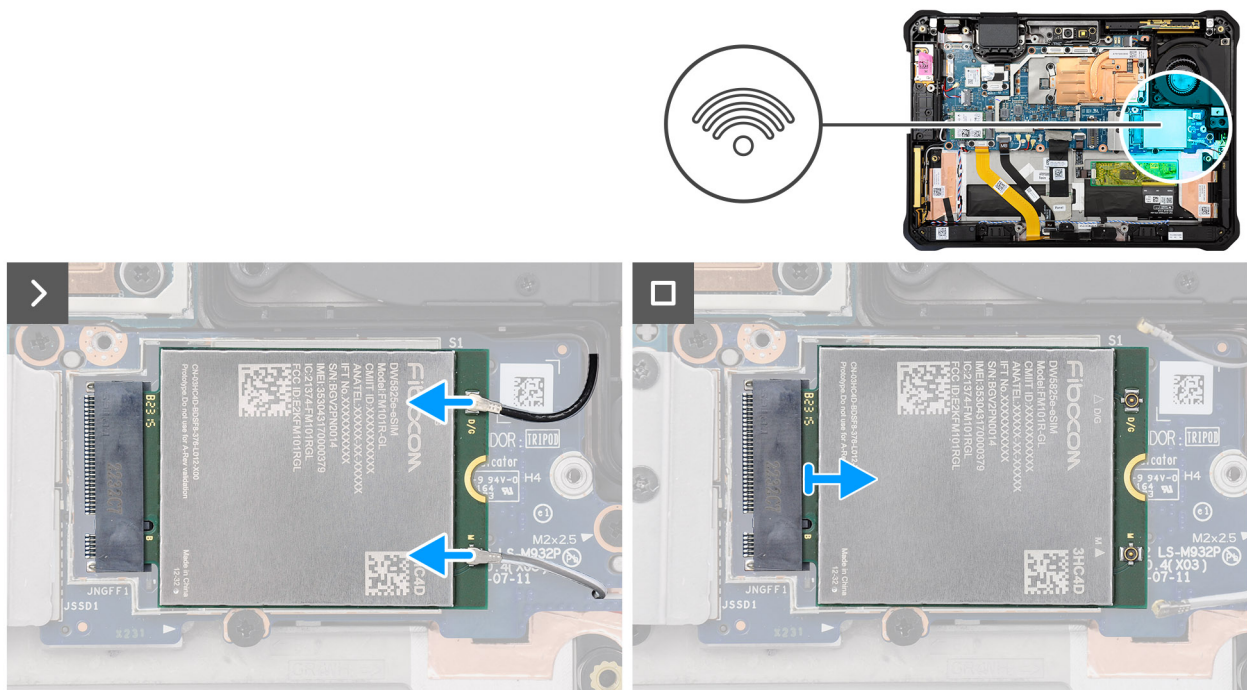
Figure 86. Removing the 4G WWAN card
