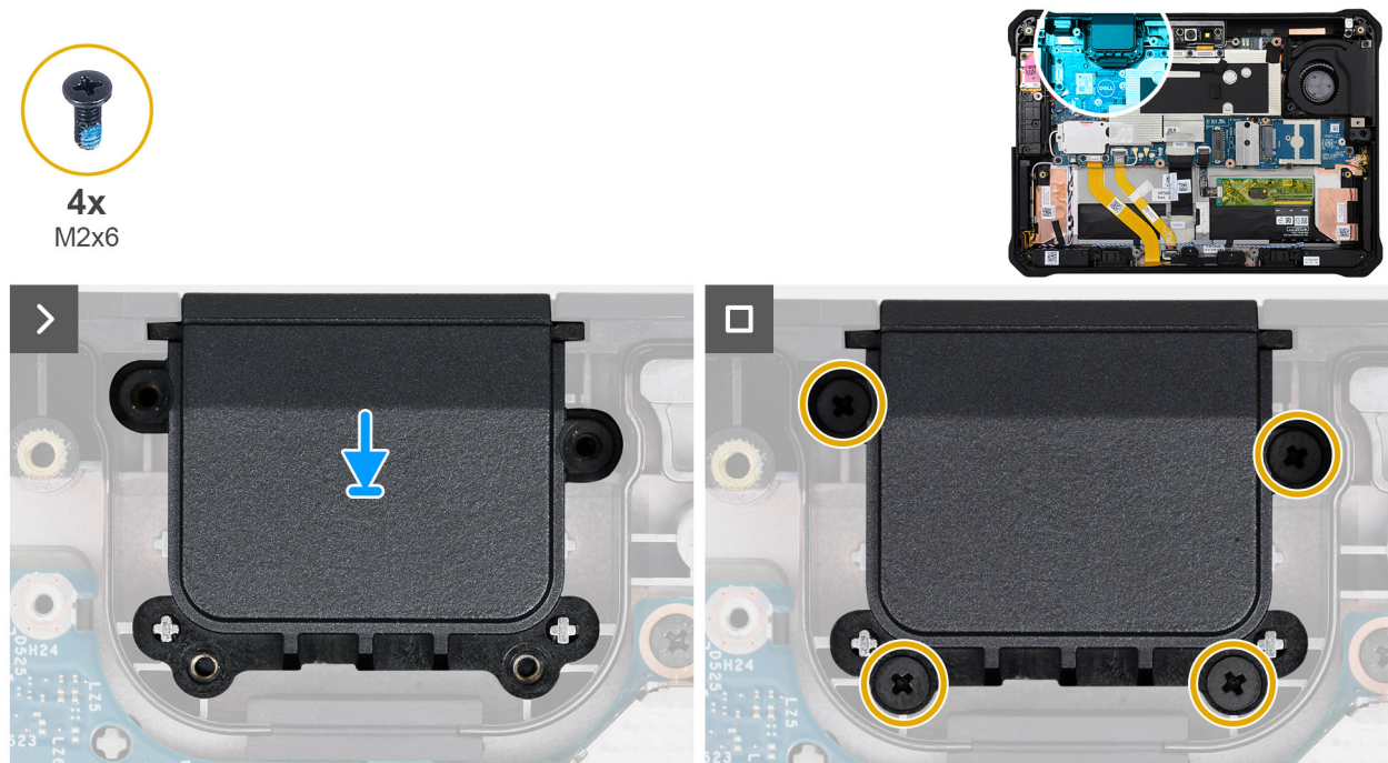
Figure 69. Installing the blank top-cover
