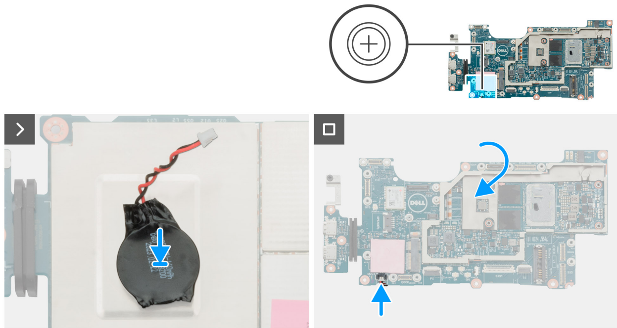
Figure 107. Installing the coin-cell battery
