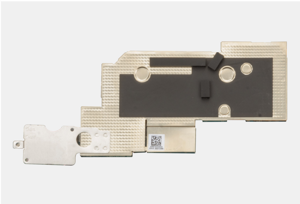
Figure 80. Removing the WWAN-card heat-sink
