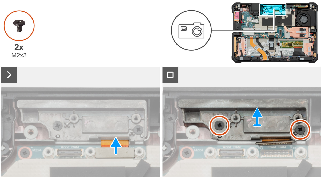
Figure 66. Removing the front camera and microphone assembly
