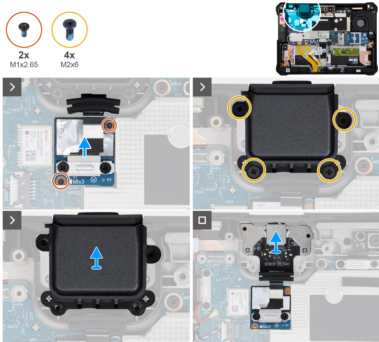
Figure 74. Removing the audio-jack assembly
