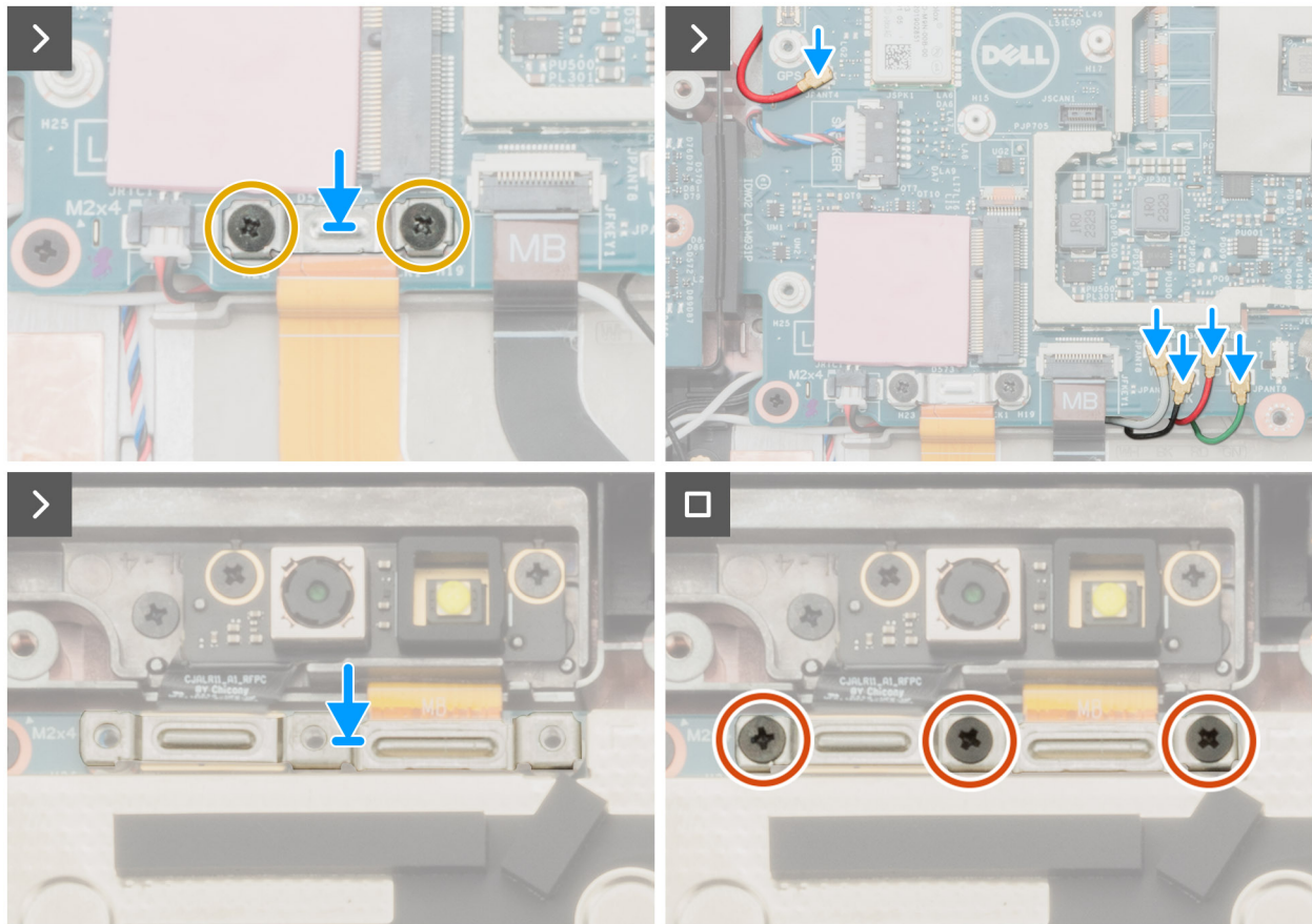
Figure 105. Installing the system board
