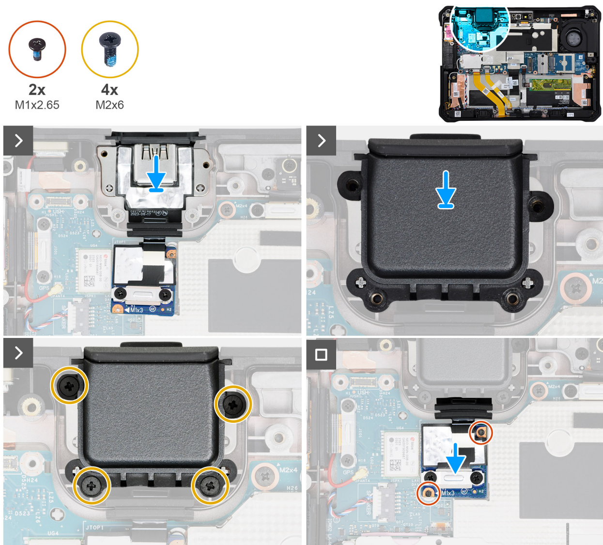
Figure 73. Installing the USB-port assembly
