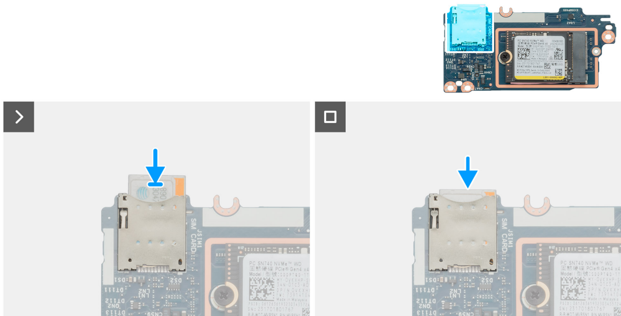
Figure 96. Installing the SIM card (for internal battery)
