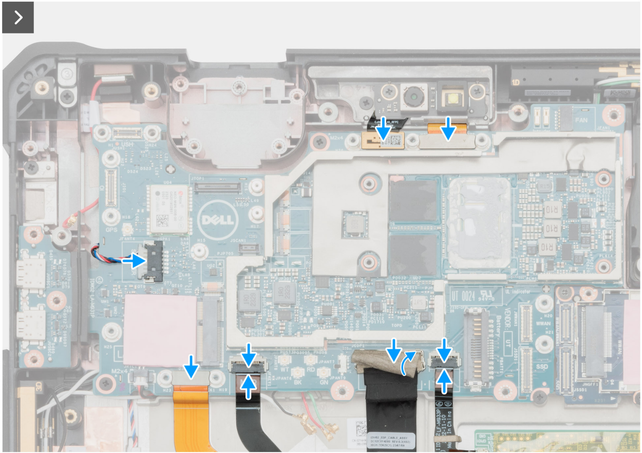
Figure 104. Installation the system board
