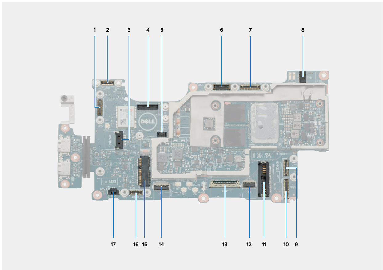
Figure 102. System board connectors
