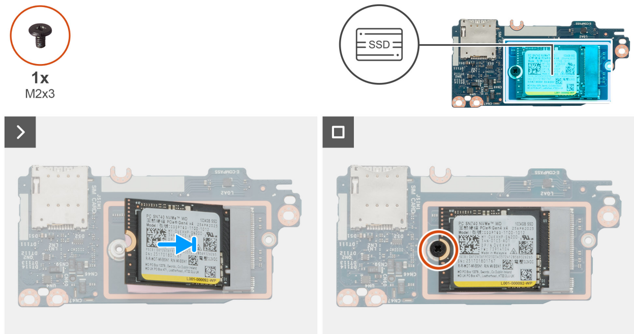
Figure 94. Installing the M.2 2230 solid-state drive
