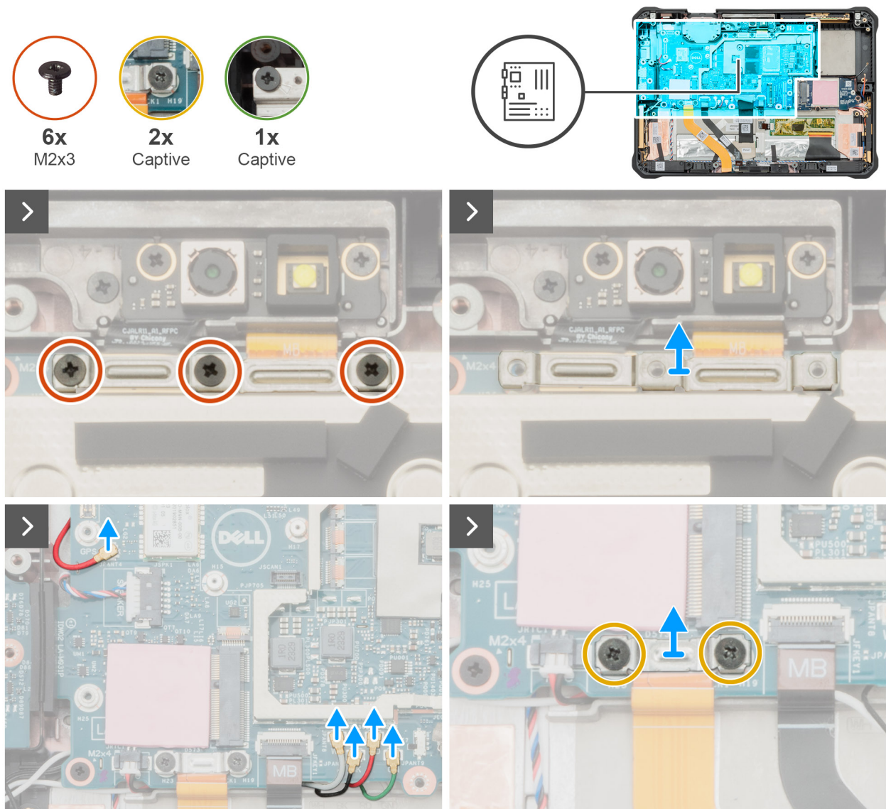
Figure 98. Removing the system board
