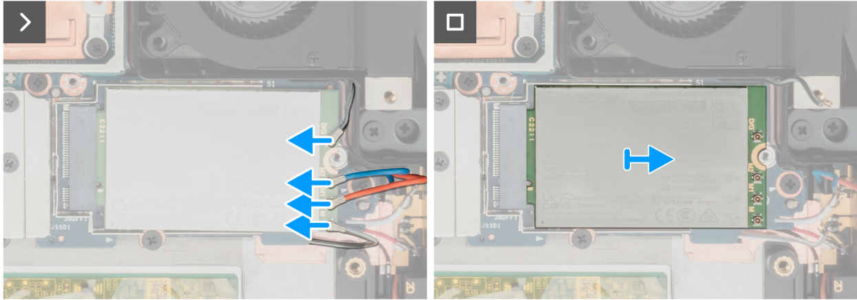
Figure 87. Removing the 5G WWAN card
