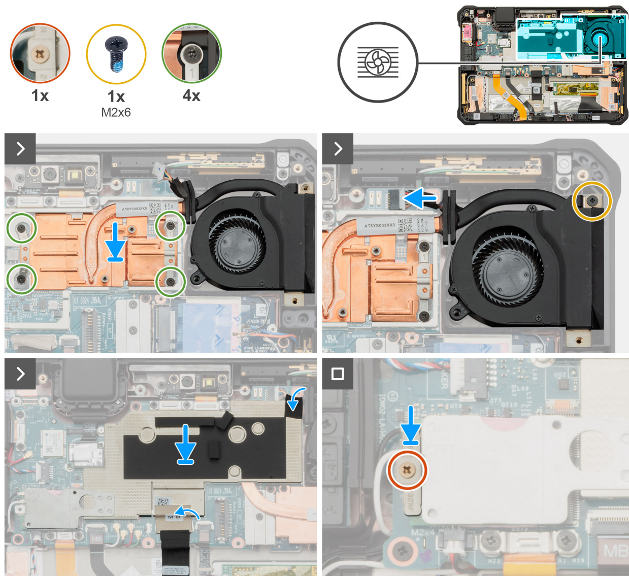
Figure 85. Installing the fan and heat-sink assembly
