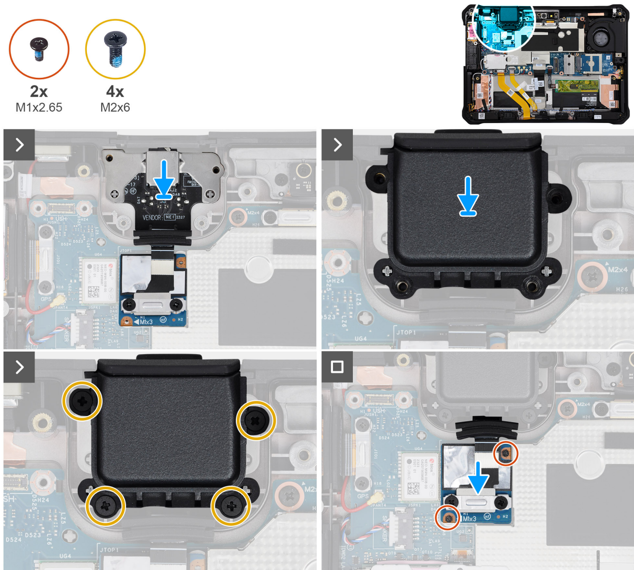
Figure 75. Installing the audio-jack assembly
