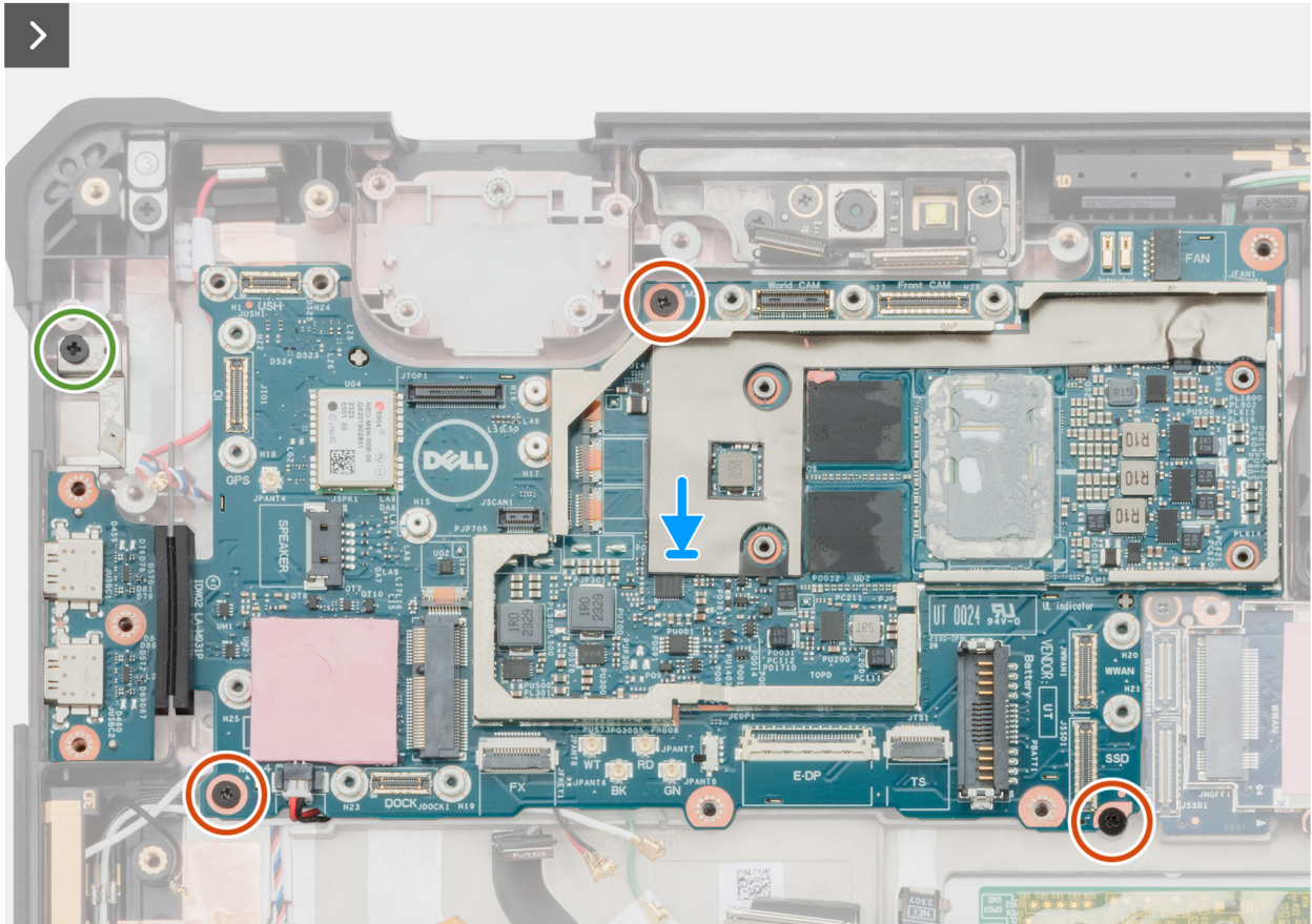
Figure 103. Installation the system board
