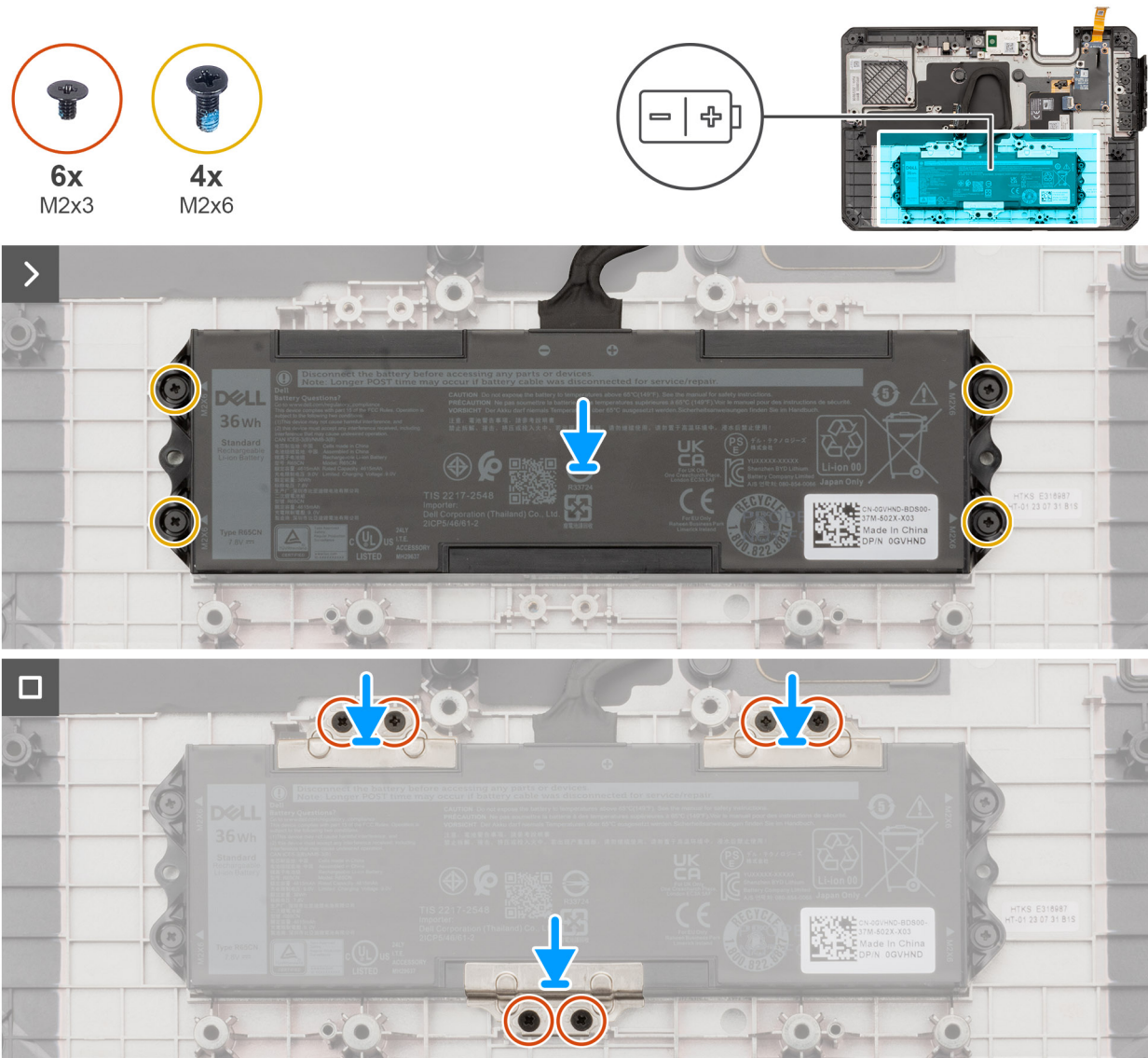
Figure 57. Installing the internal battery
