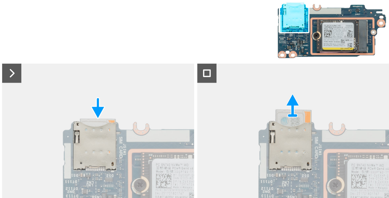
Figure 95. Removing the SIM card (for internal battery)
