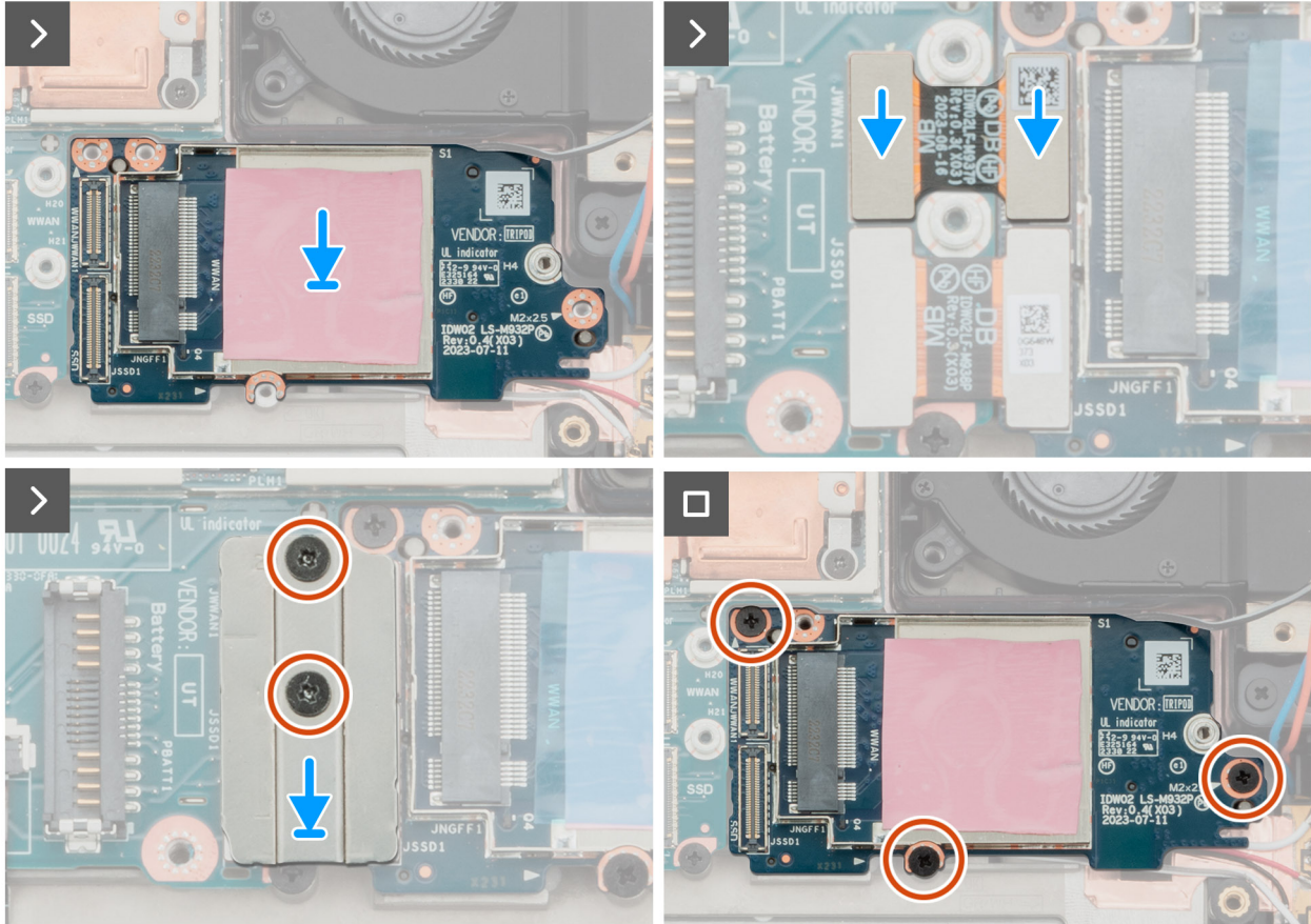
Figure 92. Installing the WWAN/SSD daughter-board
