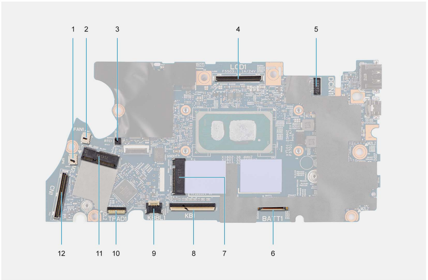
Figure 2. System-board connectors
