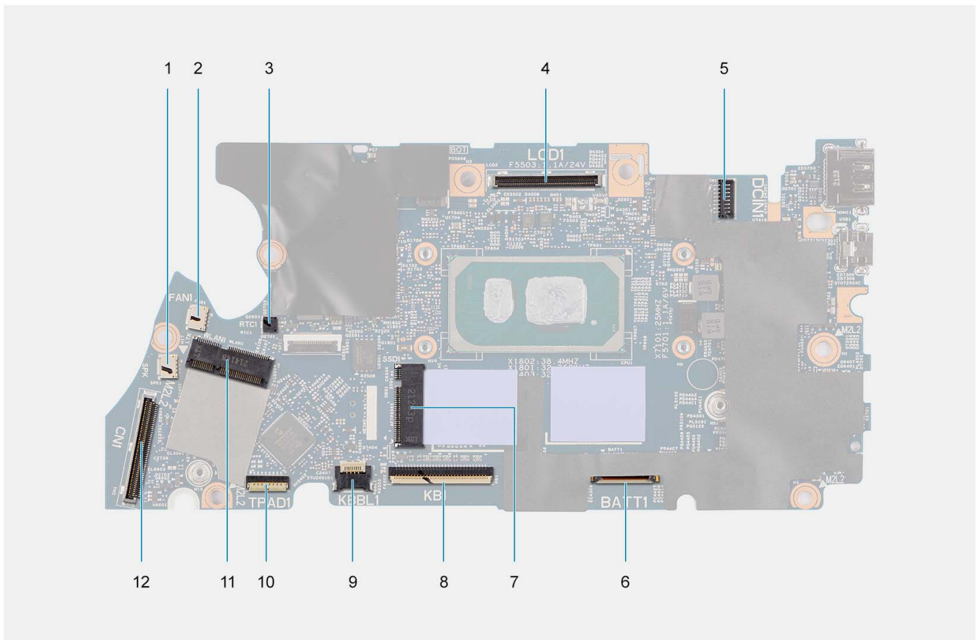
Figure 1. System-board connectors
