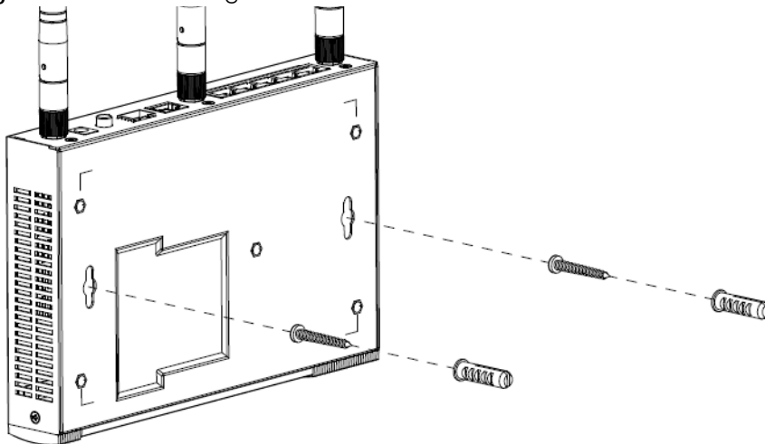
Figure 77 Wall Mounting
