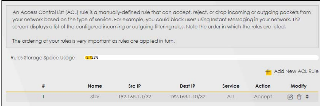
Figure 75 Security > Firewall > Access Control
