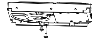
Figure 3-1 Installing the hard disk screws
