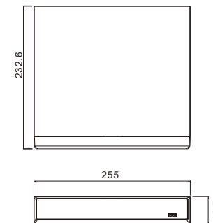
Figure 2-1 Dimensions (Unit:mm)
