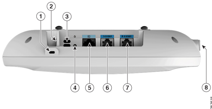
Figure 2: C9136I Top View with Connectors and Ports
