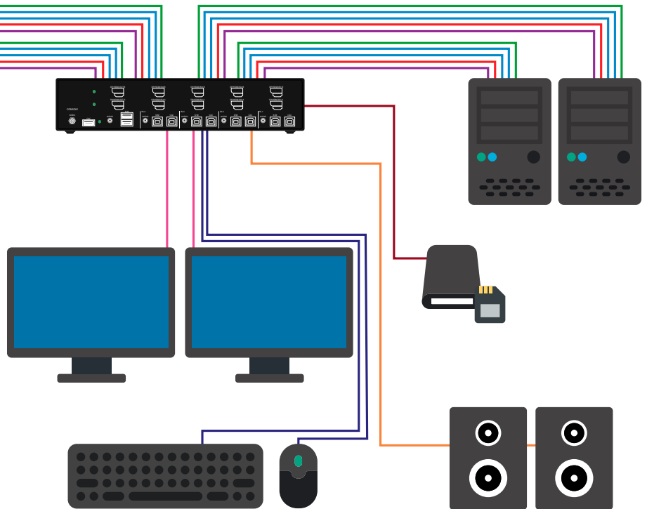
Figure 1-7: KVS4-2004HVX
