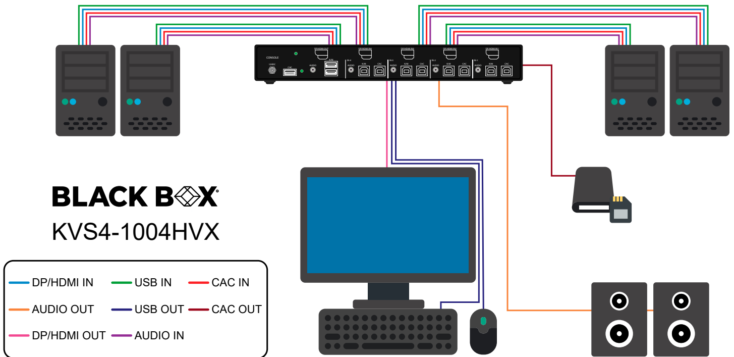
Figure 1-3: KVS4-1004HVX
