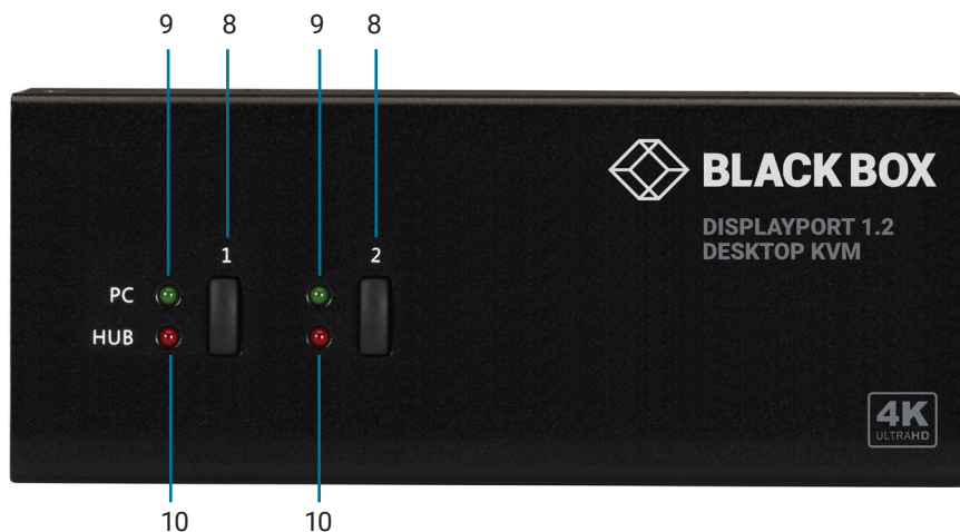
FIGURE 2-1. FRONT PANEL OF THE KV6222DP
