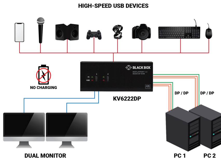
FIGURE 3-2. CONNECTION ILLUSTRATION
