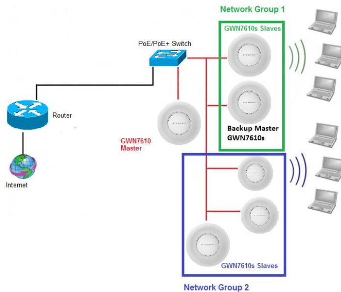
Figure 36: Failover Master
