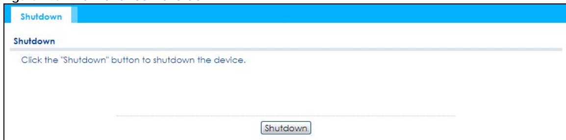
Figure 140 Maintenance > Shutdown
