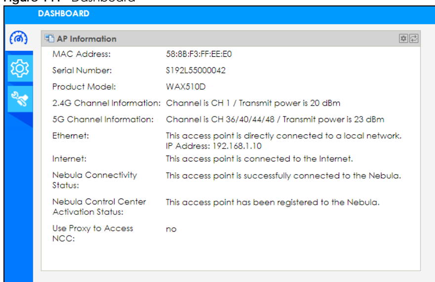
Figure 141 Dashboard
