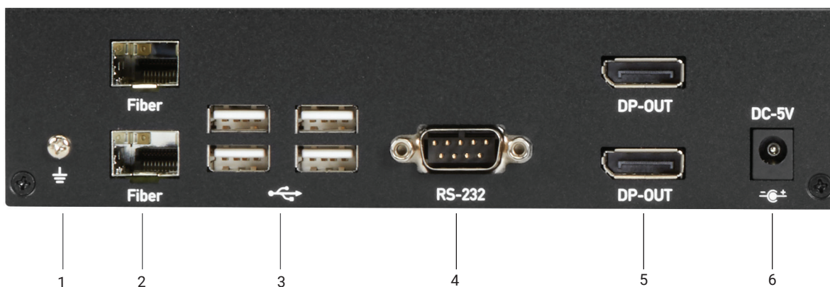
FIGURE 2-12. DUAL-HEAD FIBER RECEIVER BACK PANEL
