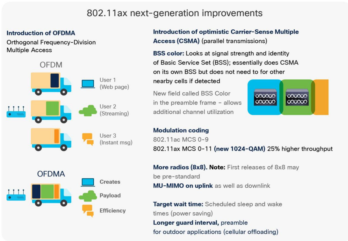
Figure 2. 802.11ax improvements
