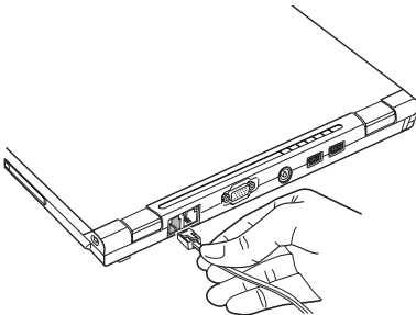
Connecting the telephone cable to the modem port
