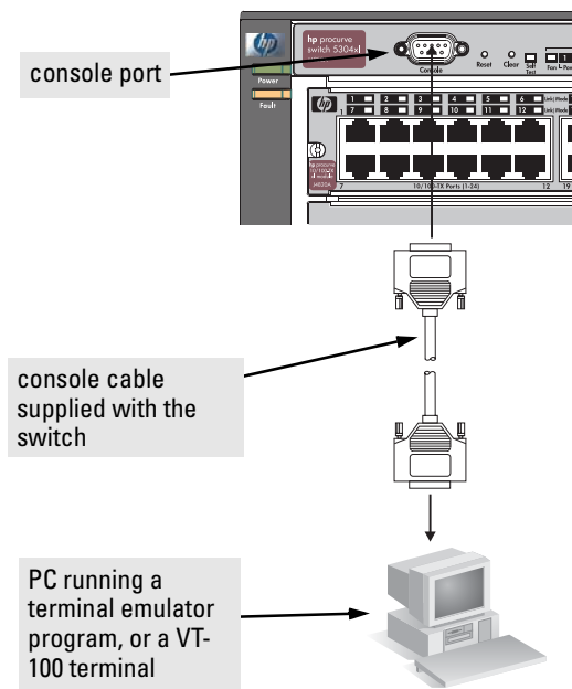
Figure 2-13. Connecting a console
