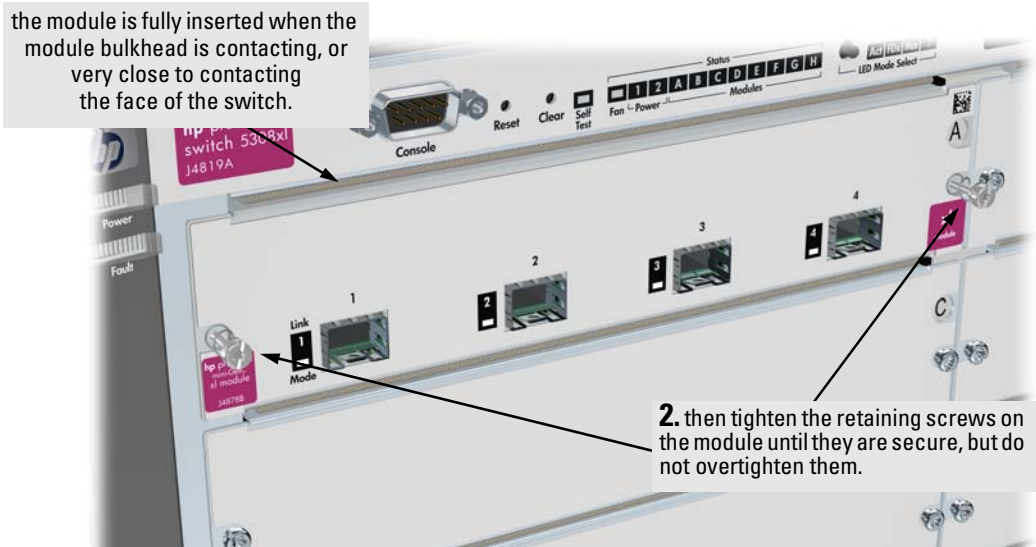
Figure 2-2. Tighting module retaining screws
