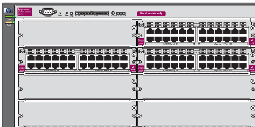
Figure 1-4. Example 5372xl bundle
