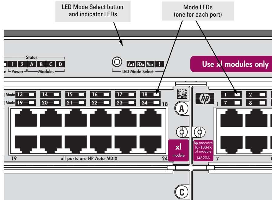
Figure 1-7. Example Mode Select button and Mode LEDs
