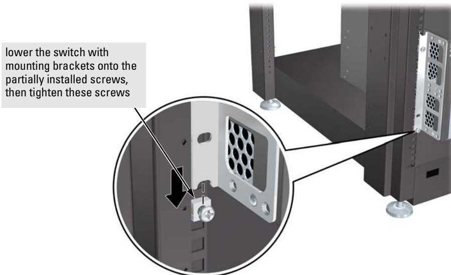
Figure 2-9. Setting the bracket notch
