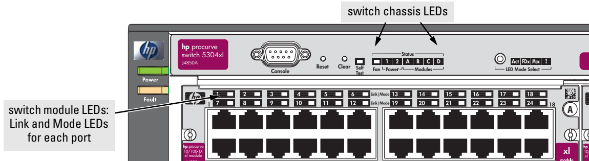
Figure 2-6. Switch LEDs
