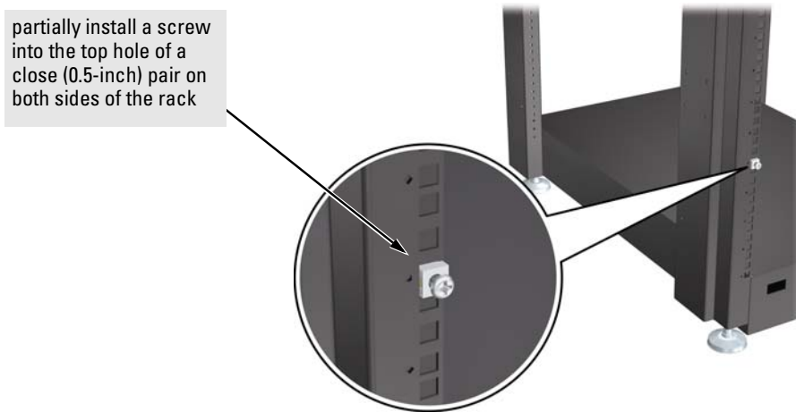
Figure 2-8. Partially installed screw for bracket notch
