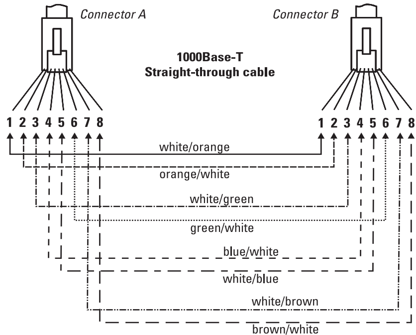
Cable Diagram
