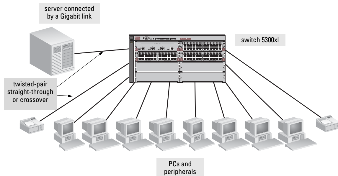
Figure 2-14. Basic topology
