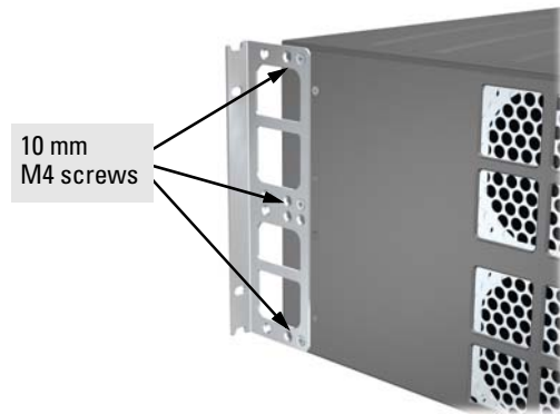
Figure 2-11. Attaching brackets to the rear of the switch
