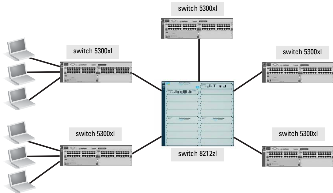
Figure 2-17. 10-GbE Aggregation Topology
