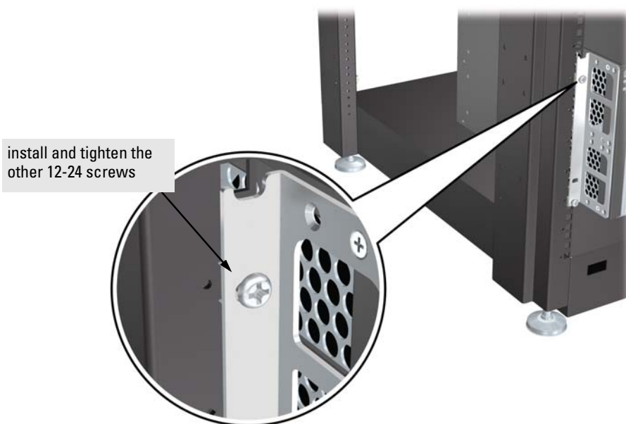
Figure 2-10. Installing the final rack mounting screw
