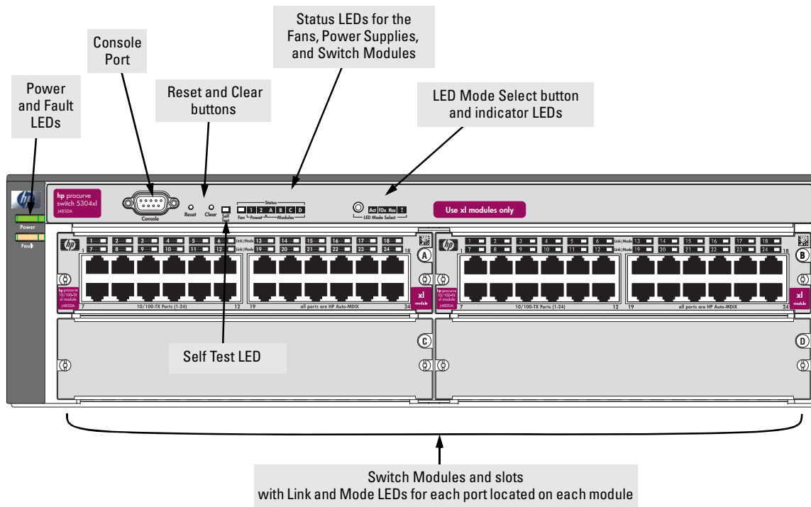
Figure 1-6. Example front description
