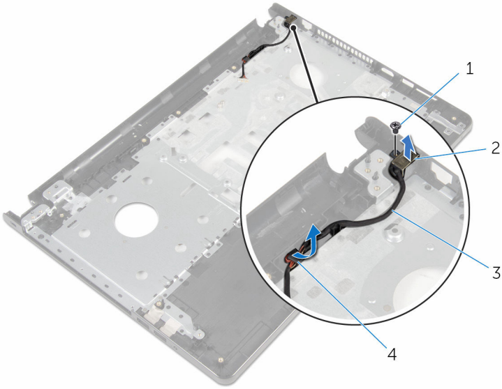
Figure 38. Removing the power-adapter port
