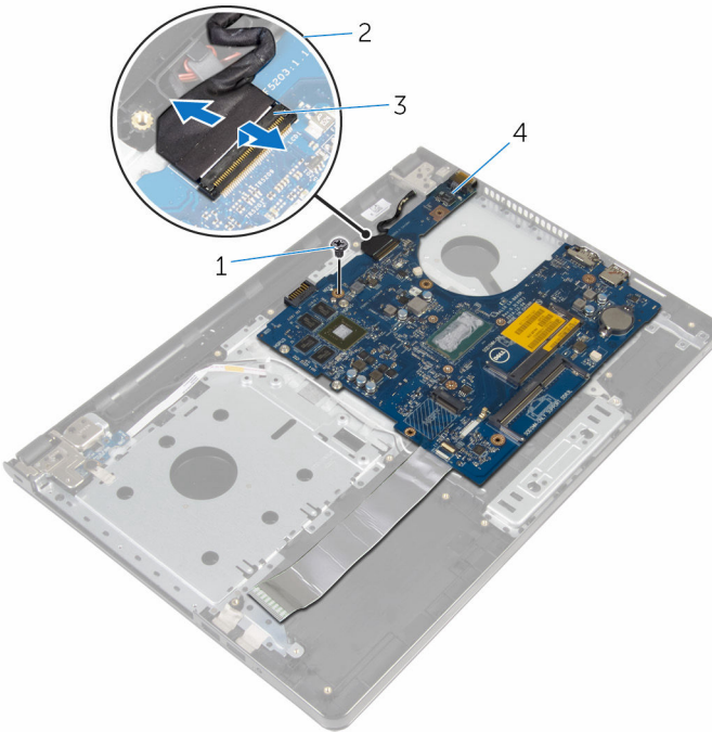
Figure 27. Removing the display cable and screw from the system board
