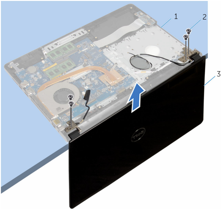
Figure 31. Removing the display assembly
