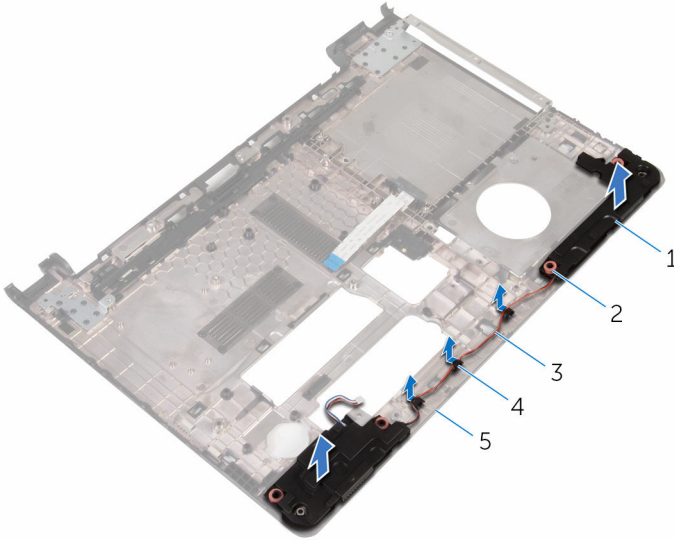
Figure 22. Removing the speakers
