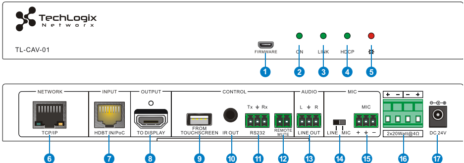
Figure 2-2 Receiver
