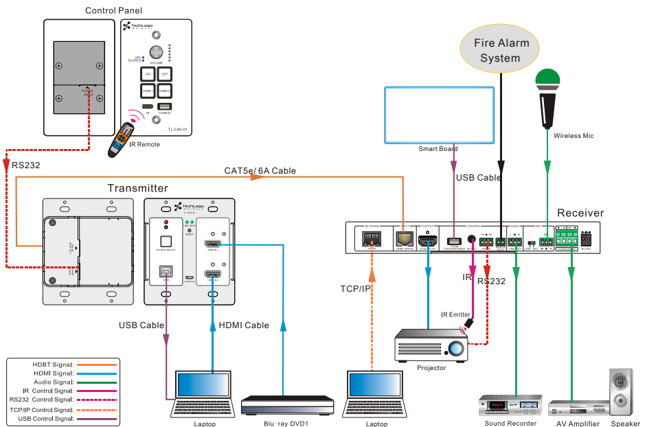
Figure 3-1 System Diagram
