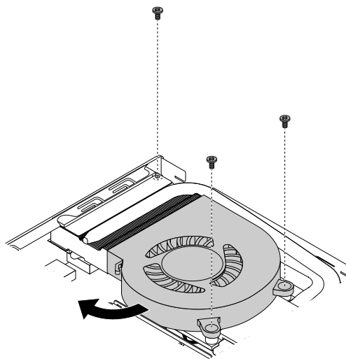
Figure 43. Removing the system fan (for M900x)
