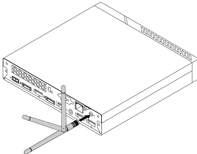
Figure 84. Installing the rear Wi-Fi antenna
