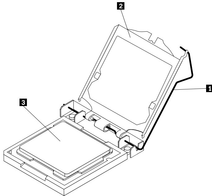
Figure 59. Opening the retainer to access the microprocessor
