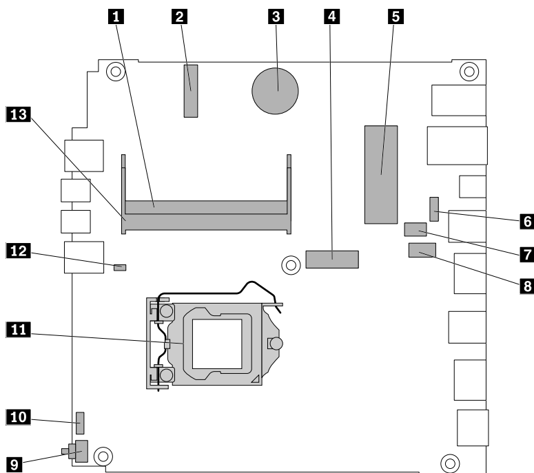
Figure 5. Parts on the system board
