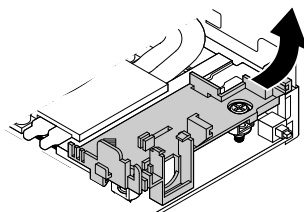
Figure 52. Removing the internal speaker holder (for M900x)
