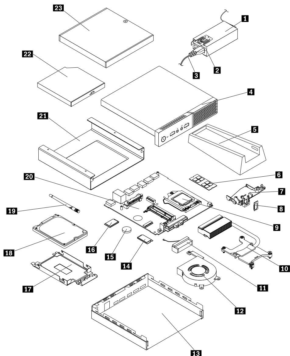
Figure 4. Major FRUs and CRUs
