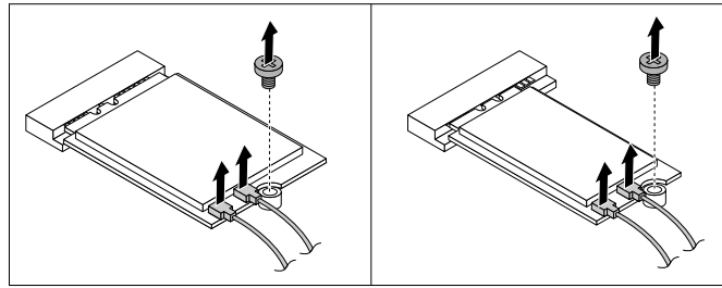
Figure 75. Removing the Wi-Fi card cables
