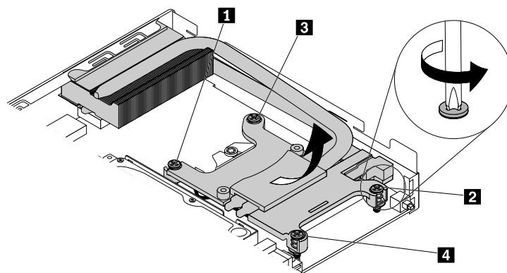
Figure 56. Removing the heat sink (for M900x)
