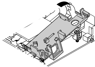
Figure 54. Installing the internal speaker holder (for M900x)
