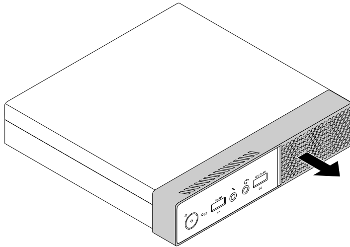
Figure 38. Removing the dust shield
