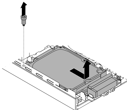
Figure 62. Removing the storage drive bracket
