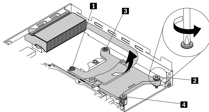
Figure 55. Removing the heat sink (for M700 and M900)
