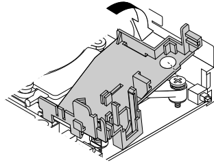
Figure 53. Installing the internal speaker holder (for M700 and M900)
