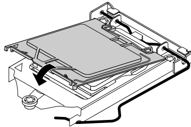
Figure 86. Installing the microprocessor socket cover
