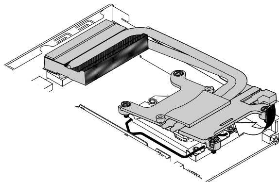
Figure 58. Installing the heat sink (for M900x)
