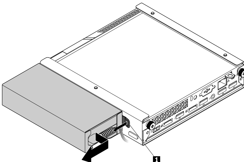
Figure 36. Removing the power adapter bracket
