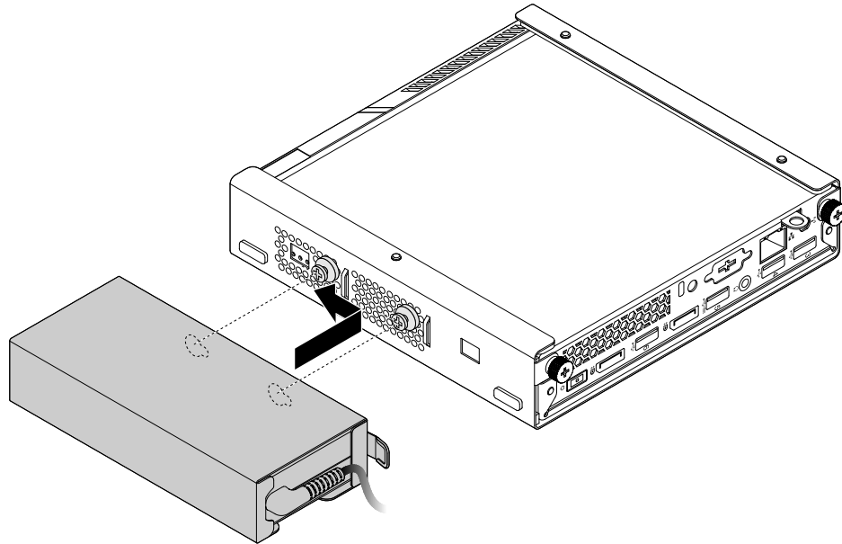
Figure 37. Installing the power adapter bracket
