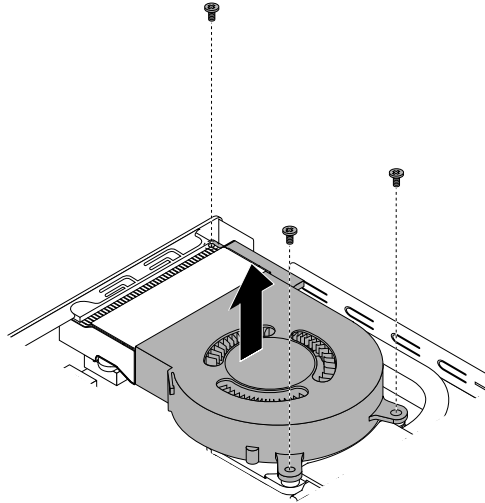
Figure 42. Removing the system fan (for M700 and M900)
