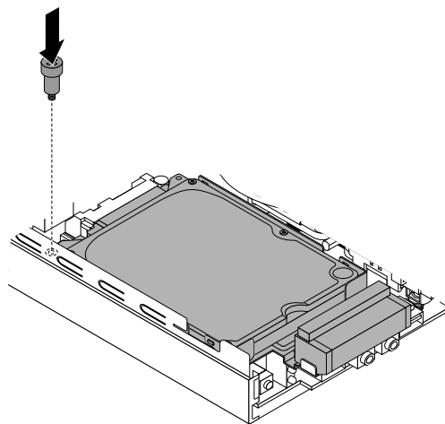
Figure 66. Installing the storage drive bracket screw
