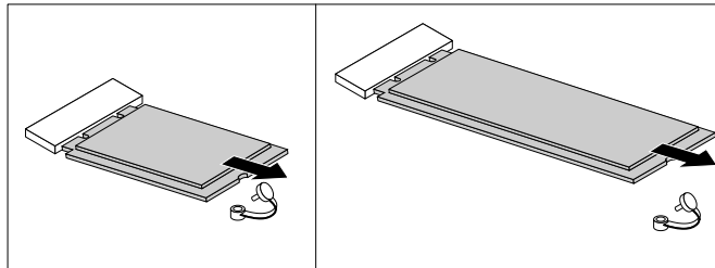
Figure 68. Removing the M.2 storage drive
