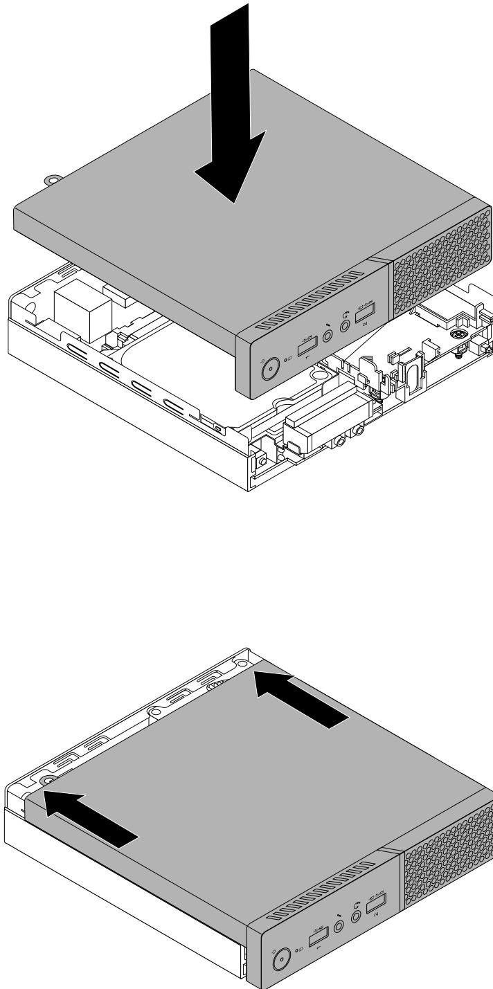
Figure 87. Installing the computer cover
