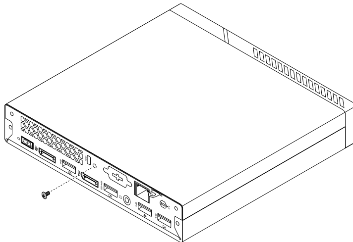
Figure 39. Removing the computer cover screw
