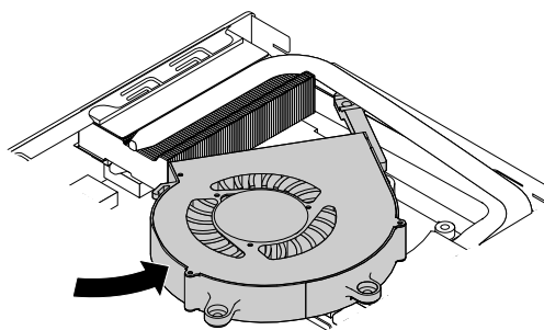
Figure 45. Installing the system fan (for M900x)
