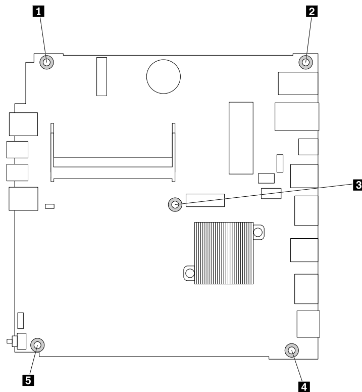
Figure 85. Removing the five screws that secure the system board
