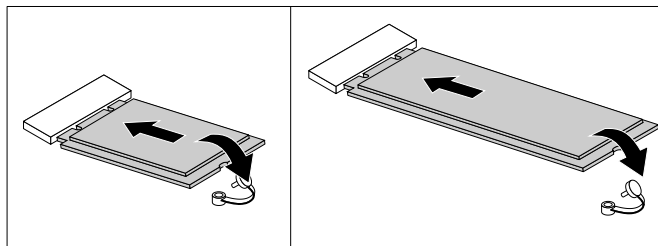
Figure 69. Installing the M.2 storage drive
