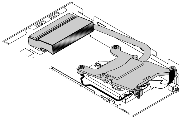
Figure 57. Installing the heat sink (for M700 and M900)
