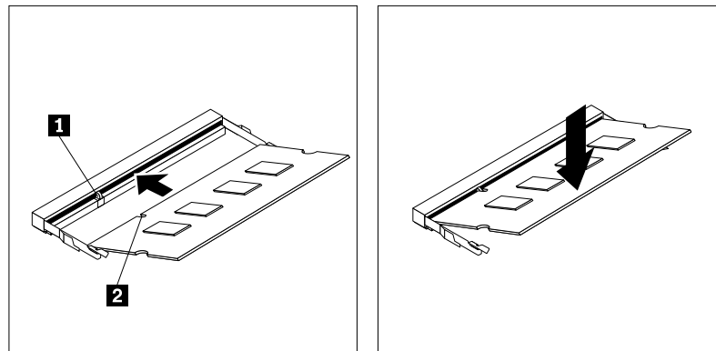
Figure 72. Installing the memory module
