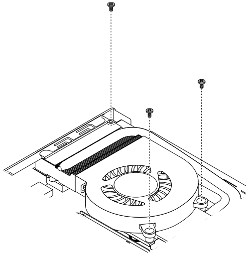
Figure 47. Installing the system fan screws (for M900x)
