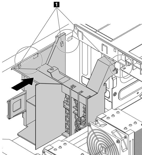
Figure 52. Reinstalling the multi-function bracket
