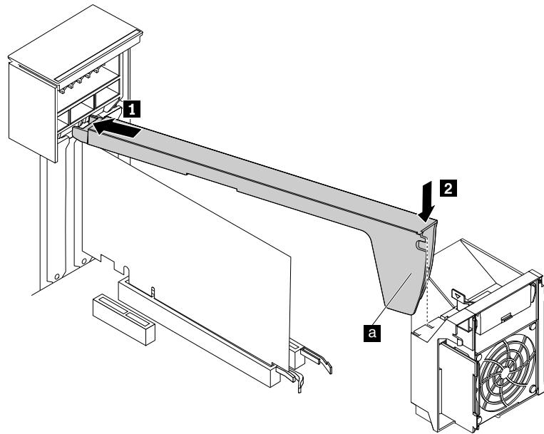
Figure 70. Installing the PCI card retainer
