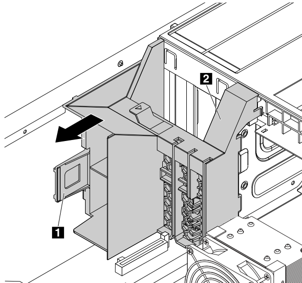
Figure 51. Removing the multi-function bracket
