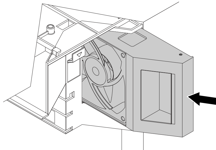
Figure 50. Installing the front fan assembly
