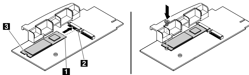
Figure 48. Installing the M.2 solid-state drive
