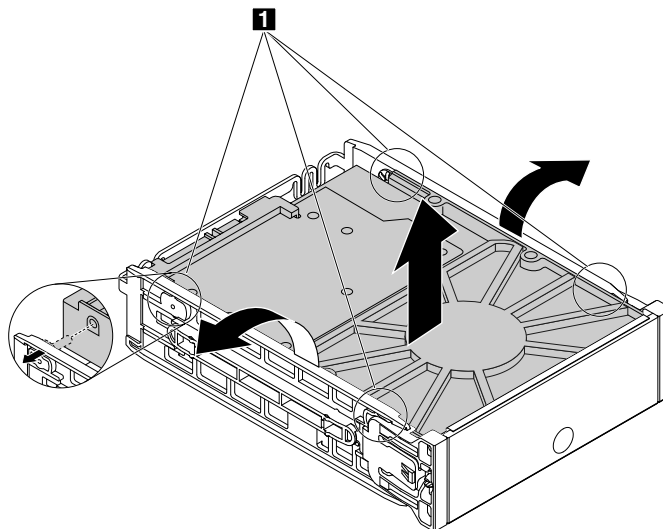
Figure 36. Removing the storage drive from the bracket
