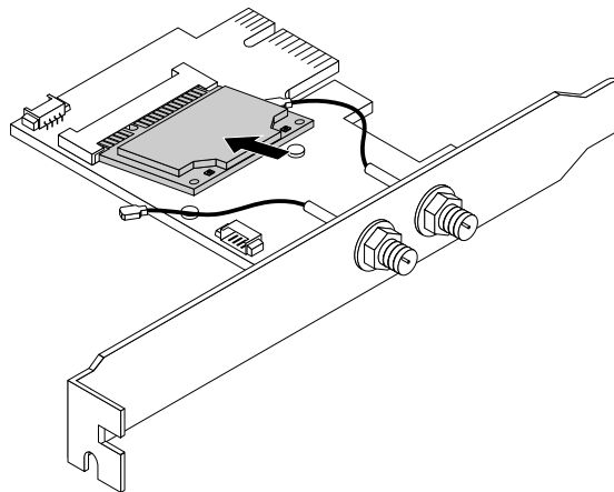
Figure 96. Installing the Wi-Fi card module
