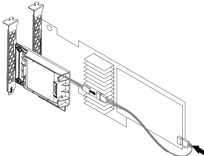
Figure 81. Connecting the super capacitor module cable
