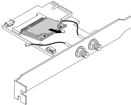
Figure 95. Removing the Wi-Fi card module
