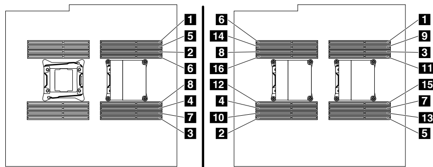
Figure 82. The order of installing memory modules
