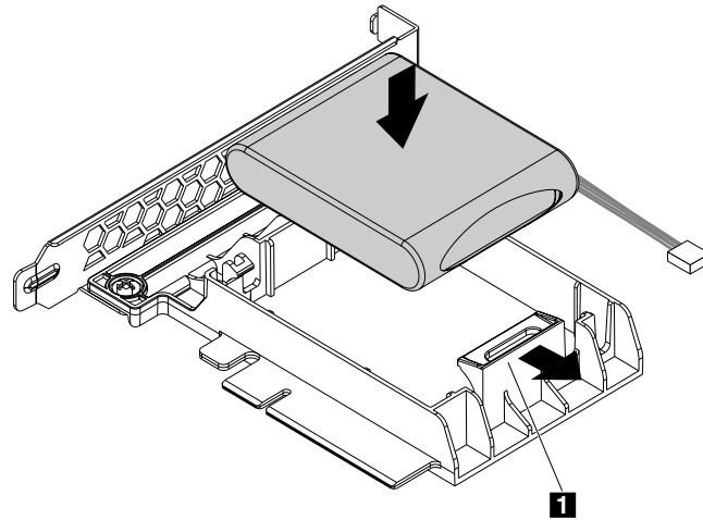
Figure 80. Installing the super capacitor module into the bracket
