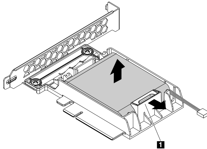
Figure 79. Removing the super capacitor module from the bracket
