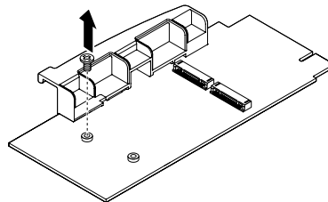
Figure 46. Removing the screw that is aligned with the M.2 slot
