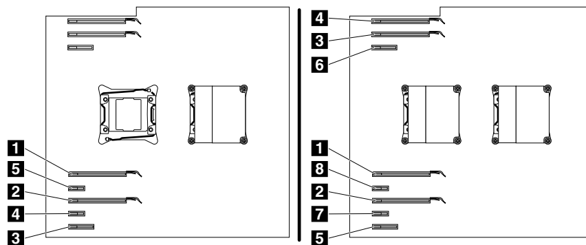
Figure 72. The order of installing PCI cards
