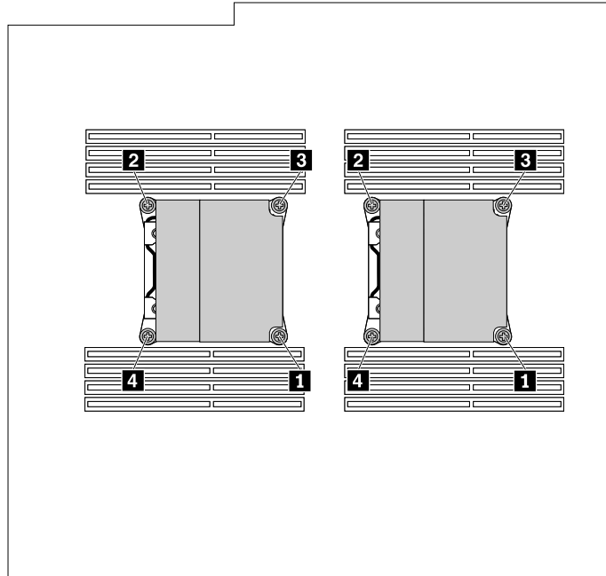
Figure 86. Removing the heat sink and fan assembly
