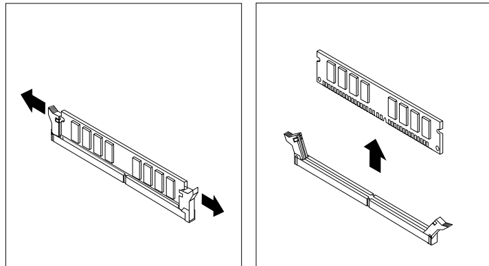
Figure 84. Removing the memory module
