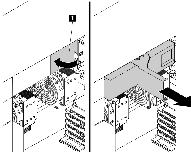
Figure 53. Removing the power supply assembly
