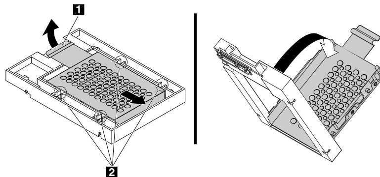
Figure 41. Removing the adapter from the converter
