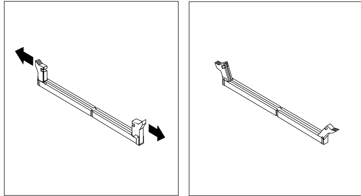
Figure 83. Opening retaining clips
