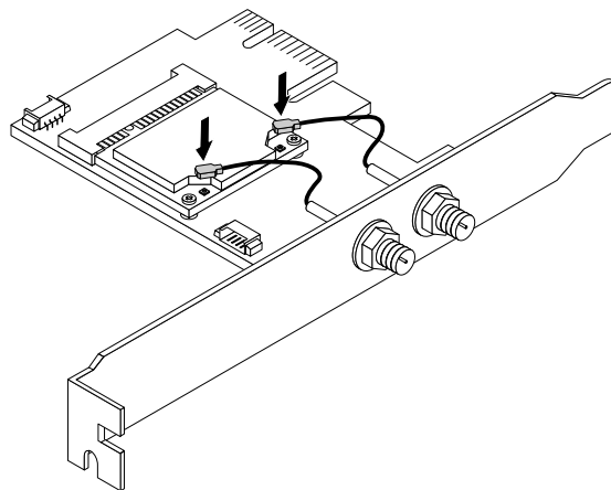
Figure 98. Connecting the Wi-Fi antenna cables
