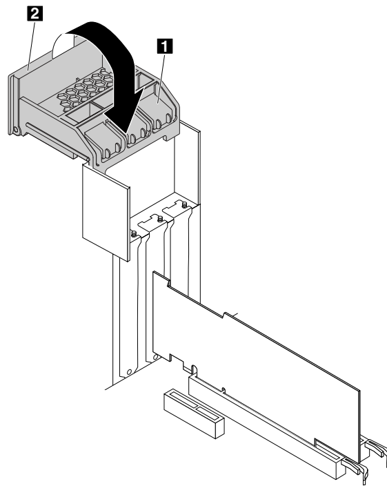
Figure 69. Closing the PCI card latch
