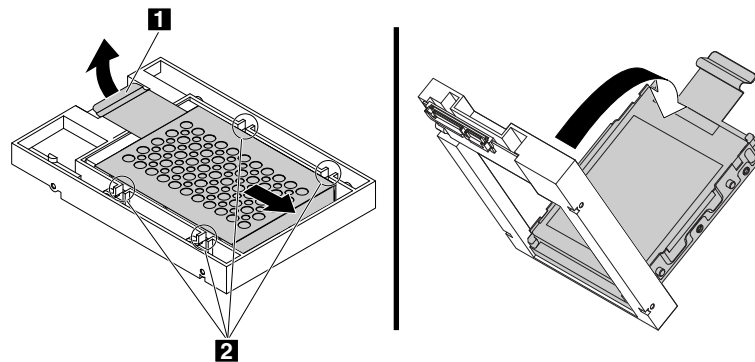
Figure 42. Removing the adapter from the converter
