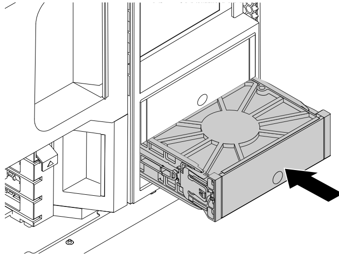
Figure 38. Installing the hard-disk-drive bracket
