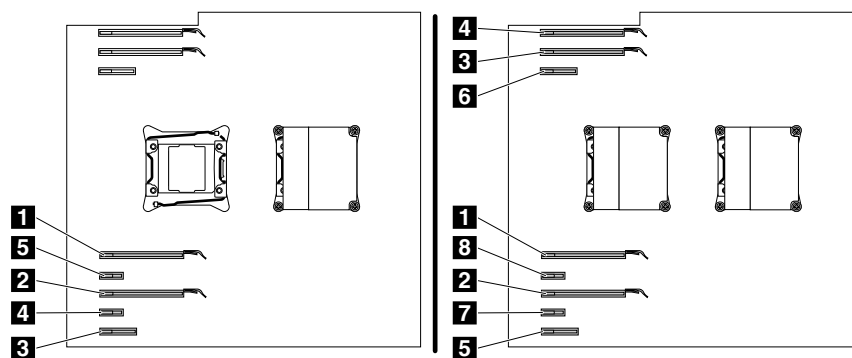
Figure 61. The order of installing PCI cards
