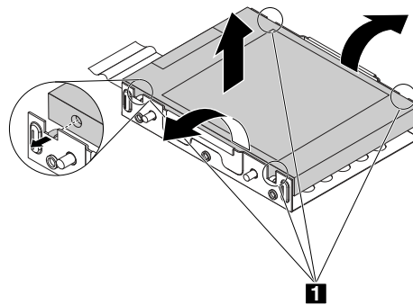
Figure 43. Removing the storage drive from the adapter
