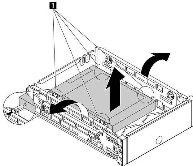
Figure 39. Removing the storage drive from the bracket
