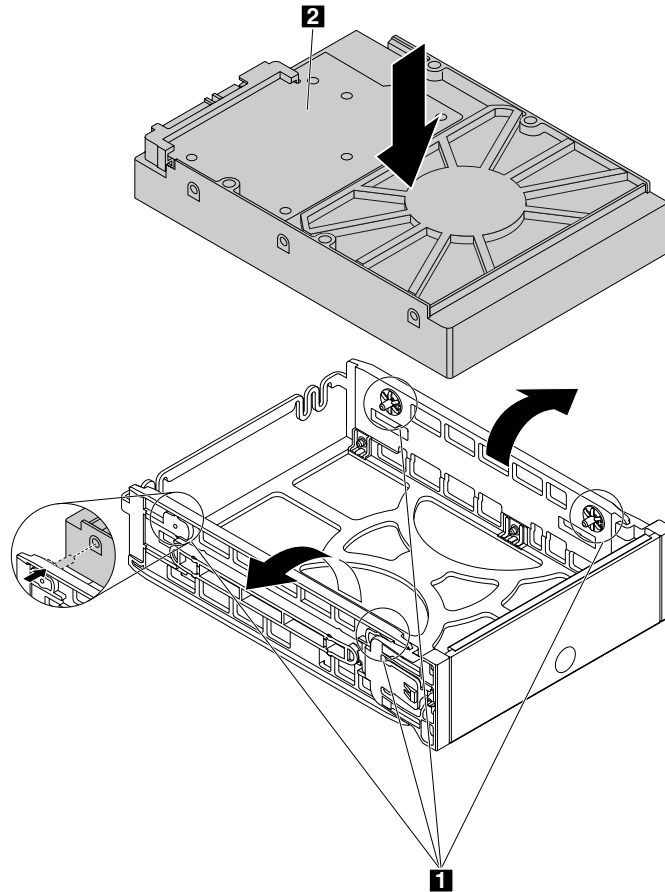
Figure 37. Installing the storage drive into the bracket
