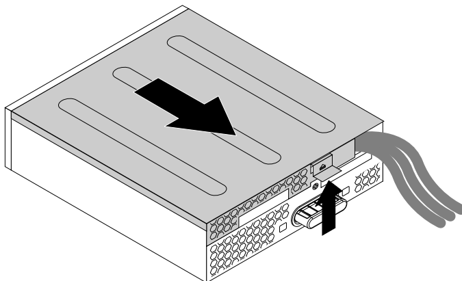
Figure 18. Removing the flex module cover
