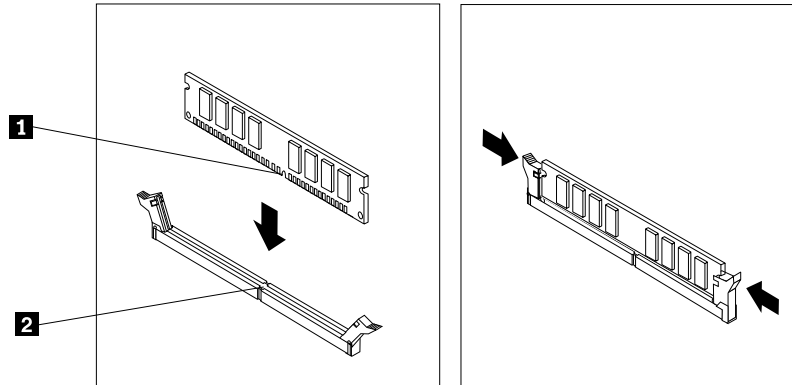
Figure 85. Installing the memory module
