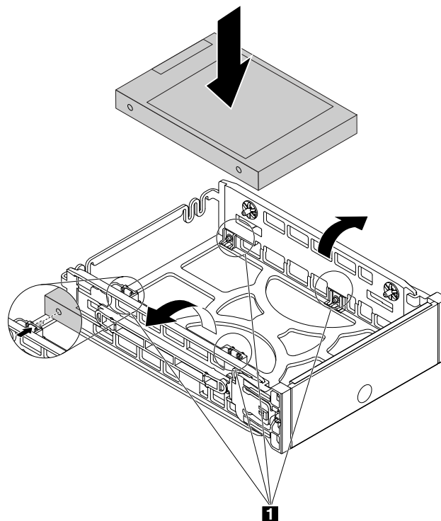
Figure 40. Installing the storage drive into the bracket
