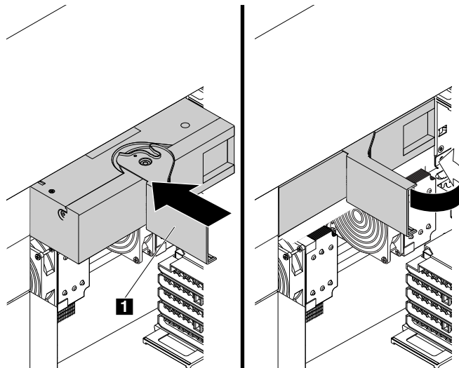
Figure 54. Installing the power supply assembly
