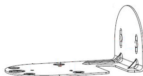
Camera Bracket
