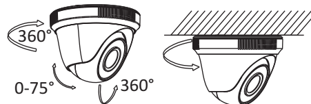
Figure 2-8 Lens Adjustment
