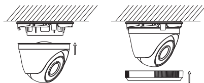
Figure 2-7 Secure the Components
