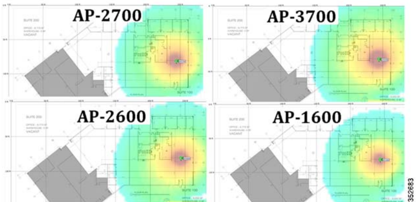
Figure 18 Heat Maps and coverage areas are fairly uniform between different APs
