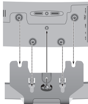
TV base, with TV-Mount attached
