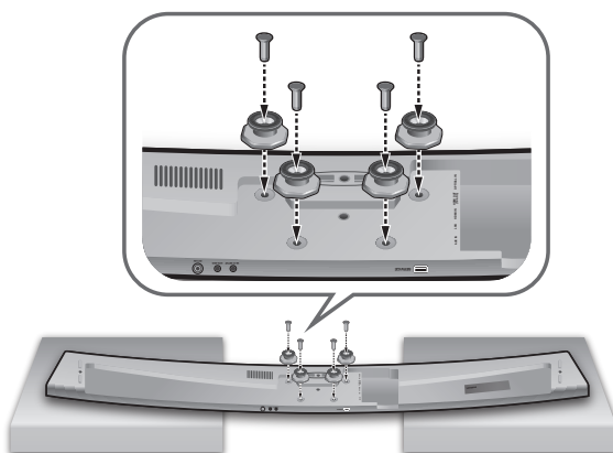
Holder-Support
