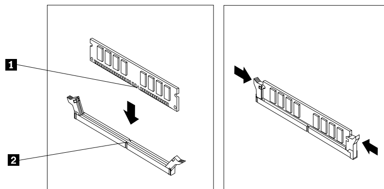
Figure 30. Installing a memory module
