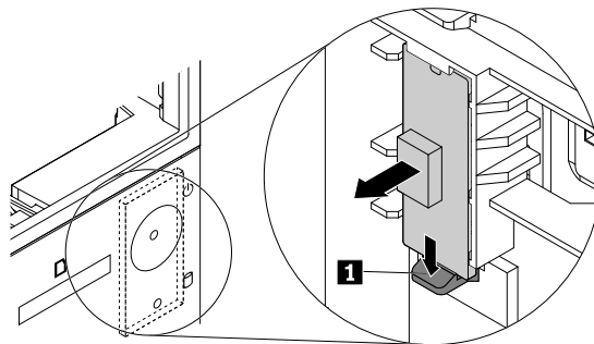
Figure 21. Removing the power button board from the front bezel
