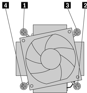
Figure 28. Removing the heat sink and fan assembly
