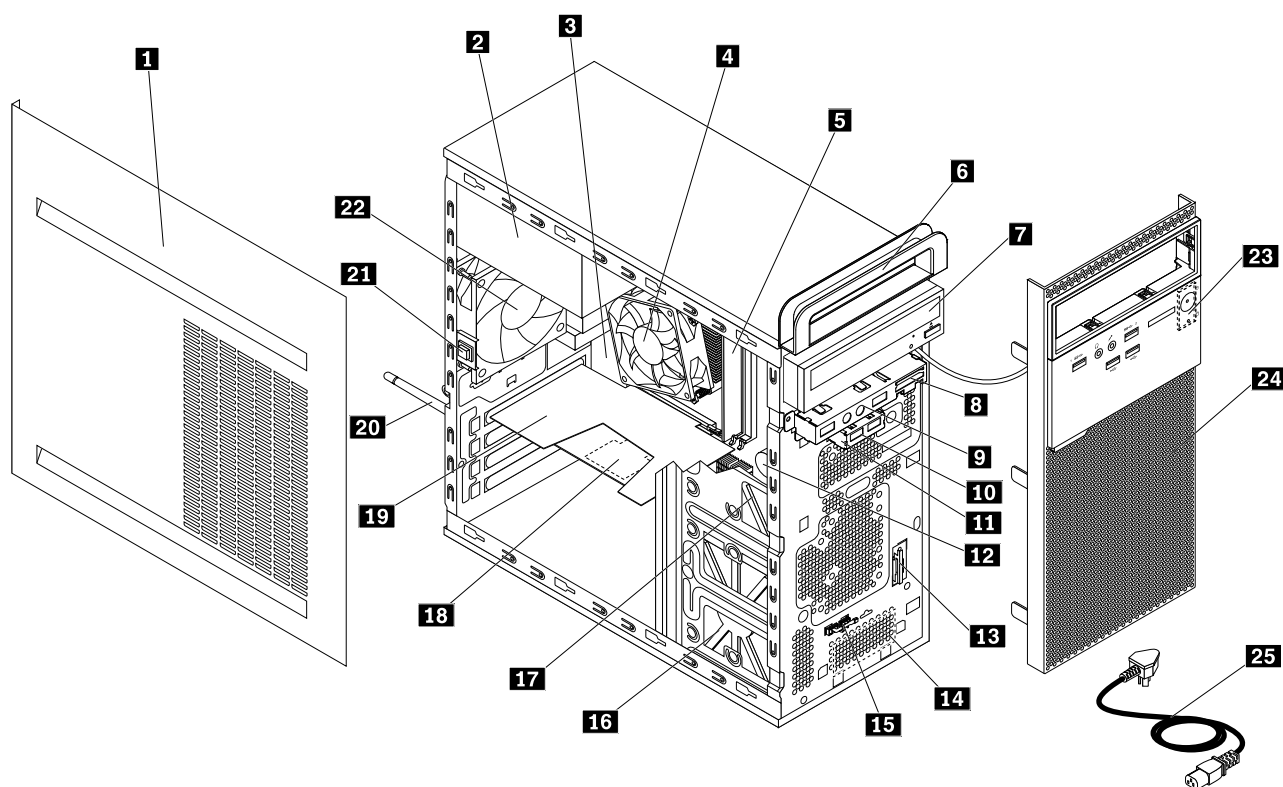
Figure 3. Computer components
