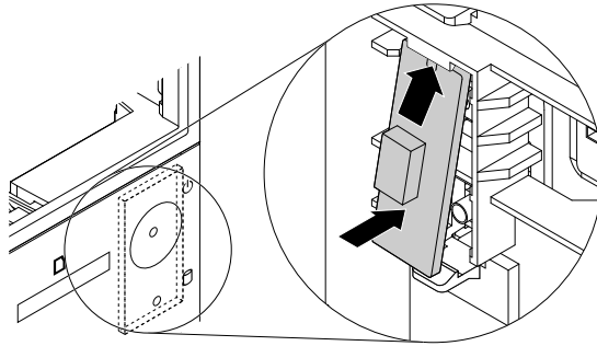
Figure 22. Installing the power button board to the front bezel
