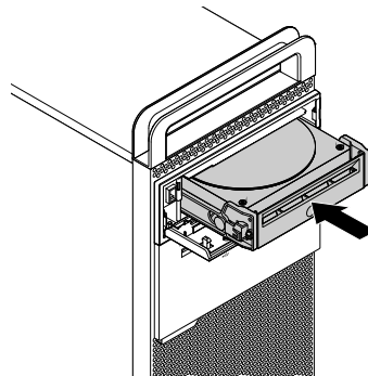
Figure 17. Installing the 3.5-inch storage drive bracket into the front-access storage enclosure
