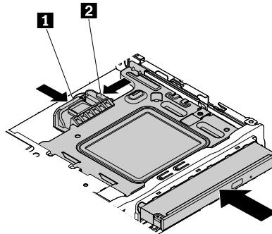
Figure 14. Removing the optical drive with the bracket
