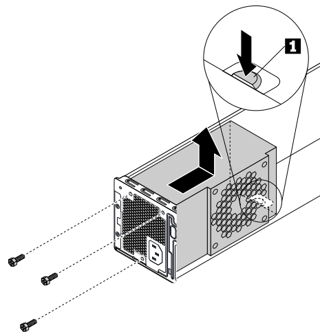
Figure 40. Removing the power supply assembly
