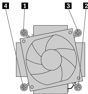
Figure 34. Removing the heat sink and fan assembly
