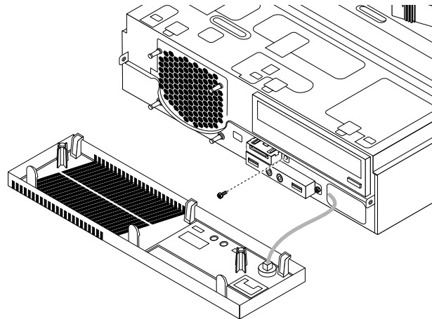
Figure 42. Installing the slim card reader bracket
