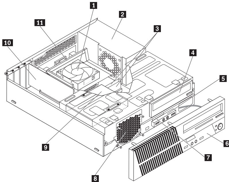
Figure 3. Component locations
