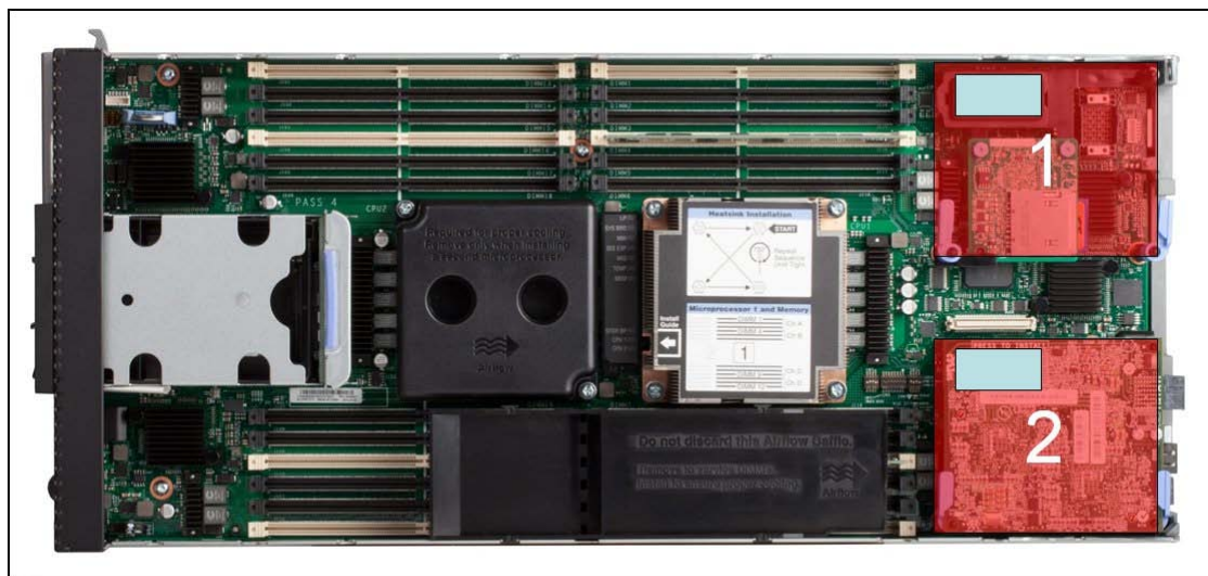
Figure 5. Location of the I/O adapter slots in the Flex System x240 M5 Compute Node
