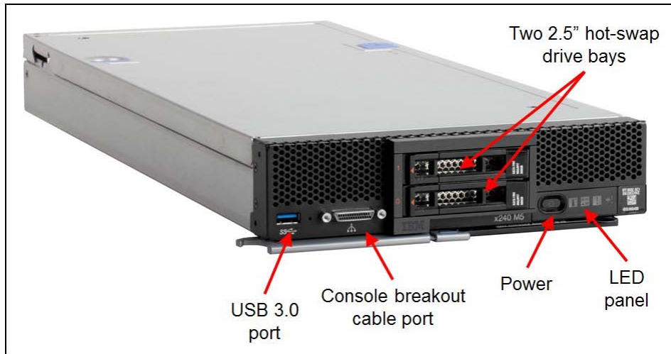
Figure 2. Front view of the Flex System x240 M5 Compute Node
