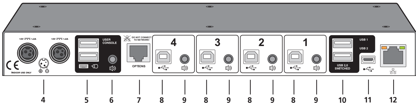
Figure 2-3. Rear panel.
