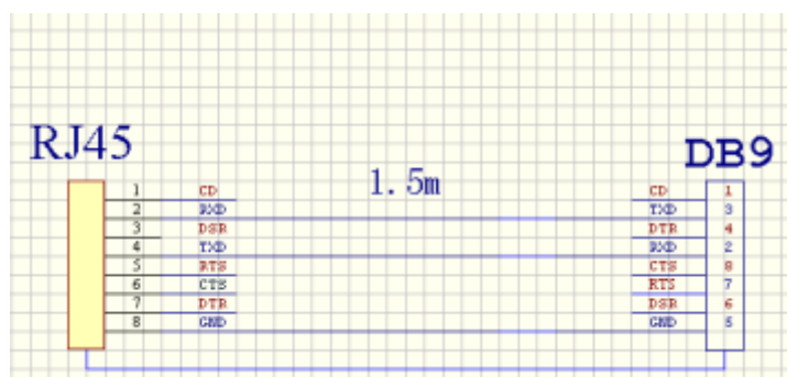
Figure 0-5 Cable connection at the console port
