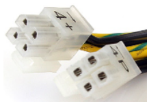
1 x 4+4 -pin ATX 12V (8-pin EPS12V)
