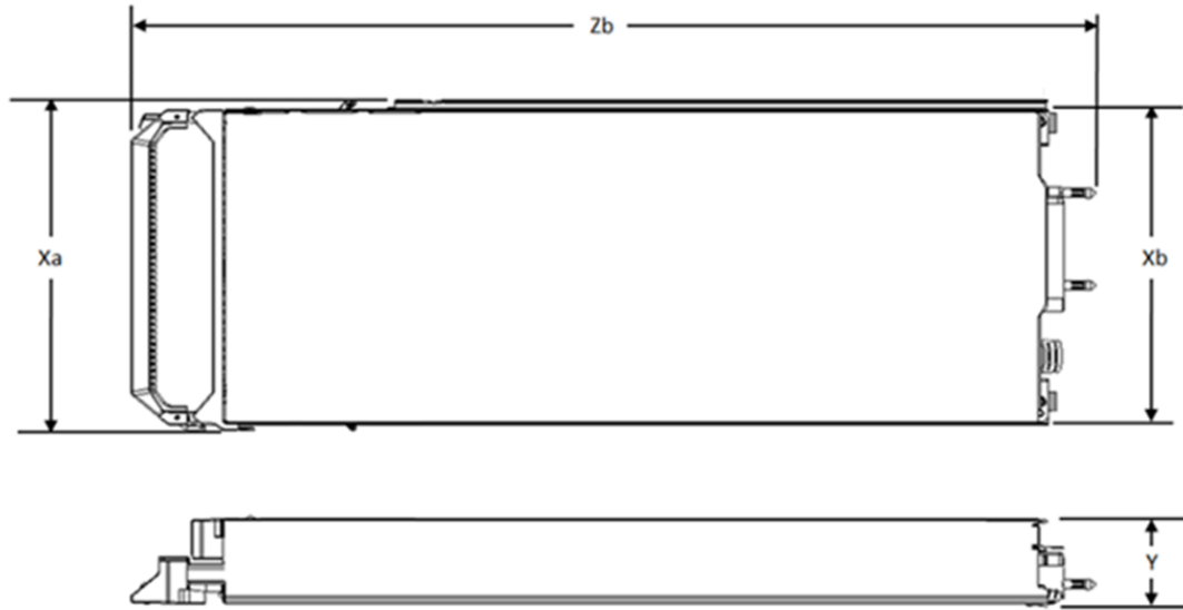
Figure 7. Module dimensions
