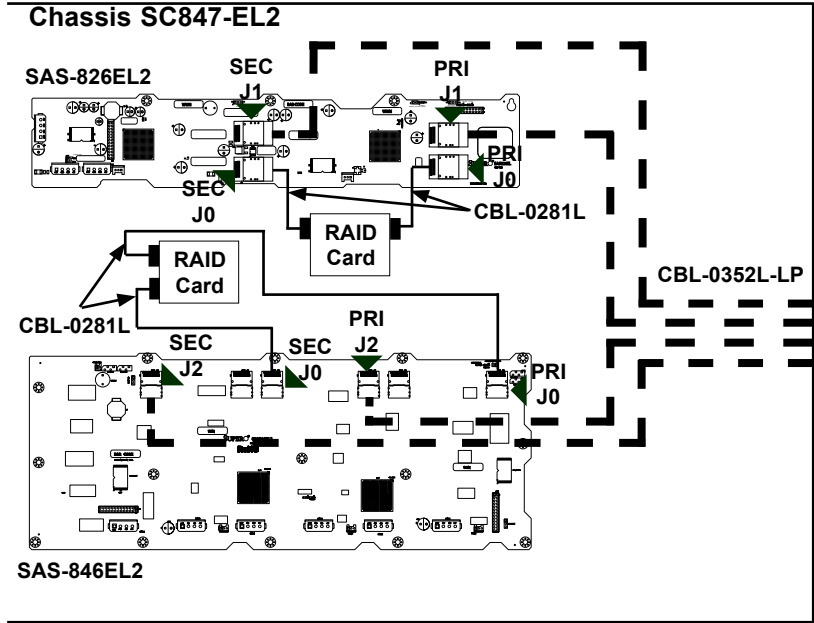
Figure 5-6: Serial Connectivity for Redundancy/Performance w/Multi-PCI Buses
