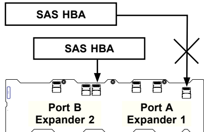
Figure F-9: Dual HBA Failover
