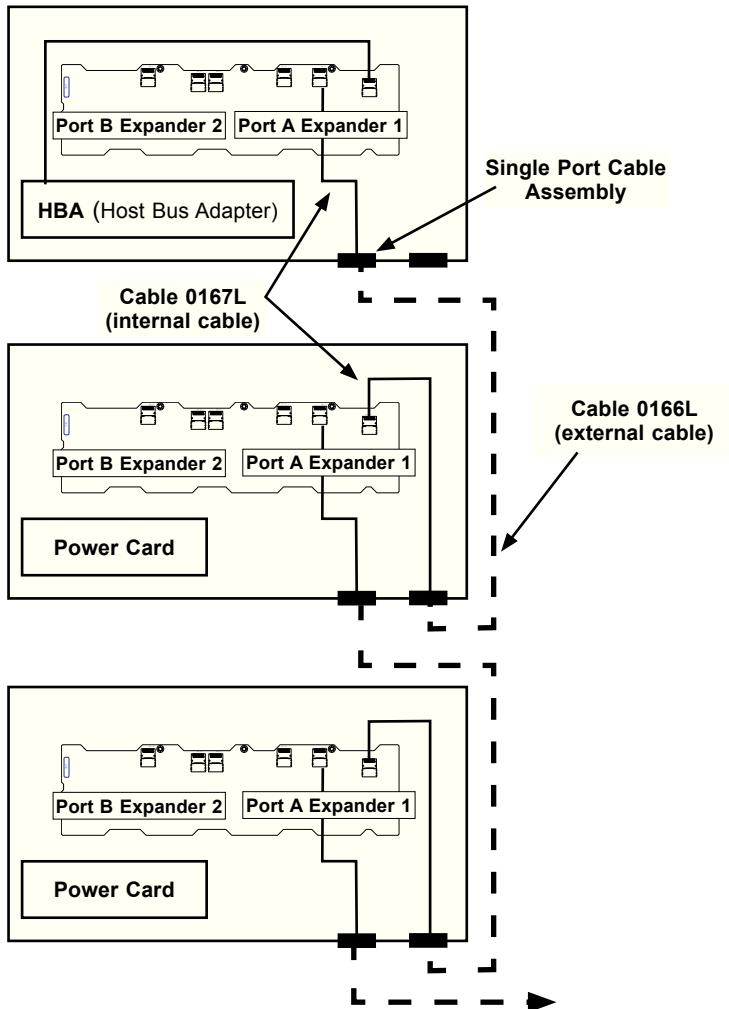
Figure F-22: Simple Cascaded Configuration
