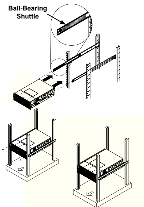
Figure 6-6: Installing into a Rack
