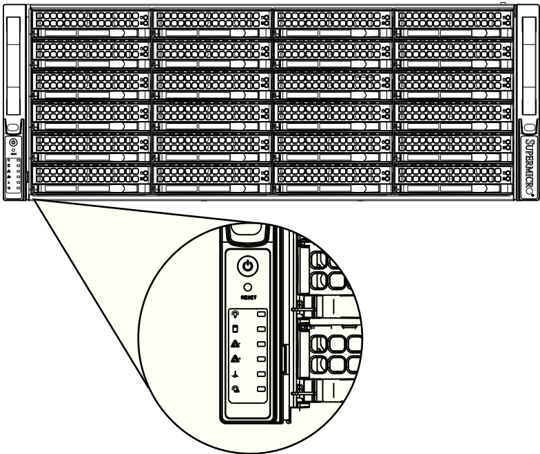
Figure 3-1: Control Panel
