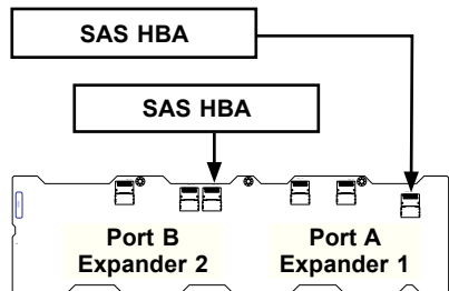
Figure F-8: Dual HBA
