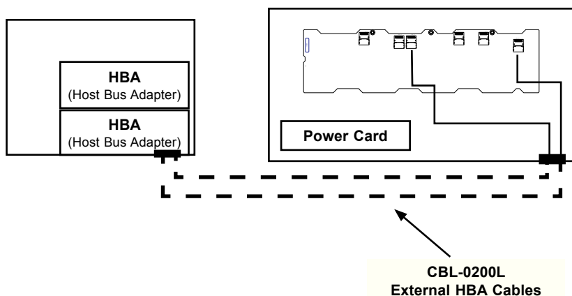
Figure F-14: Dual External Host Bus Adapter
