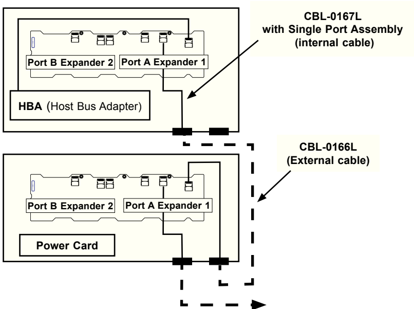
Figure F-16: Single HBA Configuration
