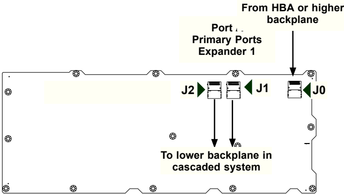
Figure F-5: SAS-846EL1 Single Port Configuration
