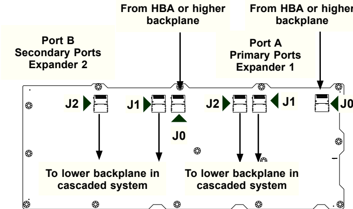
Figure F-4: SAS-846EL2 Dual Port Configuration
