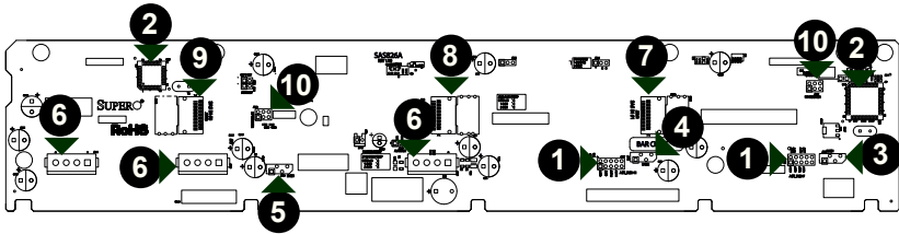
Figure C-1: Front Connectors
