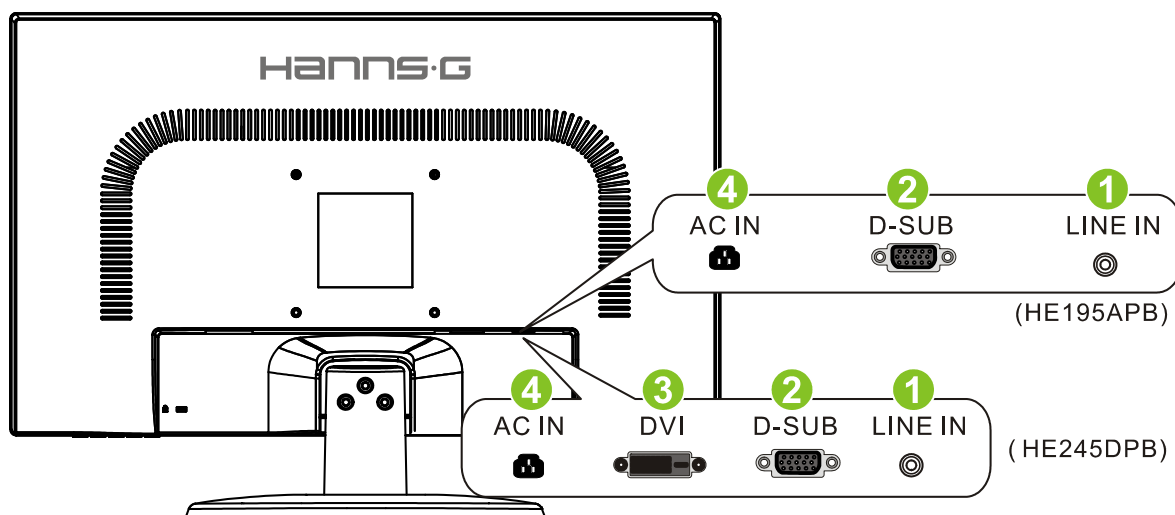
Figure.2. Connecting to a PC
