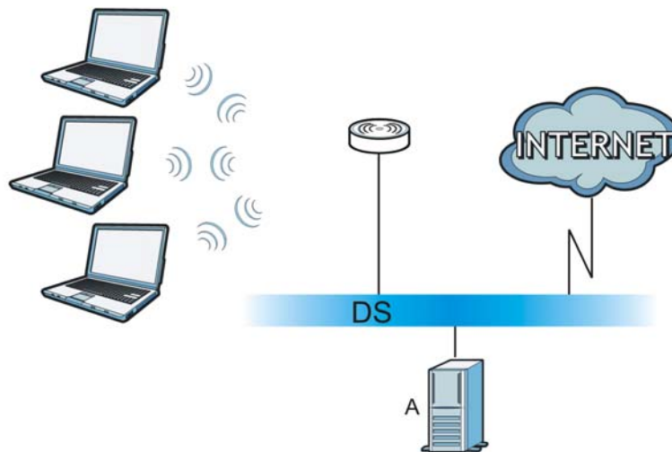
Figure 108 WPA(2) with RADIUS Application Example
