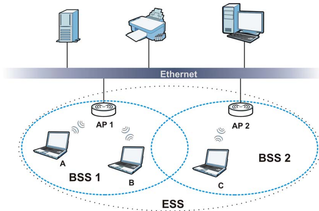
Figure 106 Infrastructure WLAN
