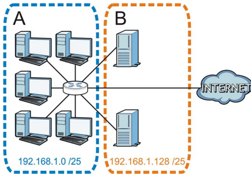
Figure 94 Subnetting Example: After Subnetting
