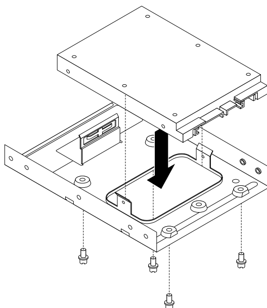
Figure 24. Installing the solid-state drive into the adapter
