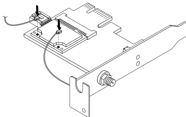
Figure 56. Connecting the WiFi antenna cables
