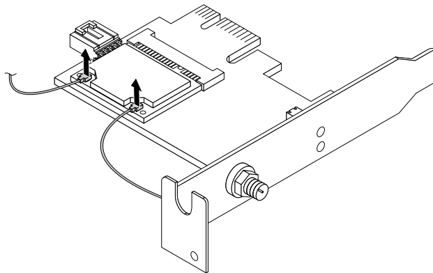
Figure 52. Removing the WiFi antenna cables
