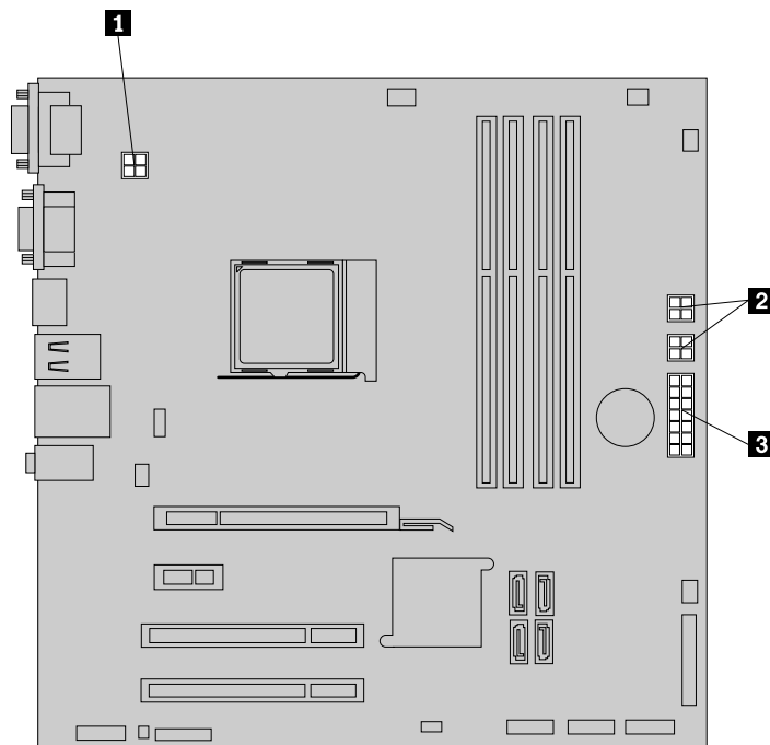
Figure 37. Power connectors on the system board
