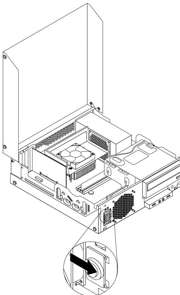
Figure 47. Installing the new internal speaker
