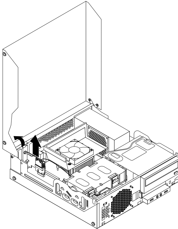
Figure 51. Removing the WiFi adapter card
