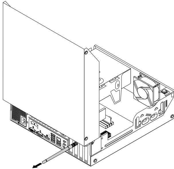
Figure 59. Removing the rear WiFi antenna
