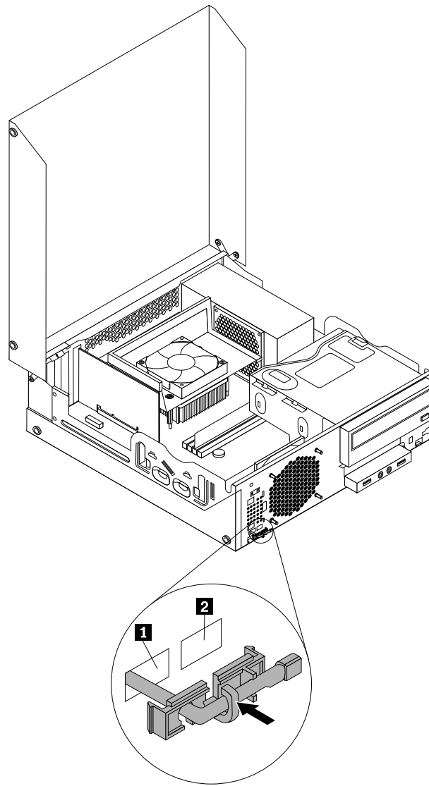
Figure 49. Installing the new thermal sensor
