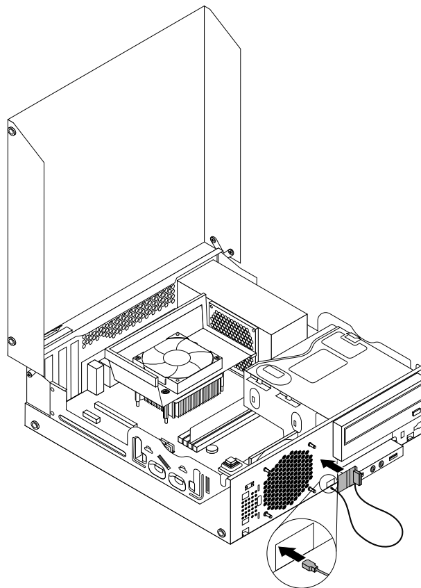
Figure 61. Installing the front WiFi antenna
