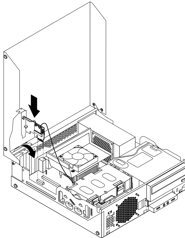
Figure 57. Installing the WiFi adapter card
