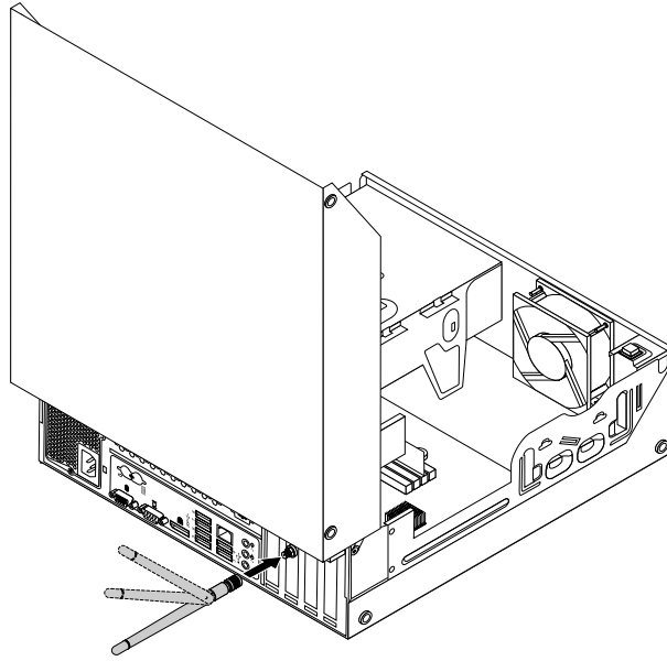
Figure 58. Installing the rear WiFi antenna
