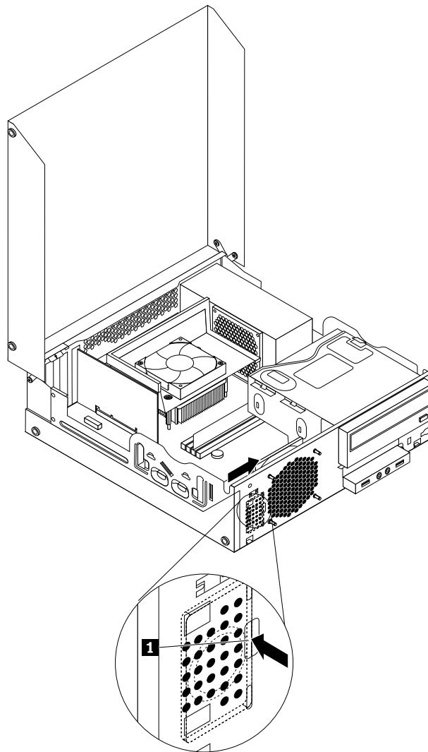
Figure 46. Removing the internal speaker
