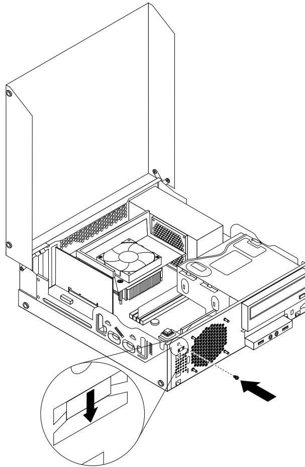
Figure 45. Installing the new cover presence switch
