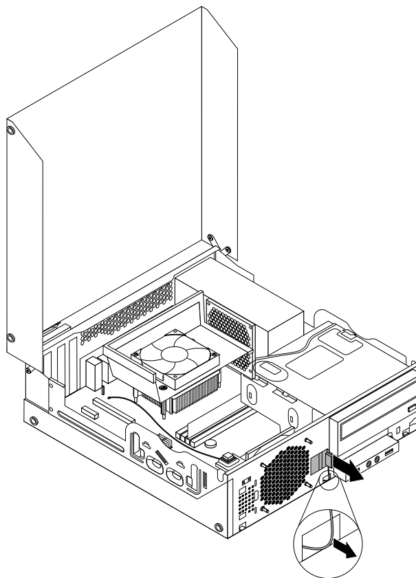
Figure 62. Removing the front WiFi antenna
