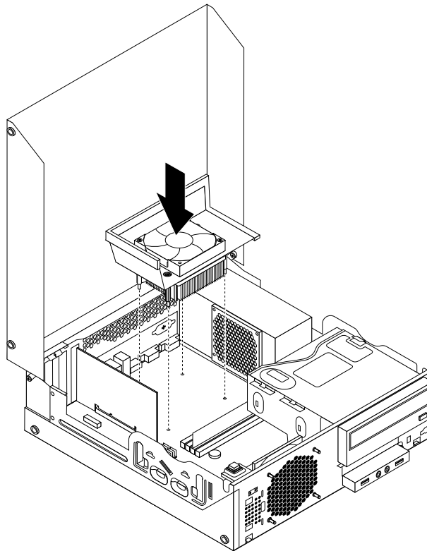
Figure 43. Reinstalling the heat sink and fan assembly with the fan duct
