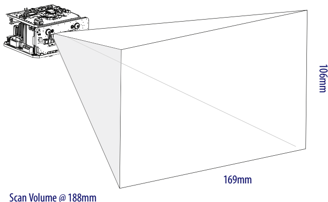
Figure 9. Scanning Volume
