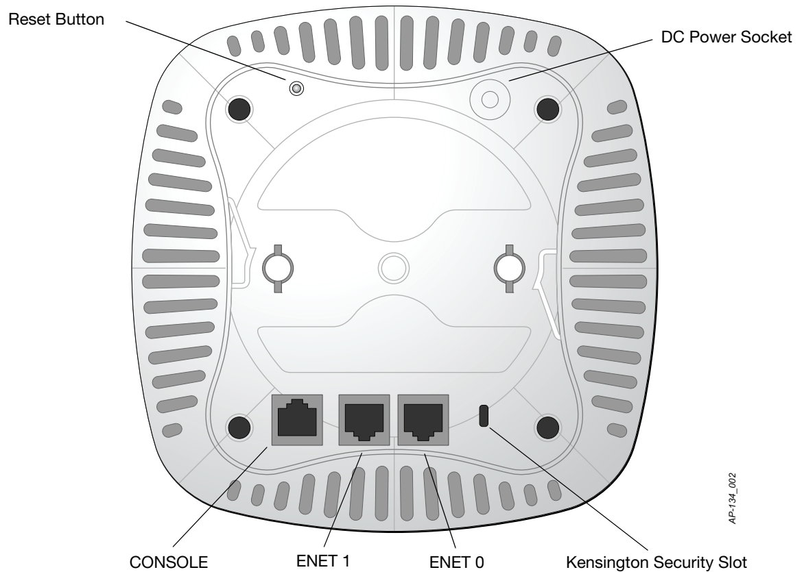
Figure 2 IAP-130 Series Rear
