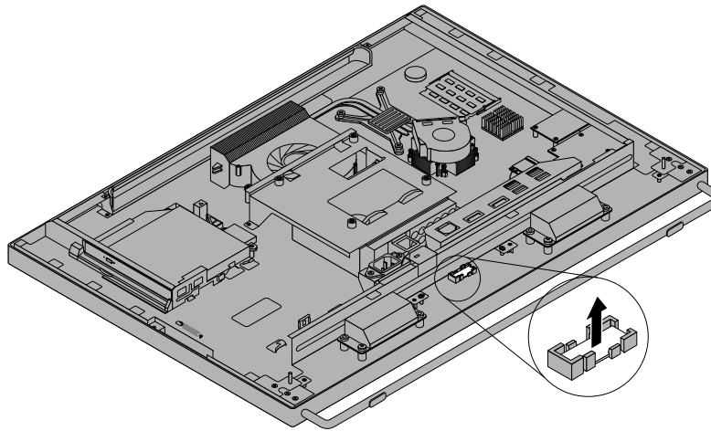
Figure 41. Removing the Bluetooth module
