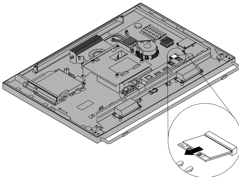
Figure 39. Removing the WI-FI card
