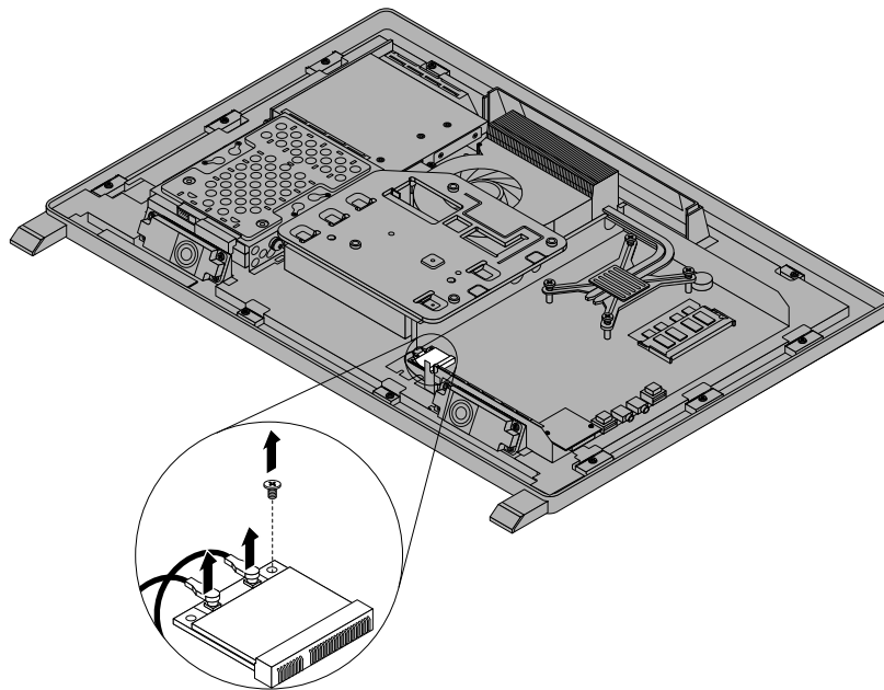
Figure 47. Removing the screw that secures the WI-FI card to the system board
