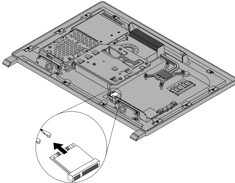
Figure 48. Removing the WI-FI card
