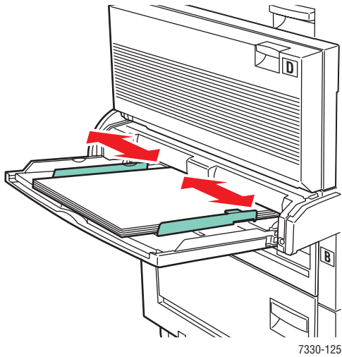
Tray 1 (MPT)
