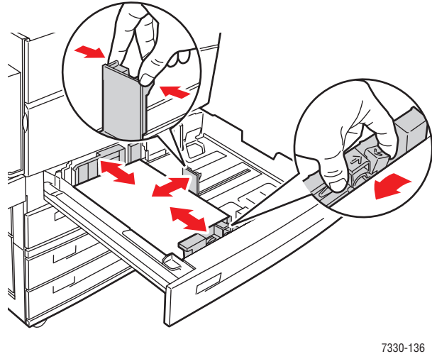
Trays 2-5
