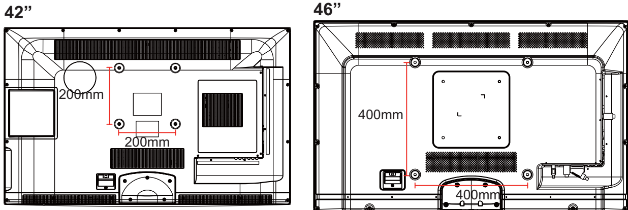
Dimensions for Mounting Hole Pattern
