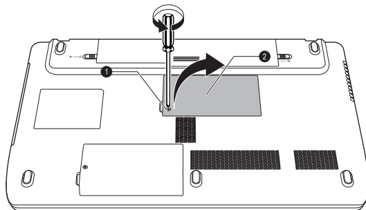
Figure 3-11 Removing the memory module cover (L770/L775/L770D/L775D)
