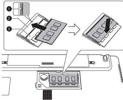
Figure 3-12 Seating the memory module (L770/L775/L770D/L775D)
