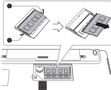
Figure 3-14 Removing the memory module (L770/L775/L770D/L775D)
