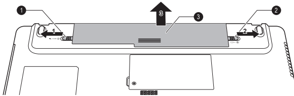
Figure 5-1 Releasing the battery pack (L770/L775/L770D/L775D)
