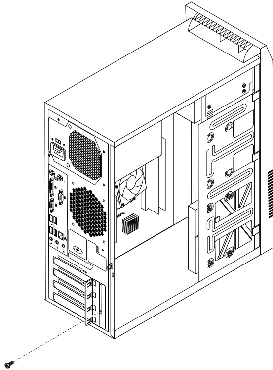
Figure 12. Removing the screw that secures the PCI card latch
