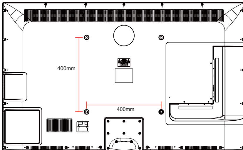
Dimensions for Mounting Hole Pattern
