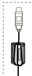
Ferrite Core for Side-HDMI (HDMI4) (LN46A650A1F: 3301-001305)
