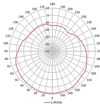
2.45GHz Vertical
