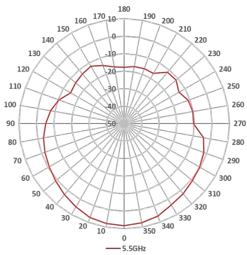
5.5GHz Vertical
