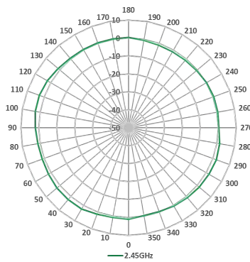
2.45GHz Horizontal
